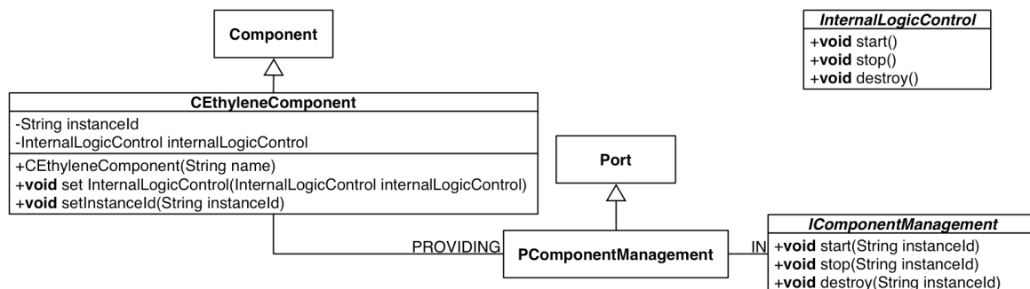
Figure VI-11 CEthyleneComponent et InternalLogicControl .
