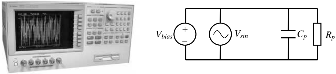
Figure 3-14: Capacitance measurement set-up and its equivalent circuit.
