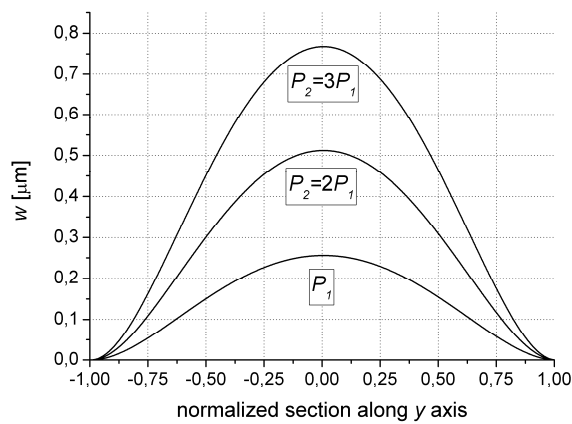
Figure 1-17: Square membrane deflection under the various pressures.
