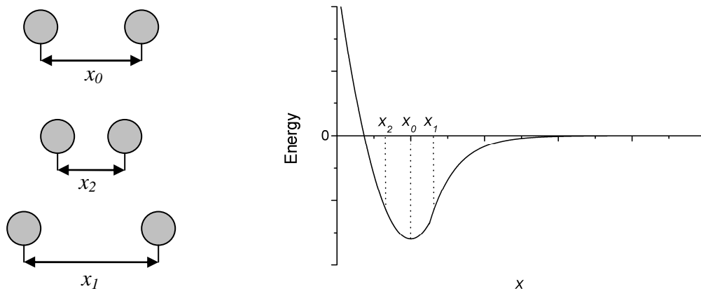
Figure A-1: Energy between two neighbouring atoms versus the distance between them.
