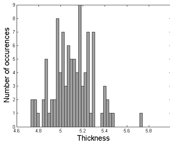
Figure 2-11: Histogram of thickness ( \mu\text{m} ) distribution on SOI wafers.
