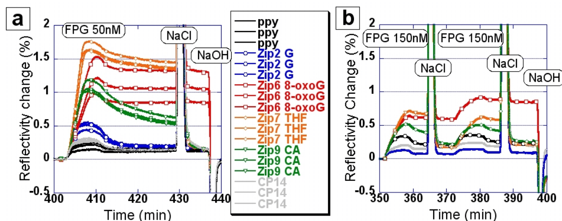
Figure 6.8: a) Covalent trapping of FPG at 50nM on its substrate 8-oxoG in 100mM NaBH 4 buffer. While FPG is regenerated by NaCl injection on all other DNA strands, it stays coupled to 8-oxoG. b) Same experiment with another FPG sample that shows much less activity. Two consecutive injections lead to accumulation of FPG on the 8-oxoG spots (signal averaged for 5 spots).
