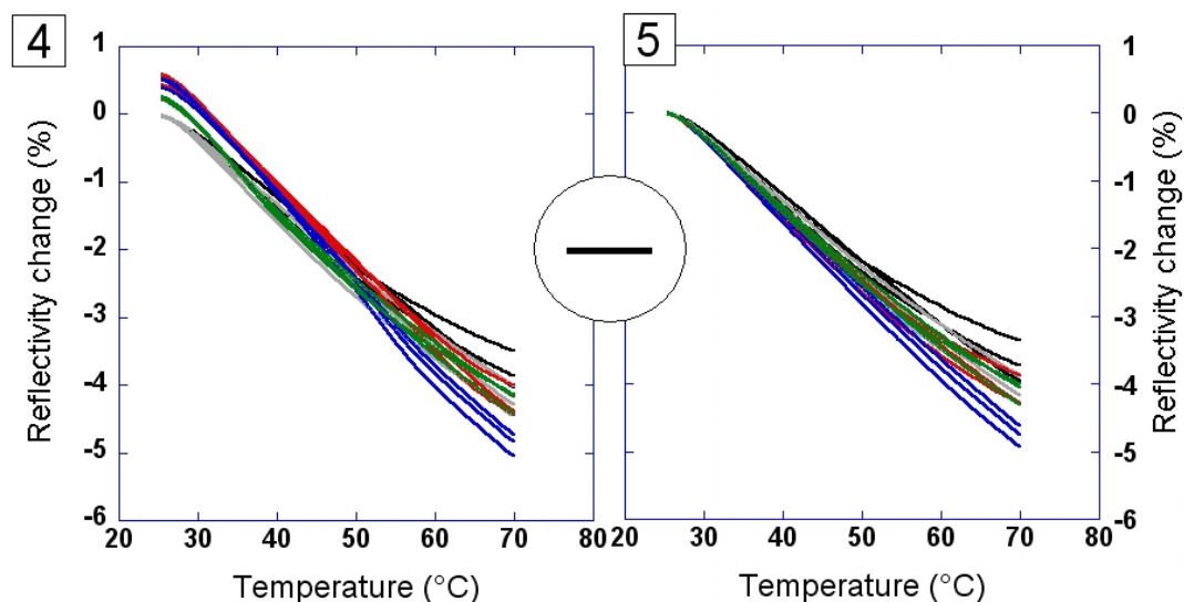
Figure 3: Data analysis - Subtraction of reference scan: 4) Synchronized T-scan with DNA. 5) Synchronized T-scan without DNA.
