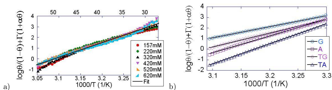
Figure 4.15: Superposition of the melting curves with one adjustable parameter c_p . a) Collapse of curves for Gc20 on TG with c_p = 13 mM. b) Fit of collapsed melting curves for all analyzed probes hybridized to Gc20.
