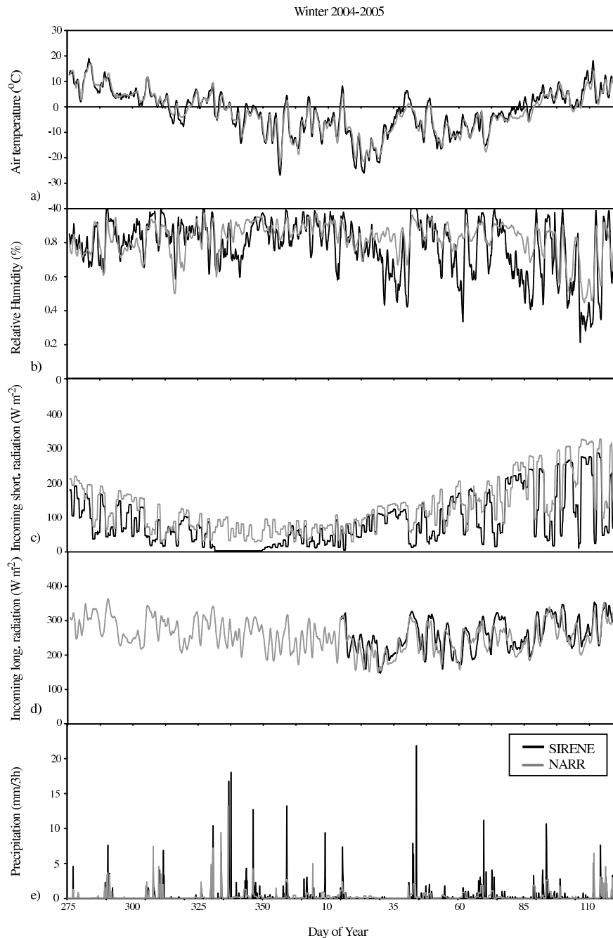
Figure 7.2: Temporal evolution of a) air temperature, b) relative humidity, c) incoming shortwave radiation, d) incoming longwave radiation and e) precipitation measured at the SIRENE station and from NARR data during the 2004-2005 winter season.
