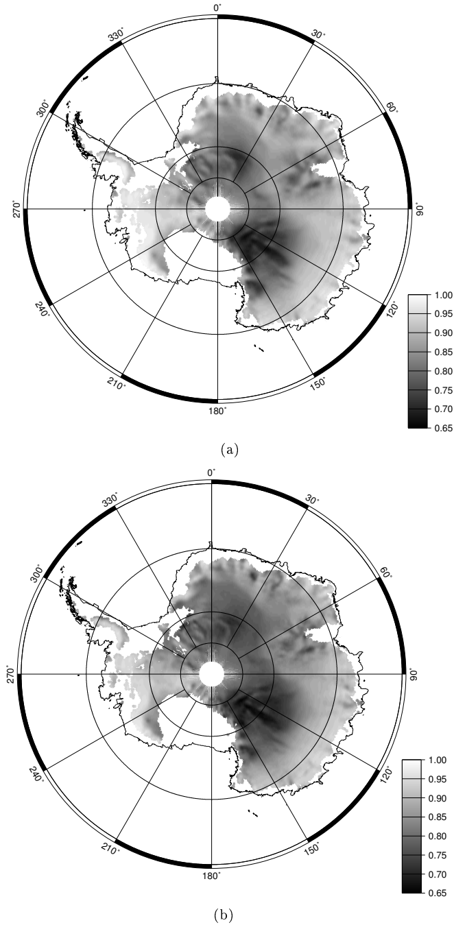
Figure 5.1: Maps of averaged emissivities at vertical polarization, 19.3 GHz (a) and 37 GHz (b) based on Equation (5.1). Regions where melt occurred are masked (in white). No data are available South of 87.8°.
