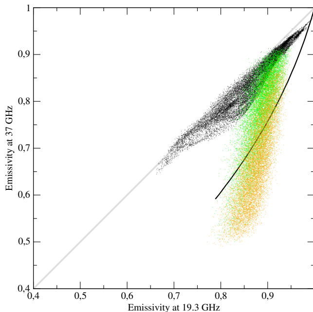
Figure 5.4: Modeled emissivities at vertical polarization for snowpacks with a fixed snow grain size (0.7 mm) and 15 random variations of snow density in the first 10 meters. Snowpacks were classified in two categories depending on the increase (orange color) or decrease (green color) of the density trend with depth. The plain curve represents the emissivity of homogeneous snowpacks (DMRT-ML calculation, grain size of 0.1 to 1 mm, see Figure 5.3). Black dots are the observed emissivities.
