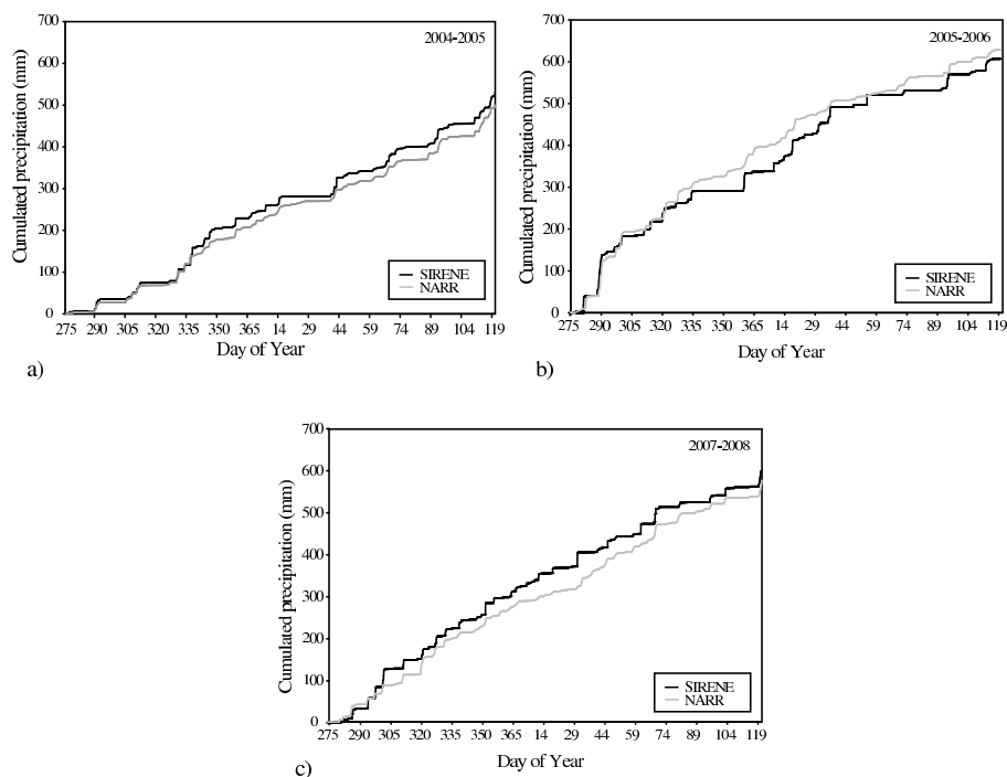
Figure 7.3: Temporal evolution of accumulated precipitation measured at the SIRENE station and from NARR during the a) 2004-2005, b) 2005-2006 and c) 2007-2008 winters.
