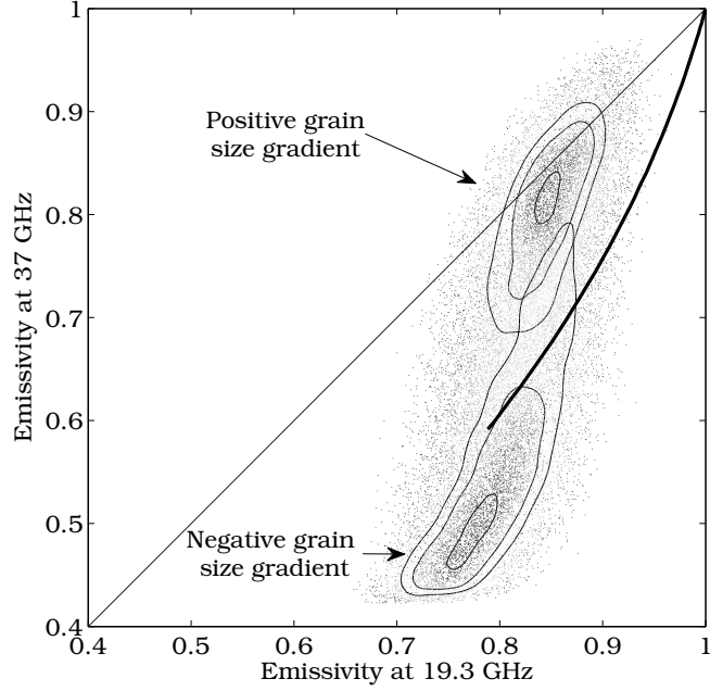
Figure 5.5: Modeled vertically-polarized emissivities for snowpacks with a fixed density and random variations of snow grain sizes. Snowpacks were classified in two categories depending on the increase or decrease of the grain size trend with depth, (i.e., positive and negative grain size gradient). Contour lines represent three various levels of density dots for the two types of snow grain size profiles. The plain curve represents the emissivity of homogeneous snowpacks (DMRT-ML calculation, density of 350 \text{ kg m}^{-3} , see Figure 5.3).
