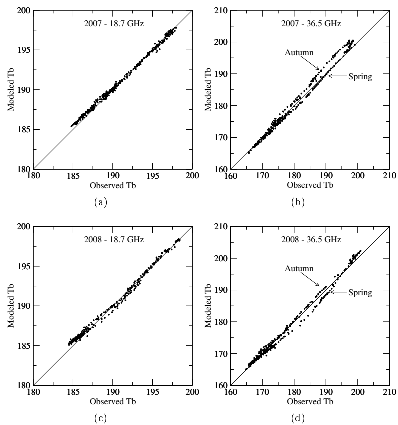
Figure 4.8: Modeled brightness temperature as a function of the observed ones, during the year 2007 (first row) and 2008 (second row), at 18.7 GHz (left panels) and 36.5 GHz (right panels).
