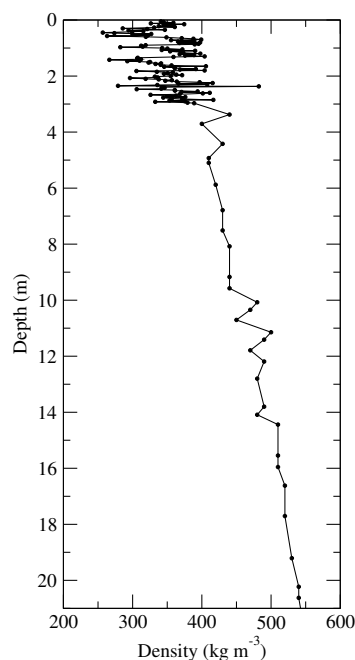
Figure 4.3: Snow density profile measured, at Dome C, used to drive the DMRT-ML model. Down to 3 m depth snow density was measured in a snow pit with a 2-3 cm vertical resolution. Below, measurements were done on a snow core.
