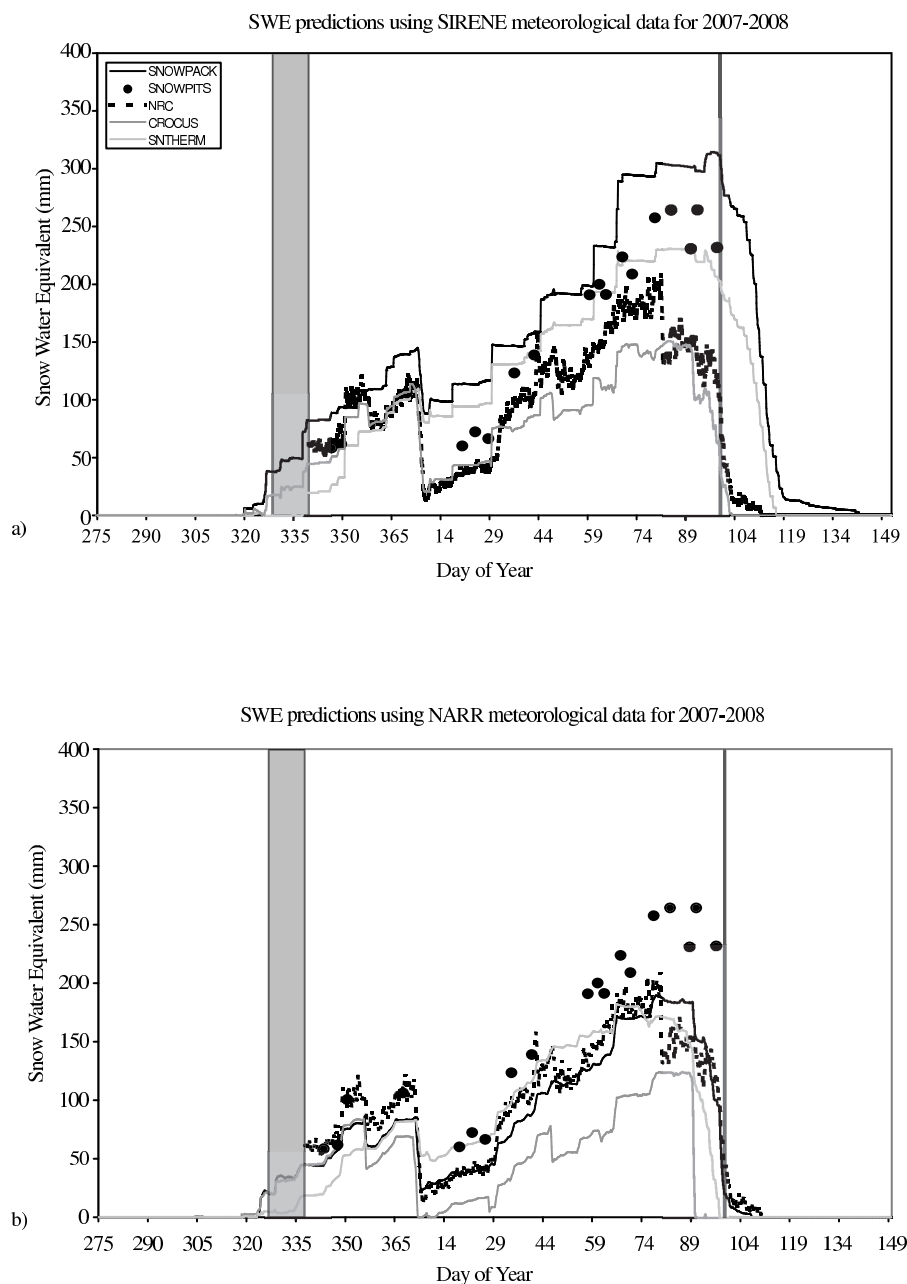
Figure 7.6: Snow water equivalent simulations from SNOWPACK, Crocus and SNTherm using a) SIRENE and b) NARR meteorological information for the 2007-2008 winter. Gray bars represent the duration between the first snow accumulation and melting observations from the Sherbrooke-A and Lennoxville Environment Canada weather stations.
