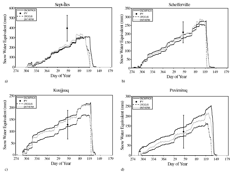
Figure 7.8: Comparison between predicted and measured SWE values in a) Sept-Îles, b) Schefferville, c) Kuujuaq and d) Puvirnituk using SNOWPACK during the IPY project.
