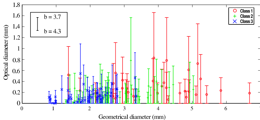
FIG. E8 – Comparison between the modeled retrieved optical diameters from NIR reflectance measurements versus measured geometrical diameters with respect to three different snow classes. The Y-bars correspond to the range of the shape factor ( b = 3.7 and 4.3 ) used in the retrieval.
