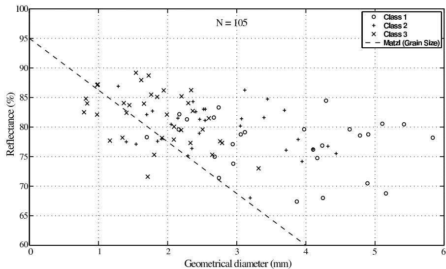
FIG. E7 – Relationship between measured NIR reflectance normalized to 840 nm versus measured snow grain geometrical diameter from the ‘traditional’ snow macro-photographs. The dotted line represents the same relation from Matzl, (2006).
