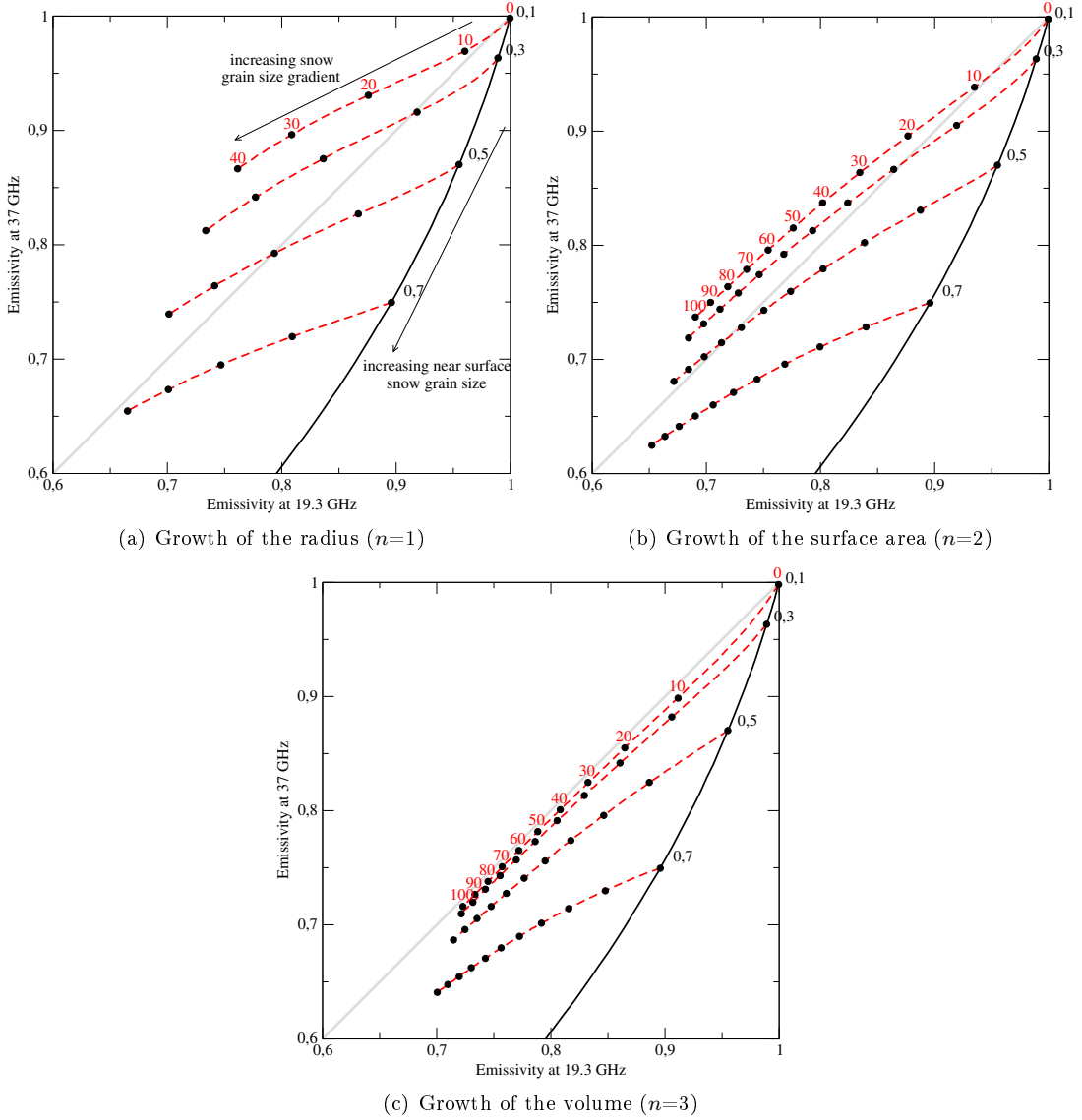
Figure 5.6: Modeled emissivities of homogeneous snowpacks (black plain curve) and of snowpack with linear increase of the snow grain radius 5.6(a), grain surface area 5.6(b) and grain volume 5.6(c). The dashed red curves represent an increase of the grain size gradient for a given near-surface snow grain size (see Equation (5.2)). Annotated values along the dashed curve is Q_n in \mu\text{m}^2 \text{m}^{-1} , and along the homogeneous curve is the near-surface grain size in mm.
