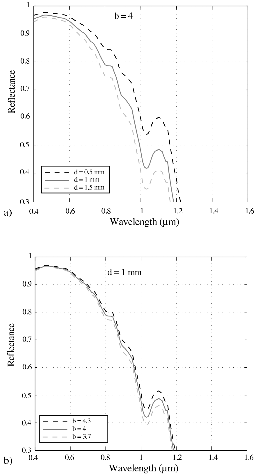
FIG. E1 – Spectral reflectance of snow a) for three different values of snow grain optical diameter, and for a constant shape factor (b) (Eq. E.1); b) for three different shape factors with constant optical diameter.
