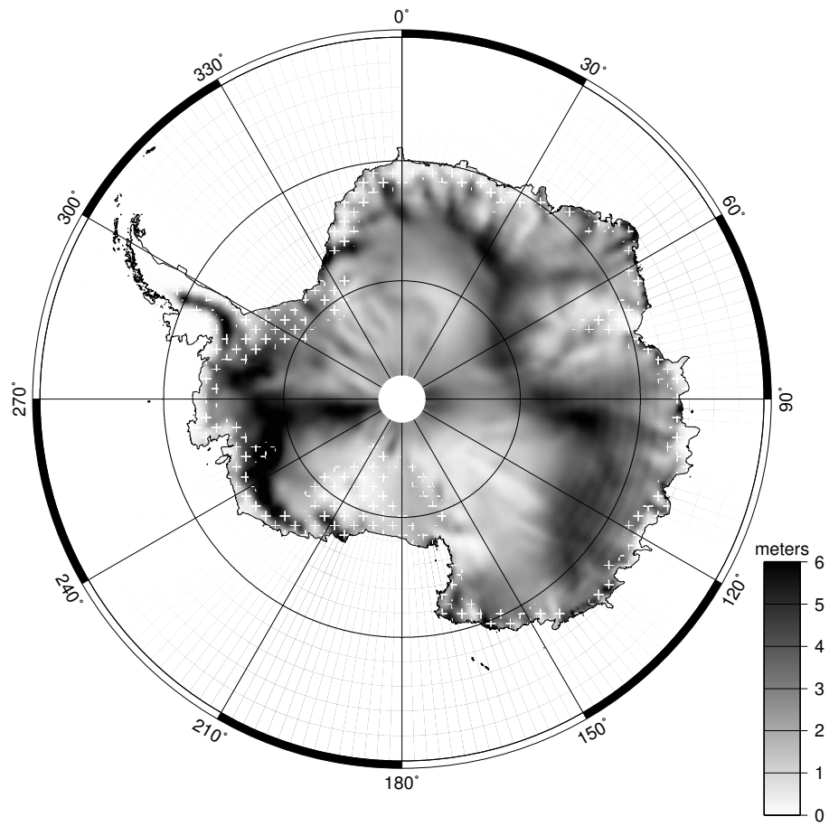
FIG. F1 – Apparent penetration depth at 19 GHz, V polarization. Penetration depth is relative to the arbitrarily chosen thermal diffusivity ( 5 \times 10^{-7} \text{ m}^2 \text{ s}^{-1} here). Melt zones are shown with white crosses.
