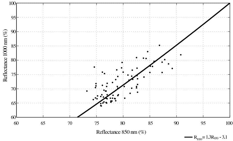
FIG. E4 – Measured offsets between the snow reflectance (averaged at 3-cm vertical resolution) acquired with 850nm and 1000nm filters, successively in the same snowpits. The line corresponds to the theoretical model using the Kokhanovsky and Zege (2004) reflectance equation E.2.
