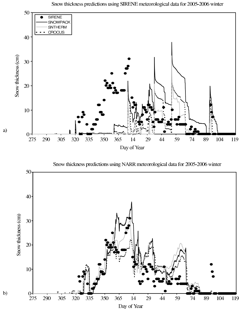
Figure 7.5: Snow thickness simulations from SNOWPACK, Crocus and SNTherm using a) SIRENE and b) NARR meteorological information for the 2005-2006 winter.
