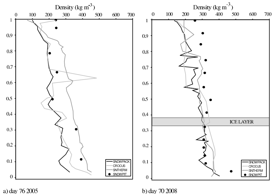
Figure 7.7: Modeled and measured vertical profile comparison of density for a) day 76 2005 and b) day 70 2008.
