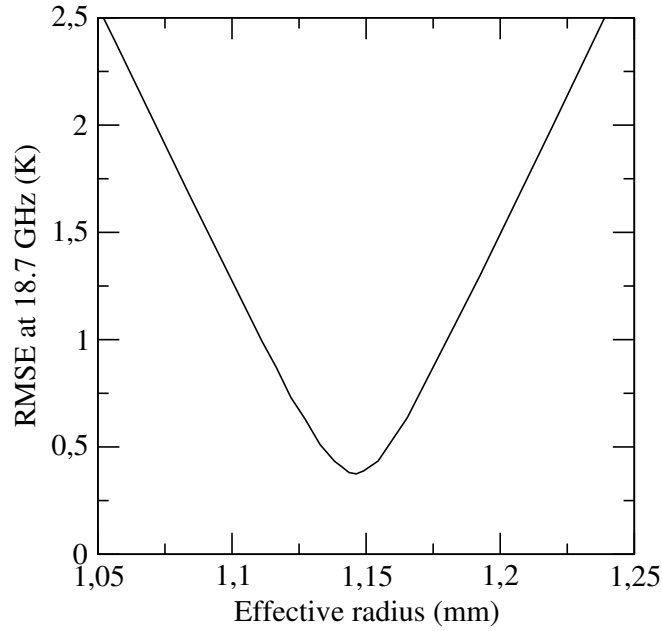
Figure 4.6: RMSE at 18.7 GHz as a function of r^z > 3m .
