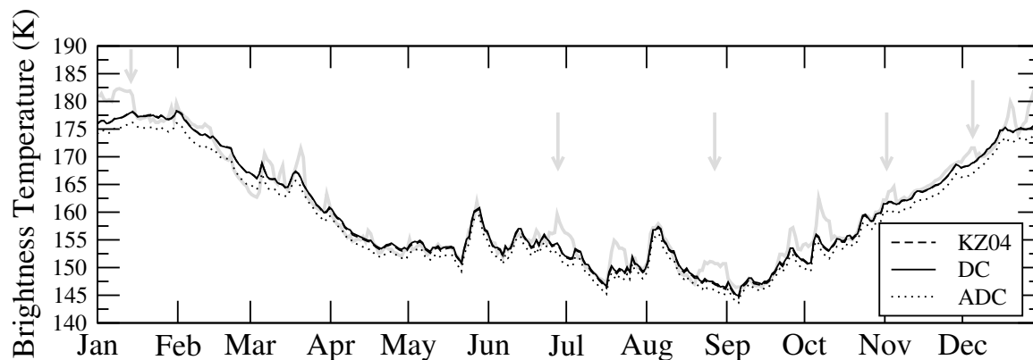
Figure 4.9: Observed (grey curves) and modeled time series of horizontally-polarized brightness temperature at Dome C between in 2007 at 36.5 GHz using parameters in Table 4.3 and all relationships (DC, ADC and KZ04). The arrows indicate locations where a change in surface properties of the snowpack occurred.
