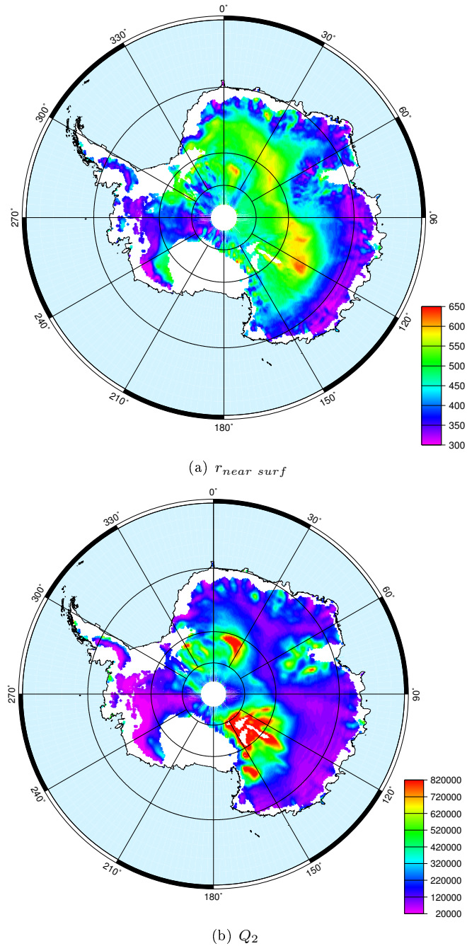
Figure 5.7: Maps of the near-surface grain size (in \mu\text{m} ) (a) and of the grain size vertical gradient Q_2 (in \mu\text{m}^2\text{m}^{-1} ) (b) in the Antarctic dry-zones derived from the 19.3 GHz and 37 GHz vertically-polarized emissivities.
