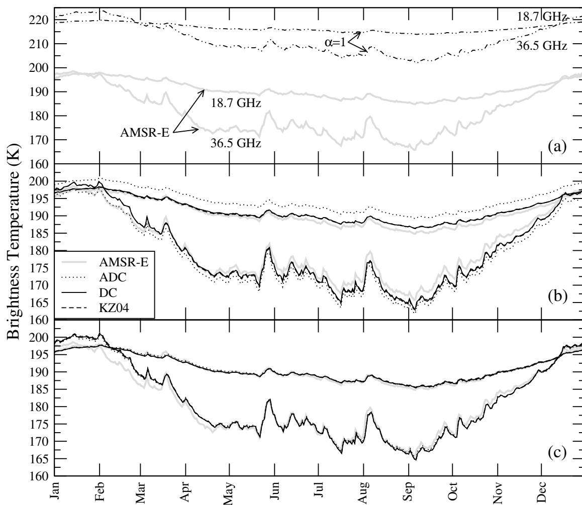
Figure 4.5: Observed (grey curves) and modeled time series of vertically-polarized brightness temperature at Dome C in 2007 at 18.7 GHz and 36.5 GHz using : (a) DC and \alpha = 1 , (b) the three relationships (DC, ADC and KZ04) with a calibrated \alpha (see Table 4.2) and (c) the three relationships with a calibrated \alpha and a calibrated snow grain size below 3 m depth (see Table 4.3).
