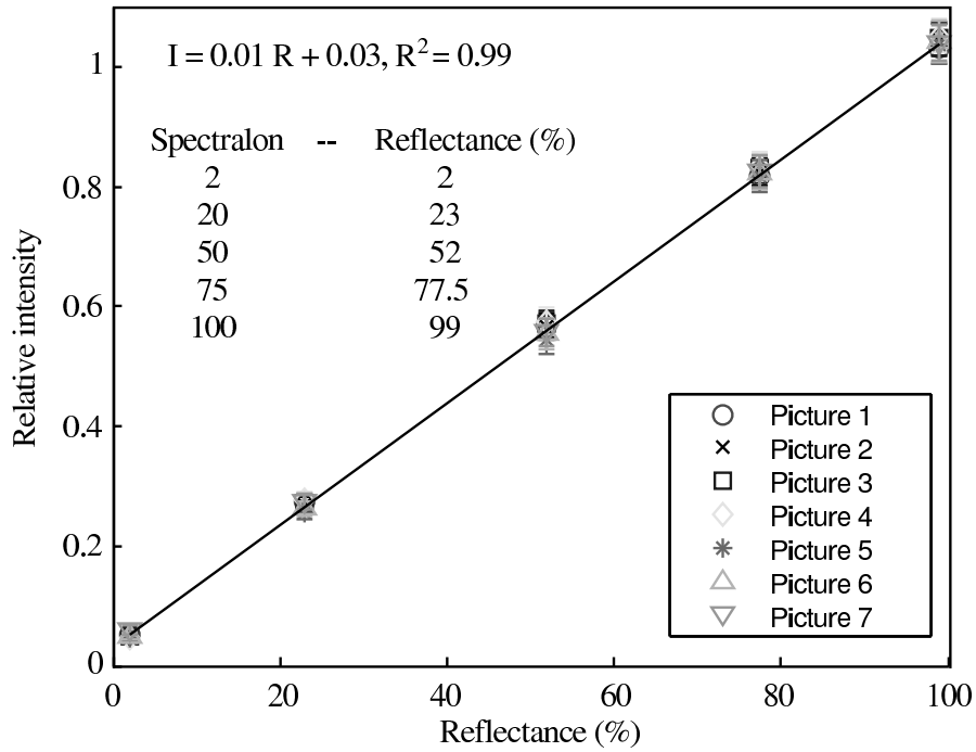
FIG. E2 – Correlation between relative intensity of NIR photographs with different standard reflectance targets at 2, 20, 50, 75 and 100% nominal reflectance.
