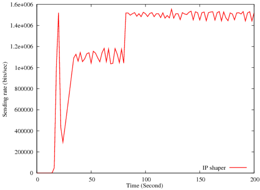
Fig 4.11-b TFRC rate IP shaper
