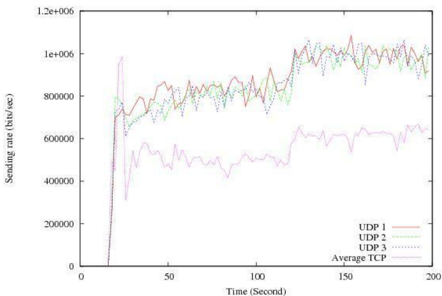
Fig 4.12 Default rate
