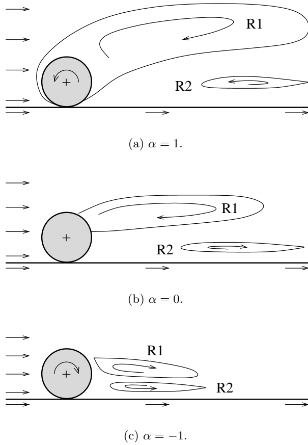
FIGURE 4.2: Schematic representation of the upper and lower recirculation zones at various rotation rates.
