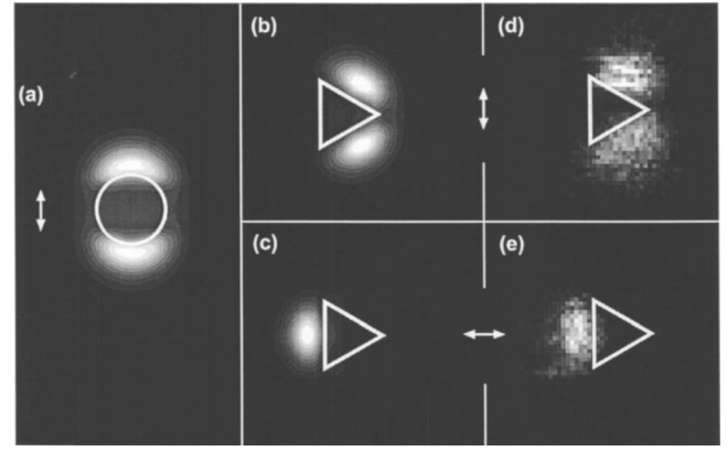
FIG. 3. Normalized electric field intensity computed at z = -10 nm for (a) a circular aperture and a polarization angle \phi = 90^\circ ; (b),(c) the same for a triangular aperture with (b) \phi = 90^\circ and (c) \phi = 0^\circ ; (d),(e) measured field map of a TA probe at a distance of \sim 10 nm from the triangular aperture for (d) \phi = 90^\circ and (e) \phi = 0^\circ . Location and shape of the respective apertures are marked by a white line; double arrows indicate the polarization direction of the incident light. Intensity scales linearly with grayscale; constant increments between successive contour lines in (a)–(c).
