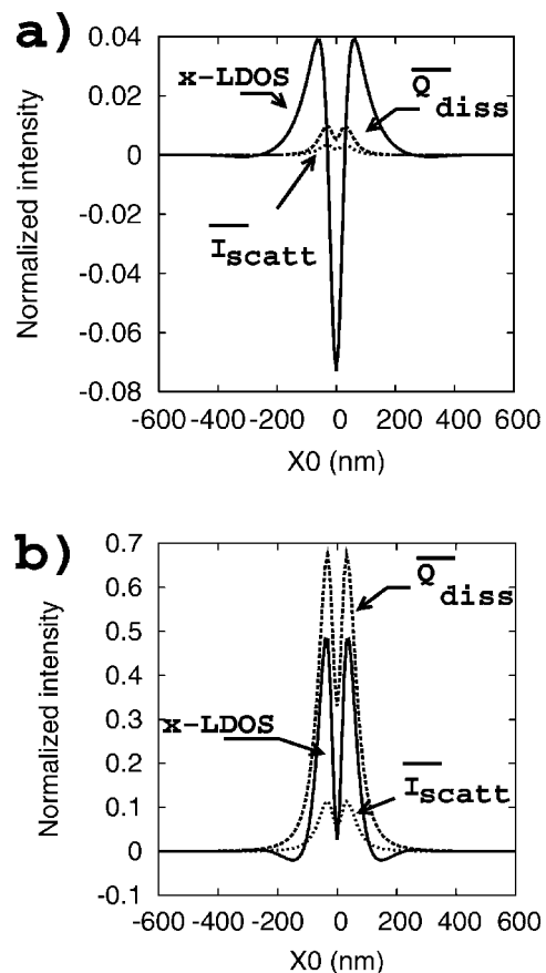
FIG. 3. Numerical simulation of the contributions to the total signal detected when a dipole is scanned over a single silver nanoparticle supported by a transparent surface. (a) Off-resonant wavelength ( \omega_0 = 2 eV). (b) Resonant wavelength ( \omega_0 = 3.2 eV). All the signals are normalized with respect to their value without the silver particle.
