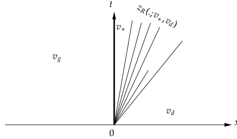
Figure 1.10: The third type of v -discontinuous solution : a stationary discontinuity followed by a R-wave whose left subwave is a rarefaction.
