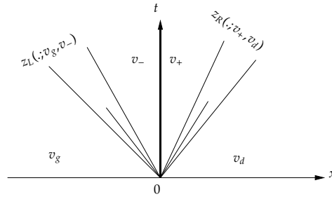
Figure 1.7: A v -discontinuous solution to the coupled Riemann problem
