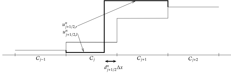
FIGURE 7.1: Principe de reconstruction
