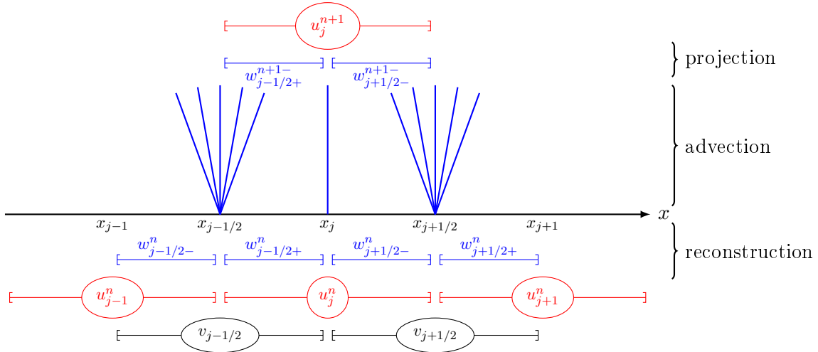
Figure 4.1: Numerical strategy
