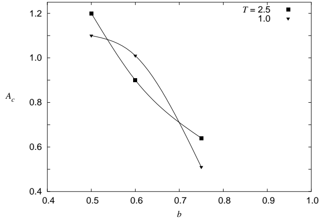
FIGURE 6.31: Critical pulse amplitudes, A_c , for the flow configurations analysed throughout section 6.3.5, for Reynolds number constant at Re = 300 , and pulse periods of T = 1.0 and 2.5 ( \alpha = 21.71 and 13.73 , respectively).
