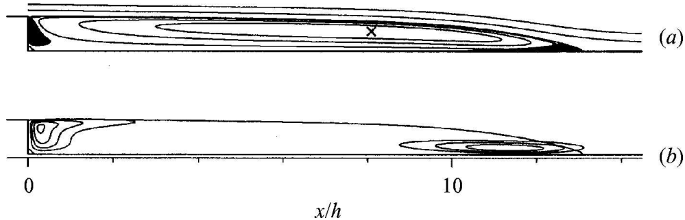
FIGURE 2.6: From Barkley et al. (2002), at Re = 750 , (a) regions (black) where the magnitude of the angular momentum decreases away from the centre (marked with a cross) of the recirculation zone. Representative streamlines are also shown. (b) Contours of the magnitude of the spanwise velocity component w or the critical instability eigenmode; the separating streamline of the base flow is also shown.
