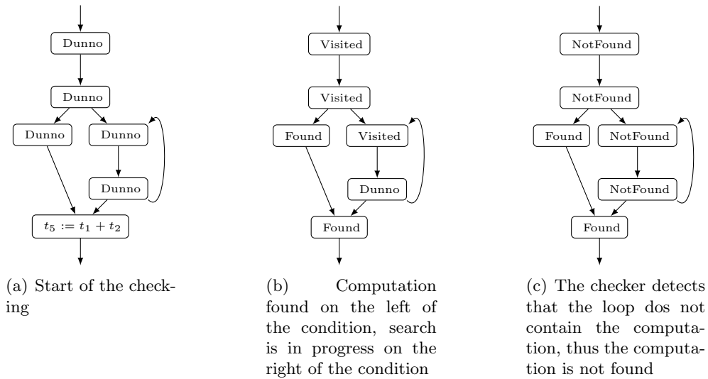
Figure 5.6: A few steps of the anticipability checking for computation t_1 + t_2 . (Only the node at the way out of the graph holds the computation.)
