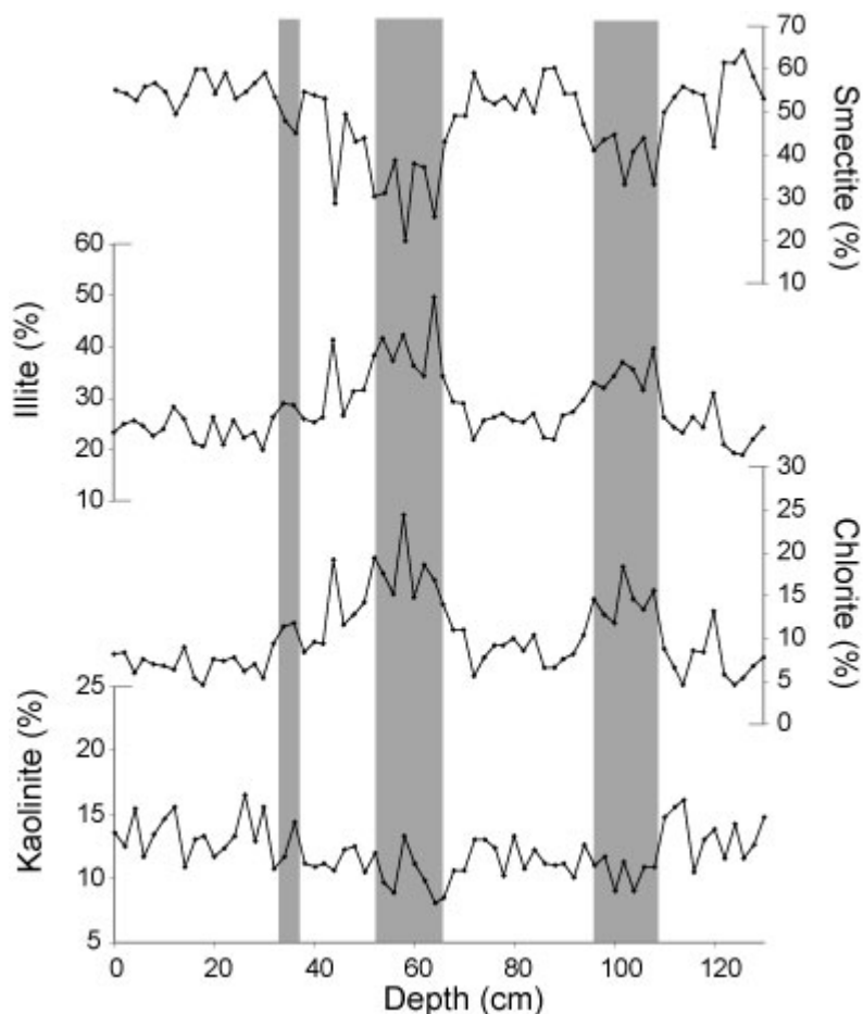
Figure 3.17 : 1.3 m of PB06 clay mineral analyses contents (%) obtained on the carbonated-free <2 \mu\text{m} size fraction. Smectite and illite are dominant (up to 75% of the total clay minerals). Illite and chlorite co-vary opposed to that of smectite. Kaolinite contents do not vary significantly with time. Shaded areas mark the main variations.
