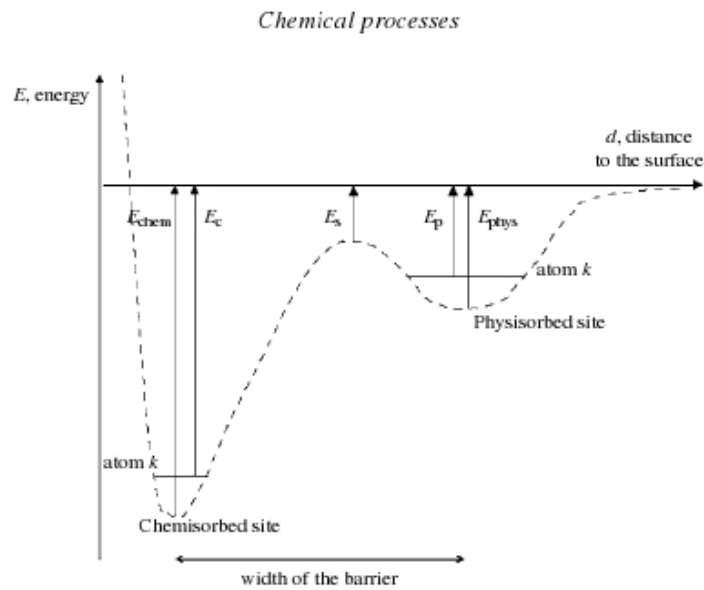
Figure 2.4.1: The interaction between an adsorbate and a surface as a function of the distance to the surface. Two types of sites can be recognized: physisorbed sites due to van der Waals interaction (binding energy, E_{phys} ) and chemisorbed sites involving shared electrons (binding energy, E_{chem} ). The actual binding energies of a species, E_p and E_c , take the zero-point energy into account. The two types of sites are separated by a saddle point with energy, E_s (from Tielens (2005)).
