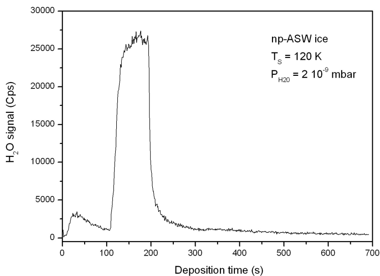
Figure 4.2.3: Example of \text{H}_2\text{O} deposition to grow np -ASW ice. In general, the deposition time depends on the number of monolayers that we want to grow. The surface temperature is set to 120 K and the \text{H}_2\text{O} partial pressure in the chamber to \sim 2 \cdot 10^{-9} mbar.
