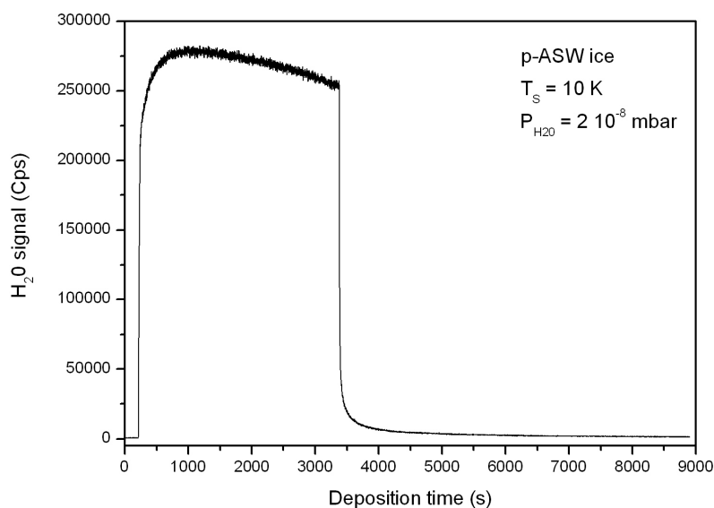
Figure 4.2.4: Example of \text{H}_2\text{O} deposition to grow p -ASW ice. The deposition time depends on the number of monolayers that we want to grow (monitored by a software applet connected to the pressure gauge). The surface temperature is set to 10 K and the \text{H}_2\text{O} partial pressure in the chamber to \sim 2 \cdot 10^{-8} mbar.
