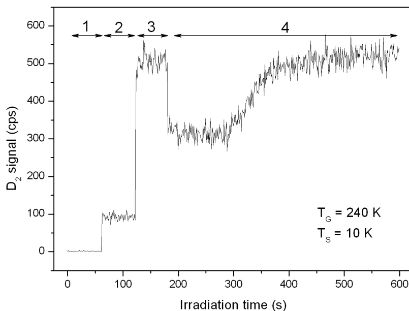
Figure 5.4.2: A typical sticking experiment. The signal is that of the mass 4 ( D_2 ) detected by the QMS during the irradiation of the surface with D_2 molecules.
