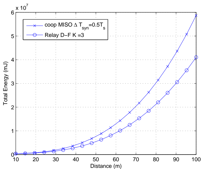
Figure 6.10: Energy consumption of relay technique vs. cooperative MISO technique with two transmission nodes N = 2 , power path-loss factor K = 3 , error rate FER = 10^{-2} , transmission synchronization error range \Delta T_{syn} = 0.5T_s and source-relay distance d_1 = d/3 .
