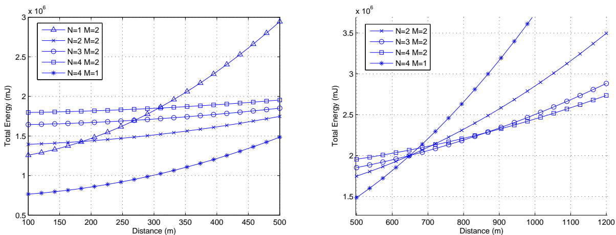
Figure 3.9: Energy consumption of cooperative MIMO and cooperative MISO systems, N = 2, 3, 4 and M = 2 cooperative transmit and receive nodes, FER = 10^{-3} requirement, Rayleigh fading channel with power path-loss factor K = 2 .
