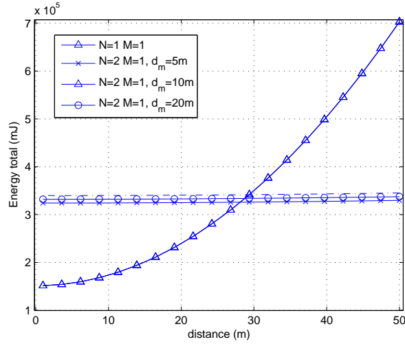
Figure 3.14: Energy consumption of the cooperative MISO 2 – 1 with different cooperative transmission distances d_m = 5, 10 and 20m , FER = 10^{-3} requirement, Rayleigh fading channel with power path-loss factor K = 2 .
