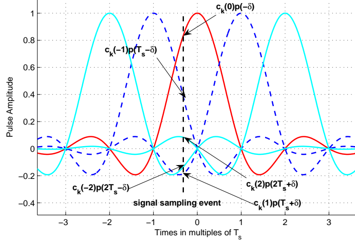
Figure 4.2: ISI of un-synchronized sequence with the synchronization error \delta
