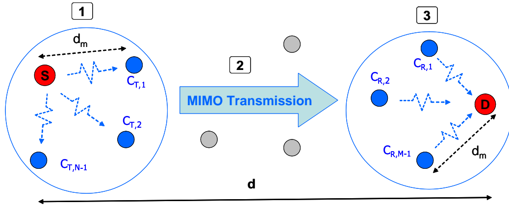
Figure 2.8: Cooperative MIMO transmission scheme from S to D with N - 1 cooperative transmission nodes ( C_{T,1}, C_{T,2}, \dots, C_{T,N-1} ) and M - 1 cooperative reception nodes ( C_{R,1}, C_{R,2}, \dots, C_{R,M-1} ).
