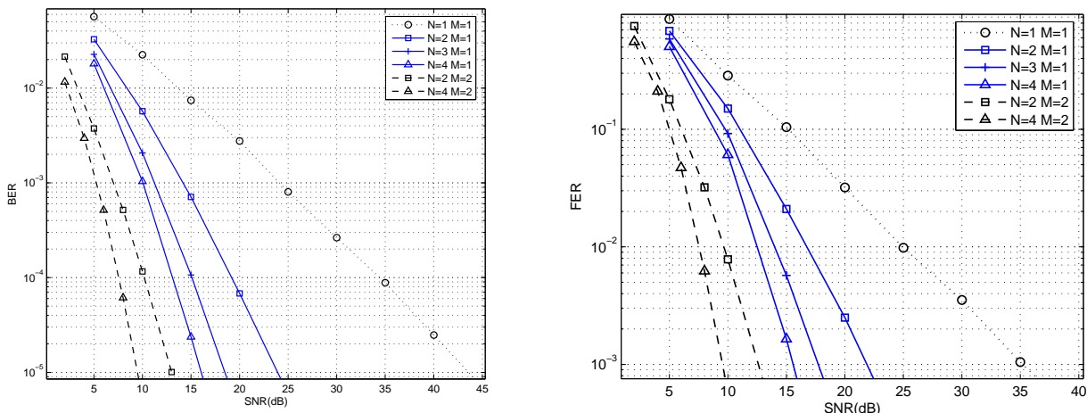
Figure 3.1: BER and FER performance of STBC for various number of transmit and receive antennas ( N and M ) over a Rayleigh fading channel.
