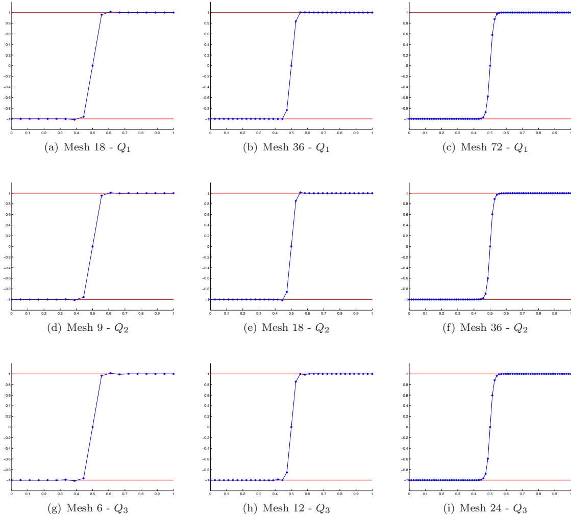
Figure 3.16: Fitted curves on the "tanh-profile".
