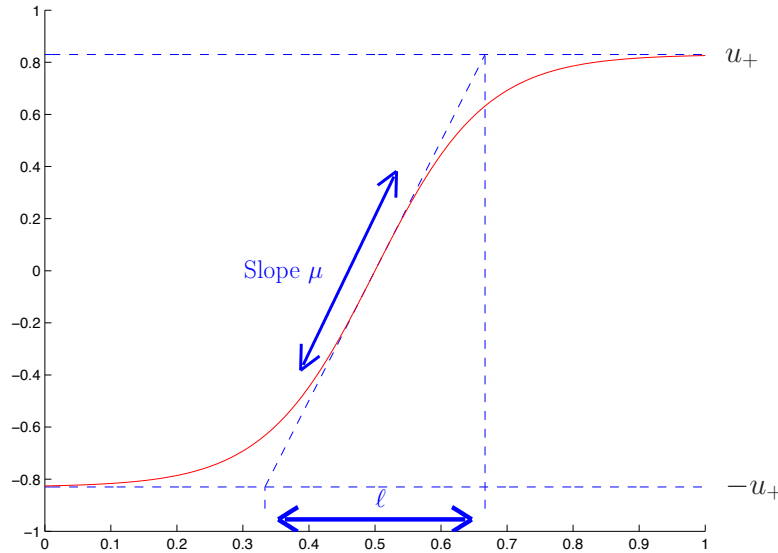
Figure 3.7: Interface length for the solution u_4 .
