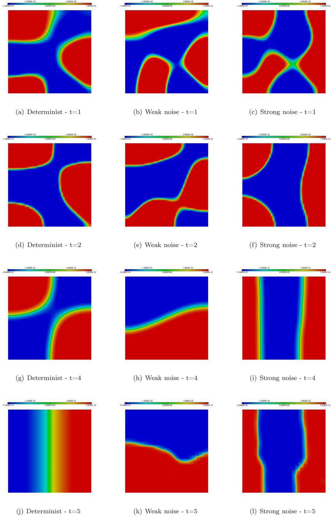
Figure 3.38: Spinal decomposition under the classic quartic double-well potential.
