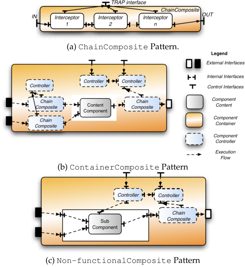
Figure 5.5: Architectural Patterns
