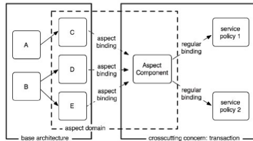
Figure 3.8: FAC: Functional and Aspect Components Example
