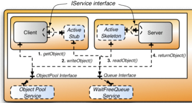
Figure 5.13: Cross-Thread Communication
