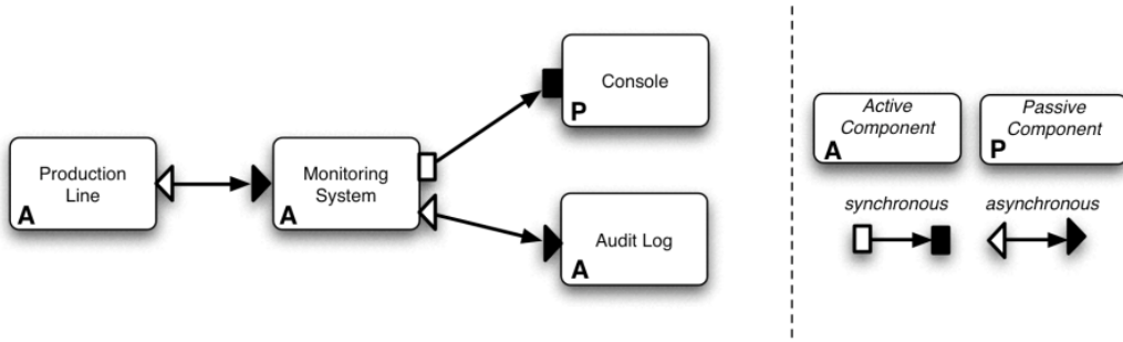
Figure 4.14: Functional View
