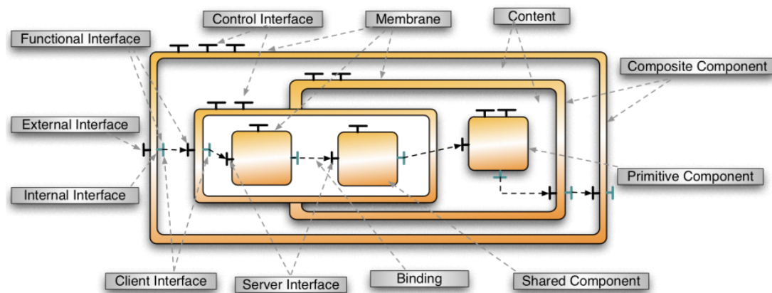
Figure 3.6: FRACTAL Concepts
