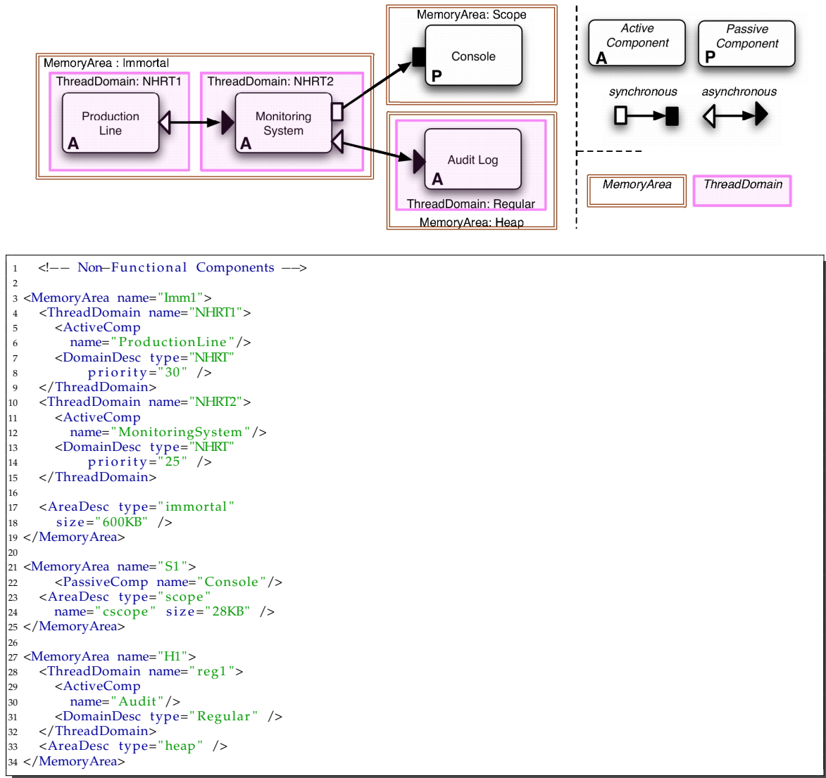
Figure C.2: SweetFactory Architecture in FRACTAL-ADL, Part 2
