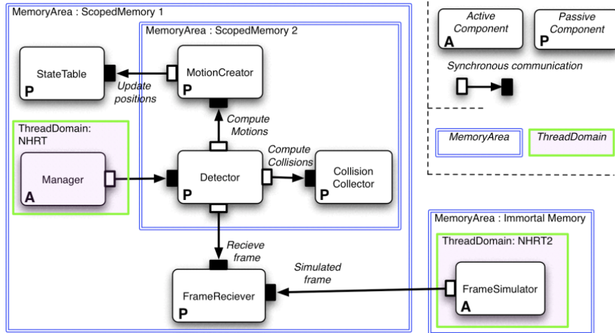
Figure 6.5: RCD Architecture
