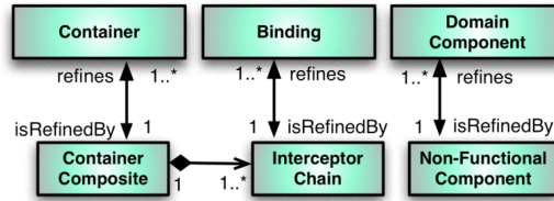
Figure 5.4: Architectural Patterns
