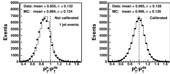
Figure 20: P_T^h/P_T^{da} distribution for one jet events, before (left) and after (right) the application of the jet calibration. The mean and \sigma values are obtained using a Gaussian fit to the central part of the distributions.
