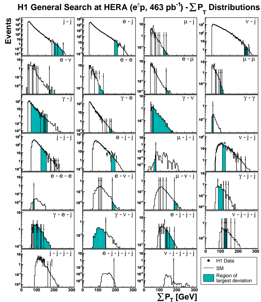
Figure 2: The number of data events and the SM expectation as a function of \sum P_T for classes with at least one event. The shaded areas show the regions of largest deviation identified by the search algorithm. No such search is performed for the j-j-j-j , e-j-j-j-j and \nu-j-j-j-j classes.
