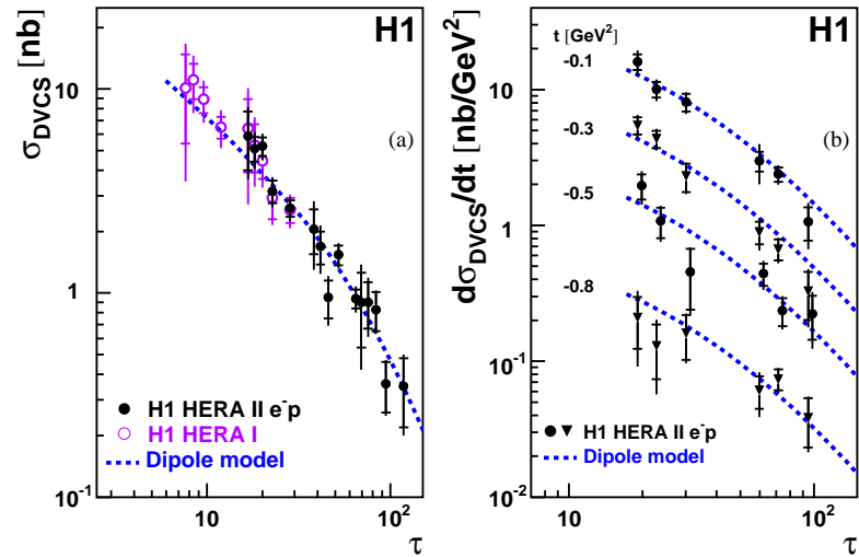
Figure 6: DVCS cross section measurements as a function of the scaling variable \tau = Q^2/Q_s^2(x) . In (a) the results are shown for the full t range |t| < 1 GeV 2 and in (b) at four values of t . The cross section measurements from the previous H1 publication [8] are also shown in (a). The inner error bars indicate the statistical errors, the outer error bars the statistical and systematic errors added in quadrature. The dashed curves represent the predictions of the dipole model [12, 14].
