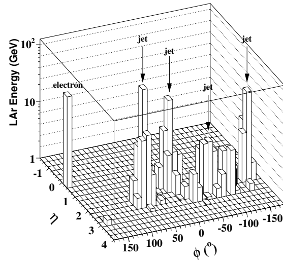
Figure 4: The calorimetric energy deposits of the e-j-j-j-j event as a function of \eta and \phi .
