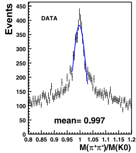
Figure 16: K_0 mass spectrum (normalised to the K_0 mass) obtained with the \mu ODS standard H1PartK0Finder . The invariant mass of the two pions is computed using the good quality tracks. The mean of a Gaussian fit (blue line) is centered to one with less than 1 % deviation.
