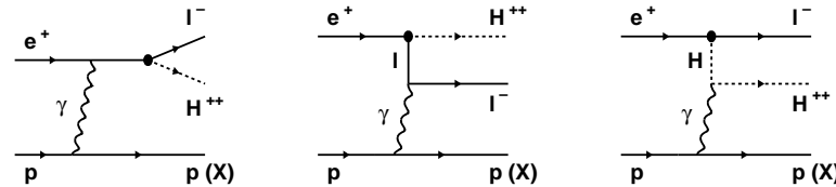
Figure 1: Diagrams for the single production of a doubly-charged Higgs boson in e^+p collisions at HERA via the h_{el} coupling. The hadronic final state is denoted by p ( X ) in the elastic (inelastic) case, where the initial proton remains intact (dissociates). The contribution of Z exchange can be safely neglected.
