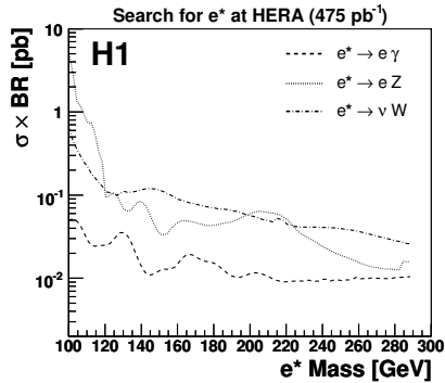
Figure 2: Upper limits at 95% CL on the product of the e^* cross section and decay branching ratio, \sigma \times BR , in the three e^* decay channels as a function of the excited electron mass. The decay channels of the W and Z gauge bosons are combined. Areas above the curves are excluded.
