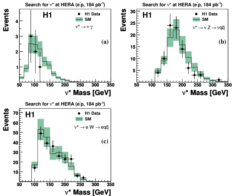
Figure 1: Invariant mass distribution of the \nu^* candidates for the \nu^* \rightarrow \nu \gamma (a), \nu^* \rightarrow \nu Z \rightarrow \nu q \bar{q} (b) and \nu^* \rightarrow e W \rightarrow e q \bar{q} (c) searches. The points correspond to the observed data events and the histogram to the SM expectation after the final selections. The error bands on the SM prediction include model and experimental systematic errors added in quadrature.
