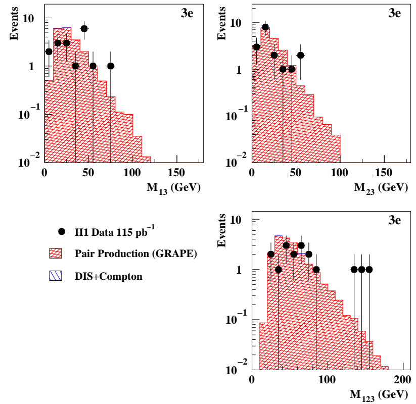
Figure 6: Invariant mass distributions of electron pairs 1-3 and 2-3 (top left and right) and of the tri-electron system (bottom right) for events classified as "3e".
