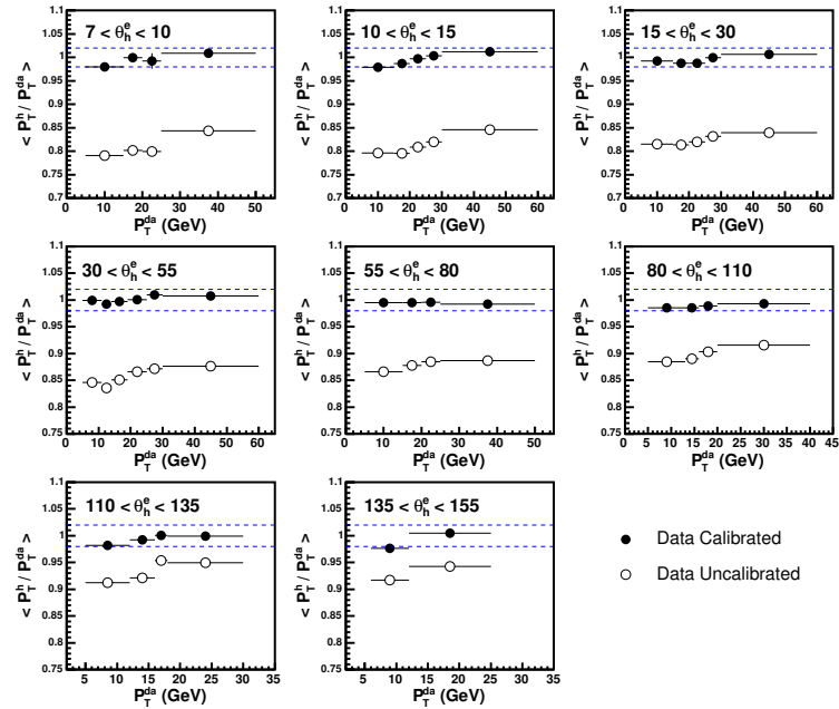
Figure 25: Evolution of the mean values of the P_T^{bal} distributions for data with P_T^{da} for the inclusive check sample in the different \theta_h^e regions, before (open circles) and after (solid circles) application of the calibration. This example is for 1999p-2000 data.
