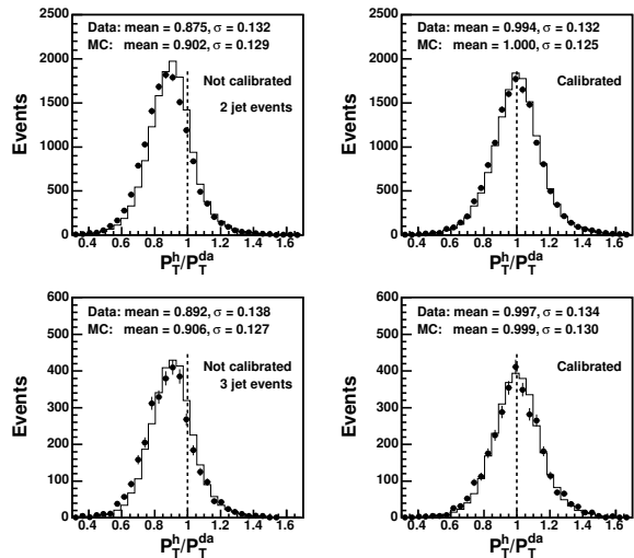
Figure 22: P_T^h / P_T^{da} distributions for two (upper figures) and three (bottom figures) jets events, before (left) and after (right) the application of the jet calibration. The mean and \sigma values are obtained using a Gaussian fit to the central part of the distributions.
