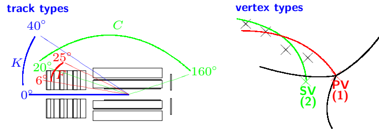
Figure 1: Different track types and their angular domain, and the two vertex hypothesis for a single track. Both primary and secondary vertex fitted tracks can be selected.
