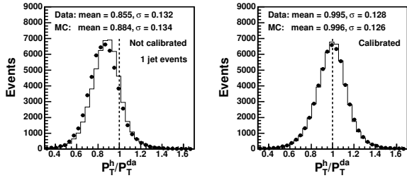
Figure 20: P_T^h/P_T^{da} distribution for one jet events, before (left) and after (right) the application of the jet calibration. The mean and \sigma values are obtained using a Gaussian fit to the central part of the distributions.
