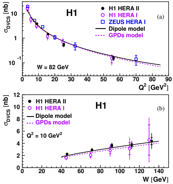
Figure 2: The DVCS cross section \gamma^* p \rightarrow \gamma p as a function of Q^2 at W = 82 \text{ GeV} (a) and as a function of W at Q^2 = 10 \text{ GeV}^2 (b). The results from the previous H1 [10] and ZEUS [12] publications based on HERA I data are also displayed. ZEUS measurements are propagated from W = 104 \text{ GeV} to 82 \text{ GeV} using a W dependence W^{0.52} . The inner error bars represent the statistical errors, the outer error bars the statistical and systematic errors added in quadrature. The dashed line represents the prediction of the GPDs model [6] and the solid line the prediction of the dipole model [15].
