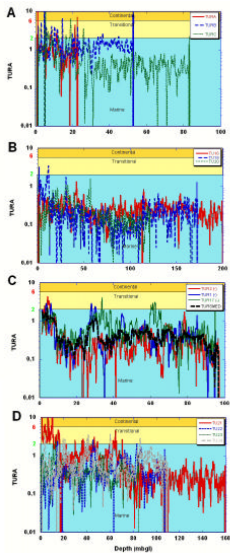
Figure P2- 19. Thorium/ Uranium ratio curves vs. depth in wells of (A) Cap Blanc, (B) Llucmajor (C) Ses Sitjoles and (D) Ses Salines sites. Similar plots are available for Ses Sitjoles wells of Campos site in Maria-Sube, submitted.
