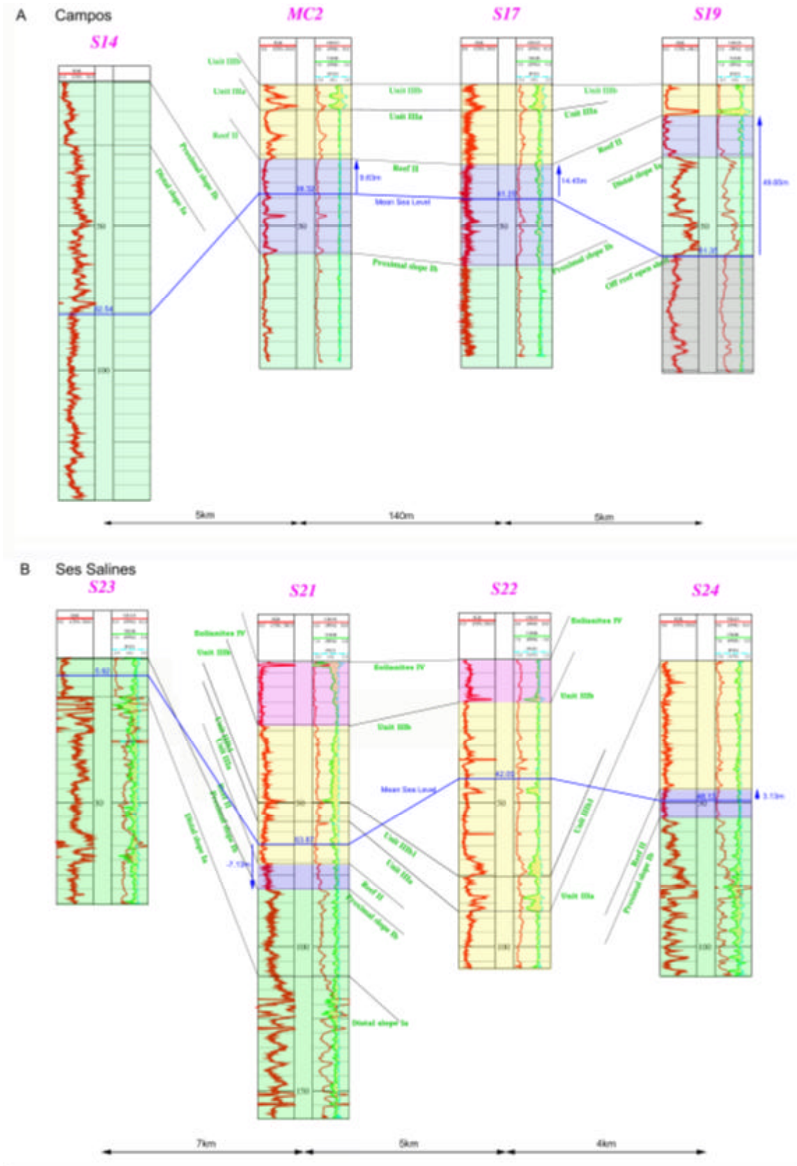
Figure P2- 16. SGR facies correlation over Campos and Ses Salines sites. Same scales and colour coding as on Fig. 15. (A) SGR Unit correlation over Campos site wells S14, MC2, S17 and S19. No spectral GR tool could be run on S14, only a total natural GR with roughly four times less CPS than for the Spectral GR; for this reason, the display scale was divided by four, for comparison purposes with the other wells. (B) SGR Unit correlation over Ses Salines site wells S21 to S24.
