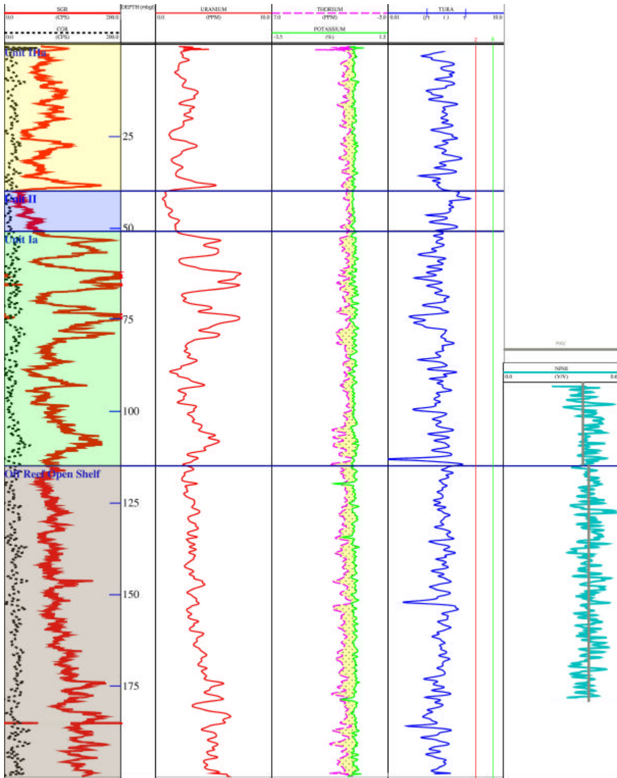
Figure P2- 13. SGR log in S16 well of Lluçmajor site. Same color coding as for Fig. P2-10, P2-11 and P2-12, with Off reef open shelf color coded light gray. Neutron porosity log in the right track ; average porosity PAV (from neutron porosity log) is indicated with a thick grey line. Note the very high porosity in the off reef open shelf, even higher than in Unit Ia.
