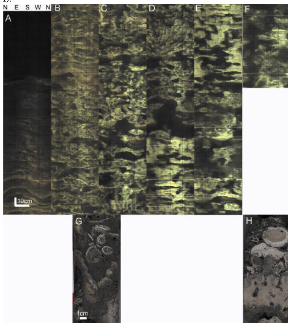
Figure P2- 23. Site MOO09B borehole high resolution full 360° optical images (A to F) and interval corresponding core slab photos (G and H); image logs and core slab are presented one on top of the other, when the core depth is included in the image log interval. (A) Optical image interval 5.32- 7.62mbsf, subunit IB: coralgal- microbialite frameworks dominated by branching and encrusting colonies of Porites and Montipora ; observe cross-stratifications in the bottom 50cm (channel?). (B) Optical image interval 7.62- 10.04mbsf, subunit IA, coralgal- microbialite frameworks (bindstone) dominated by encrusting colonies of Montipora , Montastraea , Leptastrea , Pavona and Porites and encrusting and foliaceous colonies of agariciids ( Pachyseris and Leptoseris ); other corals are less abundant and include branching colonies of Porites (see description Fig. 22G) and Pocillopora . (C) Optical image interval 10.04- 12.46mbsf, subunit IA (see description Fig. 22B). (D) Optical image interval 12.46- 14.87mbsf, subunit IC, coral assemblage dominated by massive colonies of Porites ; associated coral colonies include encrusting and branching Porites , robust branching Pocillopora , and encrusting Montipora ; branching corals are distinguished in the top 70cm. (E) Optical image interval 14.87- 17.29mbsf, subunits IC (14.87- 16.6mbsf, see description Fig. 22D) and IB (16.6- 17.29mbsf, see description Fig. 22A), massive corals. (F) Optical image interval 17.29- 18.24mbsf, subunit IB, see description Fig. 22A; coral colonies are coated with crusts of nongeniculate coralline algae up to 2.5cm thick, nongeniculate coralline algae algal crusts are generally overlain by microbialites (see description Fig. 22H). (G) Core 9R-1, within interval 8.8-10.7mbsf, subunit IA, coral framework of branching Porites colonies with coralline algae and microbialites. (H) Core 13R-1, within interval 16.6- 18.5mbsf, subunit IB, tabular colony of Acropora , note thick crusts of coralline algae covering tips of coral branches; sediments matrix contains abundant Halimeda segments (Camoin et al., 2006).
