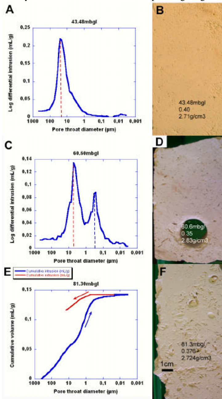
Figure P3- 8. Examples of Hg porosimetry results on MC2 samples. (A) Differential intrusion vs. pore throat diameter, at 43.48 mbgl showing a monomodal distribution of pore throats. (B) core slab photo at 43.48 mbgl (depth, porosity and grain density are indicated); the grain density value suggests that this rock is mostly pure calcite. (C) Differential intrusion vs. pore throat diameter, at 60.6 mbgl, showing a bimodal distribution of pore throats, with dominant pore throat diameters at 7 and 0.5 \mu\text{m} . (D) Core slab photo at 60.6 mbgl; the grain density value suggests that there is a high percentage of dolomite in this calcitic rock; compare with Fig. 5J at 60.92 mbgl thin section showing dolomitic cement. (E) Cumulative intrusion (increasing pressure, blue curve) and extrusion (decreasing pressure, red curve) at 81.3 mbgl showing trapped porosity. (F) Core slab photo at 81.3 mbgl, displaying moldic porosity.
