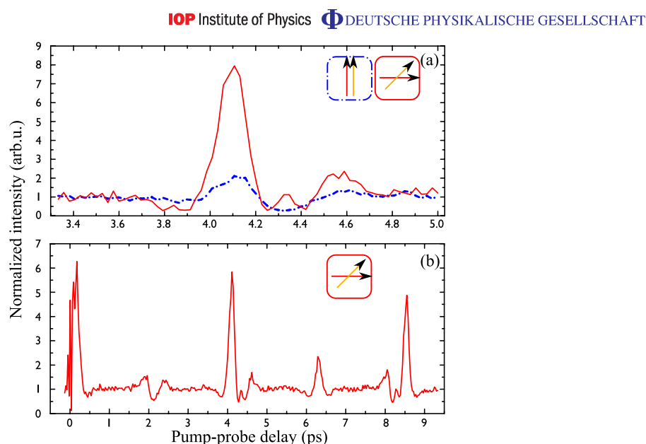
Figure 6. Pump–probe scans in \text{N}_2 , with a pump intensity of 5 \times 10^{13} \text{ W cm}^{-2} and a probe intensity of 1.2 \times 10^{14} \text{ W} \cdot \text{cm}^{-2} . (a) Evolution of the H21 signal as a function of pump–probe delay in two configurations. Conventional configuration (blue): the pump and probe pulse polarizations are parallel and the analyzing waveplate is rotated to maximize the reflection on the polarizer (S polarization). Polarization-resolved spectroscopy (red): the pump-pulse polarization is rotated by 40^\circ with respect to the probe. The analyzing waveplate is rotated so that the probe pulse is P polarized on the polarizer. (b) Evolution of the H19 intensity as a function of pump–probe delay over a full-rotational period of \text{N}_2 , in the polarization resolved spectroscopy configuration.
