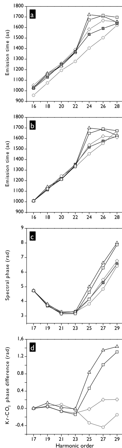
Figure 3.3. The steps of data analysis: from the measured emission times to the DME phase. These data are some of those plotted in figure 3 in paper I: Krypton (■), \text{CO}_2 aligned at \theta = 0^\circ (□), 10^\circ (△), 30^\circ (◇) and 90^\circ (⊙). Emission times as measured (a), Emission times with normalized absolute timing (b), phase obtained by integrating the emission times (c), \text{CO}_2 -phases normalized by the krypton phase (d). Error bars are omitted for clarity; they have about the size of the symbols.
