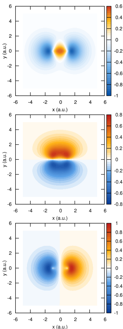
Figure 1.5. Projection of N_2 orbitals onto the x - y -plane. The inter-nuclear axis is along the x -axis and the inter-nuclear distance is R = 2 a.u.. Upper: \phi_{3\sigma_g}(\mathbf{r}) – the HOMO of N_2 . This MO is dominated by a (\psi_{2p_x} - \psi_{2p_x}) combination. Middle: One of the two degenerate \phi_{1\pi_u}(\mathbf{r}) – the HOMO-1 of N_2 . This MO is dominated by a (\psi_{2p_y} + \psi_{2p_y}) combination. Lower: \phi_{2\sigma_u}(\mathbf{r}) – the HOMO-2 of N_2 . This MO is dominated by a (\psi_{2s} - \psi_{2s}) combination.
