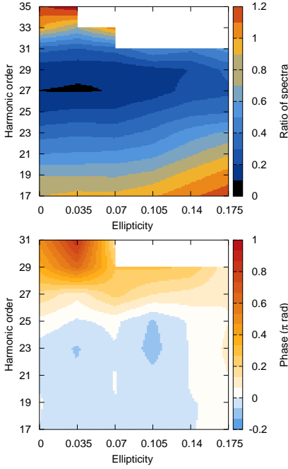
Figure 3.6. Harmonic spectra measured with \text{CO}_2 aligned at \theta = 0 , normalized by those measured with \theta = 90^\circ (upper panel), and difference of spectral phase \varphi_{\text{CO}_2}(\omega, \theta = 0^\circ) - \varphi_{\text{CO}_2}(\omega, \theta = 90^\circ) (lower panel), as function of the driving laser ellipticity. The white area in the upper right of both plots notes missing data – at higher ellipticities, the highest harmonic orders can no longer be detected reliably. Note that the phase is plotted up to harmonic 31 only, whereas the spectral ratio is plotted up to H35.
