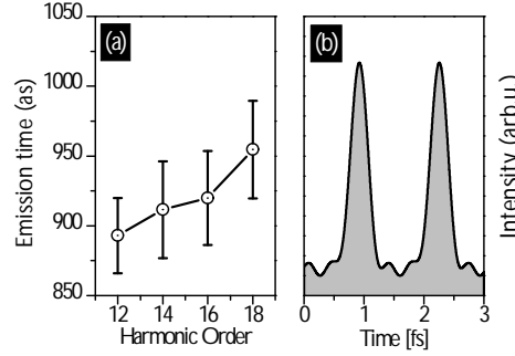
Figure 3: Emission times and phase of consecutive harmonics
