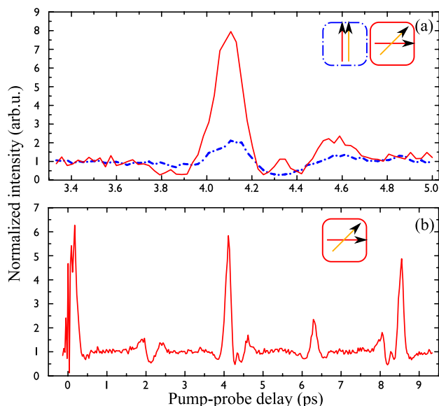
Figure 6. Pump–probe scans in \text{N}_2 , with a pump intensity of 5 \times 10^{13} \text{ W cm}^{-2} and a probe intensity of 1.2 \times 10^{14} \text{ W} \cdot \text{cm}^{-2} . (a) Evolution of the H21 signal as a function of pump–probe delay in two configurations. Conventional configuration (blue): the pump and probe pulse polarizations are parallel and the analyzing waveplate is rotated to maximize the reflection on the polarizer (S polarization). Polarization-resolved spectroscopy (red): the pump-pulse polarization is rotated by 40^\circ with respect to the probe. The analyzing waveplate is rotated so that the probe pulse is P polarized on the polarizer. (b) Evolution of the H19 intensity as a function of pump–probe delay over a full-rotational period of \text{N}_2 , in the polarization resolved spectroscopy configuration.
