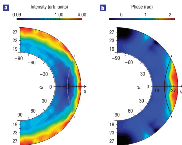
Figure 3 Experimental spectral intensity and phase of the CO 2 harmonic emission normalized by that of Kr. CO 2 harmonic intensity and phase (measured for molecule angles from 90° to 0°) normalized to the krypton data taken under the same experimental conditions (intensity of 0.95 \times 10^{14} \text{ W cm}^{-2} ). To prevent the dispersion effects due to the larger ionization rate of Kr, the corresponding data were taken at lower pressure (25 torr versus 60 torr for CO 2 ) ensuring good phase-matching conditions. The dashed lines are the same as the one shown in Fig. 1b converted to harmonic order. The relation between the measured data and the recombination dipole moment is given in the Methods section. a , Intensity ratio versus alignment angle \theta (measured in steps of 5°) and harmonic order q . The ratio is not corrected for the different pressures. A clear intensity minimum is measured around harmonic 23 for \theta = 0 that disappears when the molecule is rotated. b , Spectral phase difference (as in Fig. 2b), measured in steps of 10°. A phase jump of 2 rad is observed at the same position as the intensity minimum.
