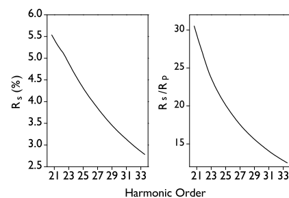
Figure 3.22. Reflectivity of a pair of silver mirrors with 60° incidence (defined with respect to the surface normal) for s-polarized light (left). Reflectivity ratio for s- and p-polarized light (right), i.e. the extinction ratio of the polarizer. These data are based on (Henke et al. [72]).
