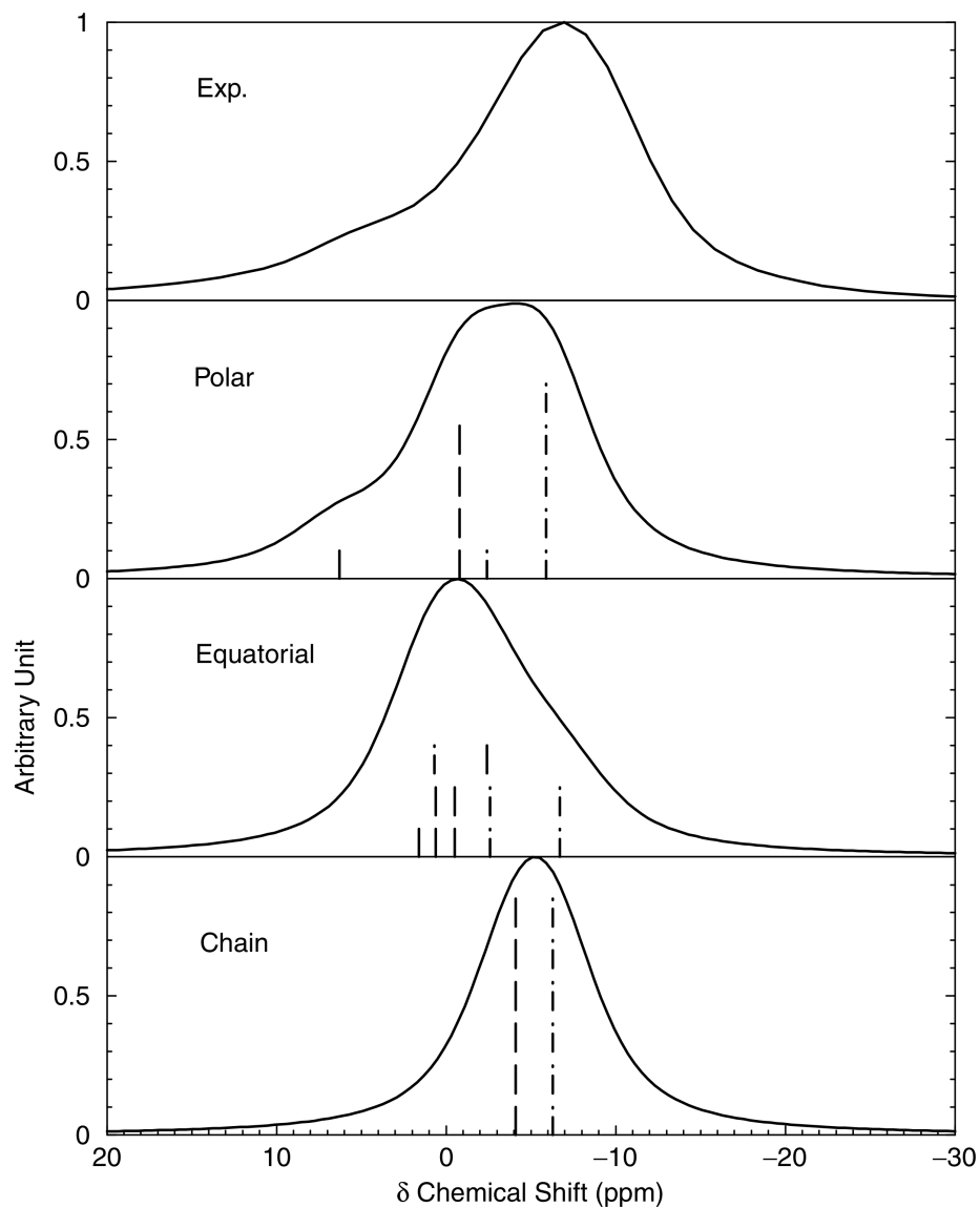
Figure 5.4: \text{B}_4\text{C} : ^{11}\text{B} NMR chemical shift spectrum. Experimental data is from Ref. [131] and theory for the polar , equatorial and chain models from Ref. [42].
