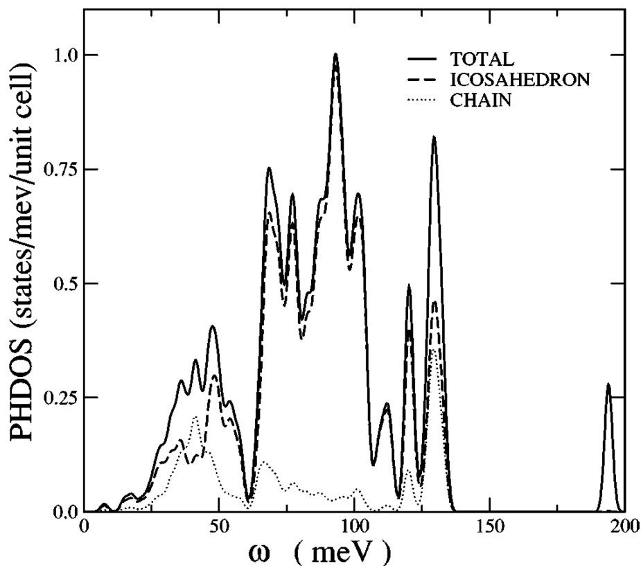
Figure 5.6: Phonon density of states of B_{13}C_2 from Ref. [6]. Solid line : total DOS. Dashed line : contribution from the vibrations of the icosahedron. Dotted line : contribution from the phonon modes of the chain.
