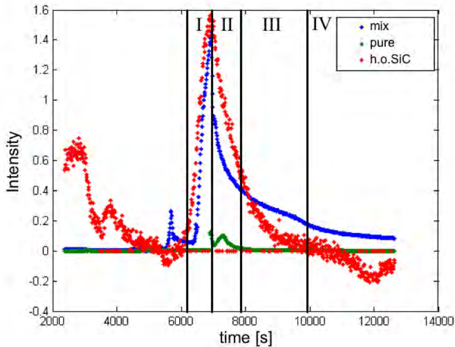
Figure 4.1: Domains of Arrhenius evolution (I), powder aging and SiO 2 elimination (II), active oxidation (III) and carbon precipitation(IV) displayed on: a) SiO(g) partial pressure measured during vaporization experiments in HTMS compared to p(\text{SiO}) calculated for congruent SiO 2 pure vaporization and for SiO 2 /SiC vaporization at interface. b) CO(g) intensities from experiments in mass spectrometer reactor with capillary tubing.
