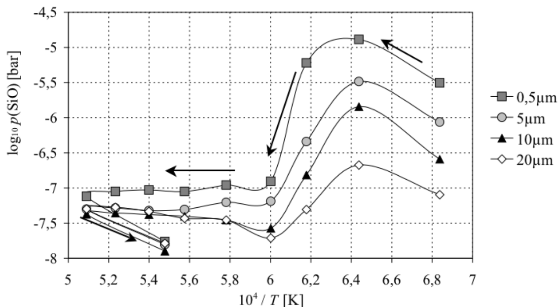
Figure 3.15: Decimal logarithm of SiO(g) partial pressure for powders from the SiC-05m experiment as a function of the inverse of temperature.
