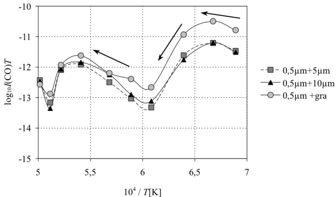
Figure 3.19: Logarithm of I \cdot T products for CO(g) as a function of the inverse of temperature from different grain sizes mixtures. Arrows show the evolution with time.
