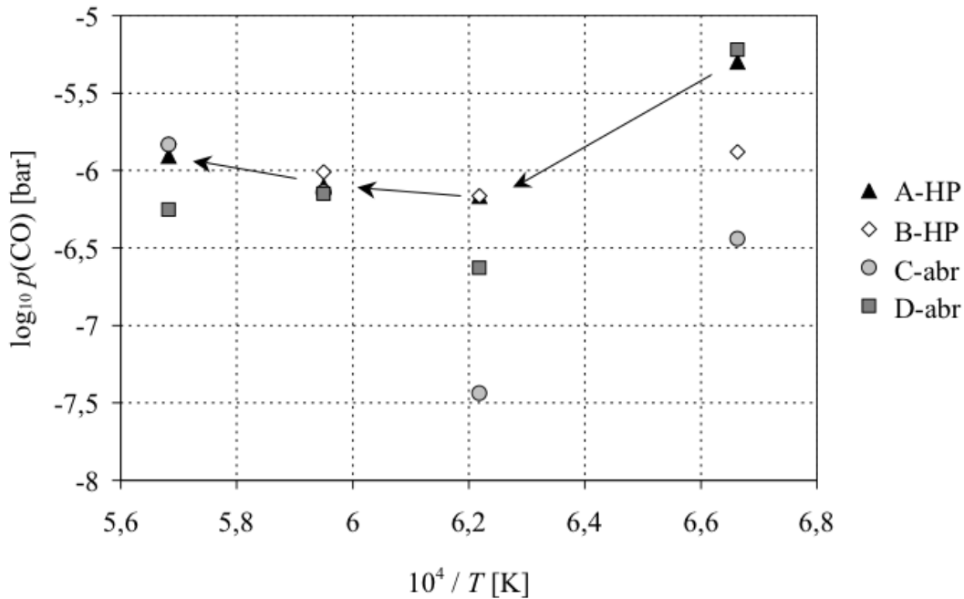
Figure 3.12: Decimal logarithm of CO partial pressure for powders from the SiC-2m experiment as a function of the inverse of temperature. Arrows show evolution with time.
