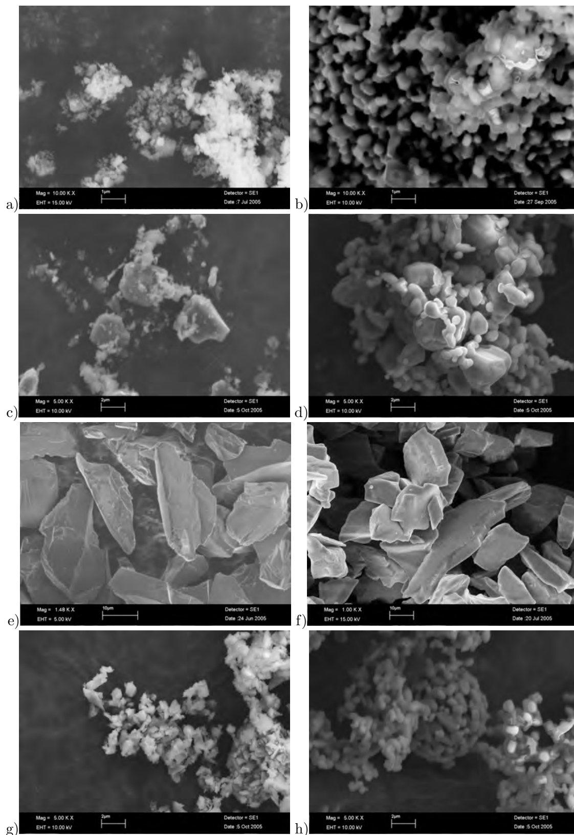
Figure 3.23: SEM images of sample powders for SiC-02m experiment. a) A-HP initial powder; b) A-HP after experiment; c) B-HP initial powder; d) B-HP after experiment; e) C-abr initial powder; f) C-abr after experiment; g) D-abr initial powder; h) D-abr after experiment
