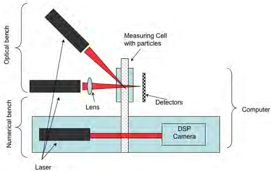
Figure 3.9: Grain size measurement principle of the CILAS 1064.
