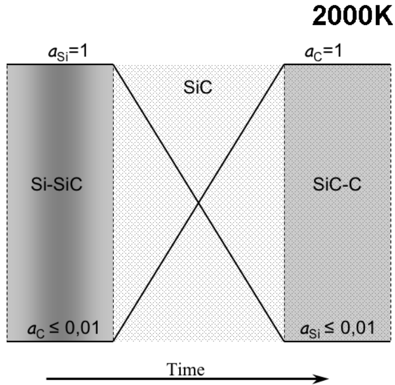
Figure 2.4: Isothermal evolution of the activities of Si and C components in the stoichiometric domain of SiC, displayed by enlarging intentionally this domain.
