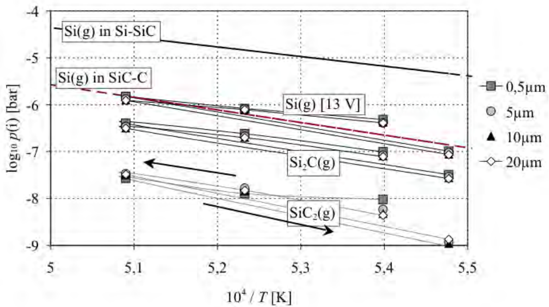
Figure 3.17: Decimal logarithm of Si, Si 2 C and SiC 2 partial pressures for powders from the SiC-05m experiment as functions of the inverse of temperature. Arrows show the evolution with time.
