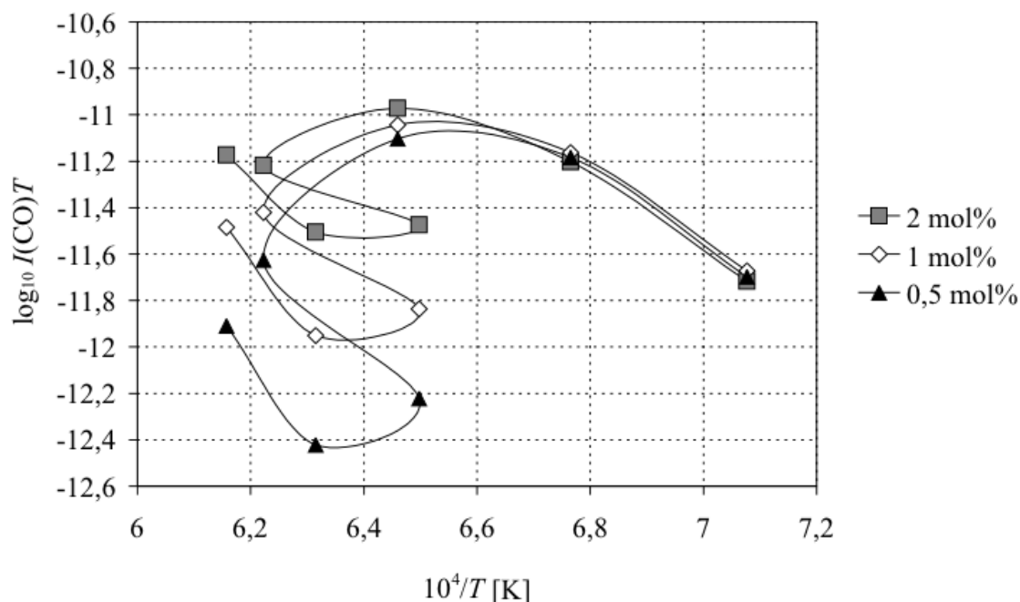
Figure 3.34: Evolution of the decimal logarithm of I(\text{CO}) \cdot T for SiC-SiO 2 mixtures with 2, 1 and 0,5 mol% SiO 2 content as a function of the inverse of temperature.
