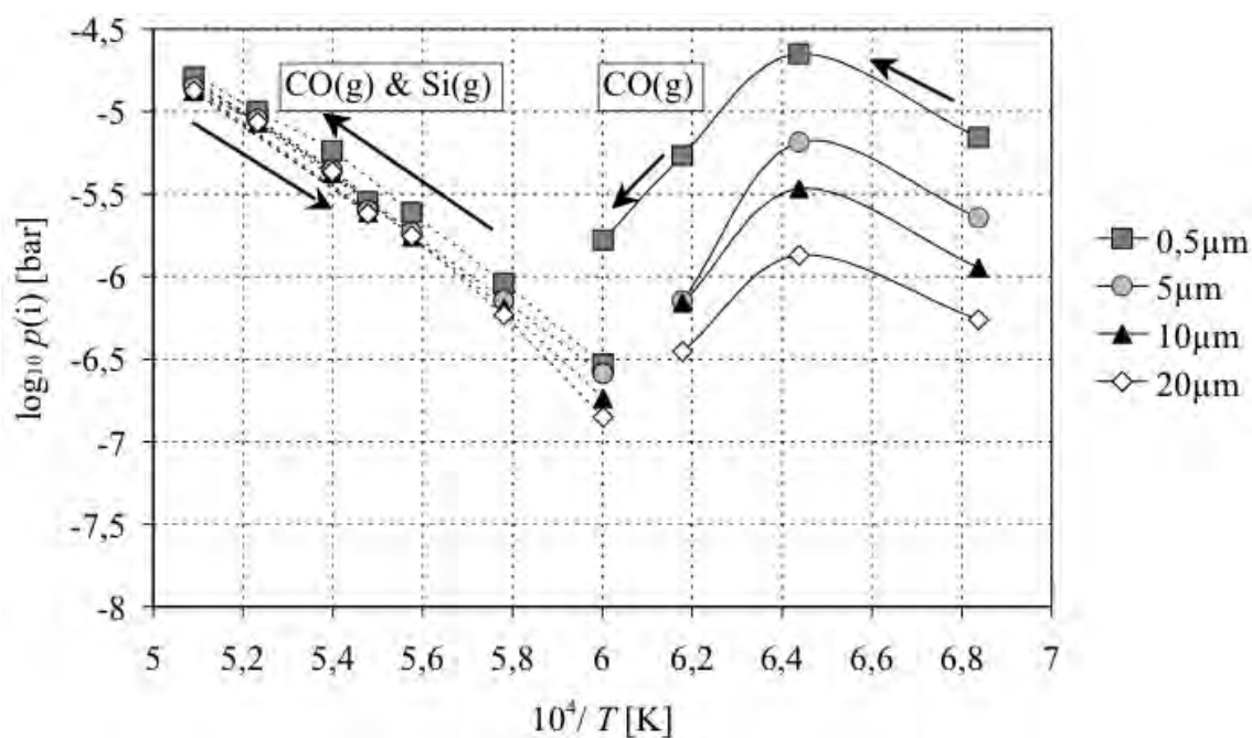
Figure 3.16: Decimal logarithm of CO(g) partial pressure for powders from the SiC-05m experiment as a function of the inverse of temperature.
