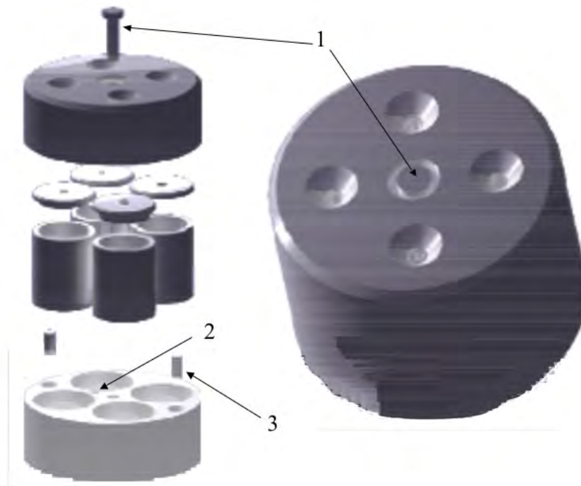
Figure 3.4: Multiple cell device. 1: Pin used for black body of the axial hole. The pyrometric viewing is done from the bottom. 2: Bottom hole for thermocouple going into the upper envelope. 3: Tungsten tips for correct assembling of the upper and bottom envelopes of the multiple cell.
