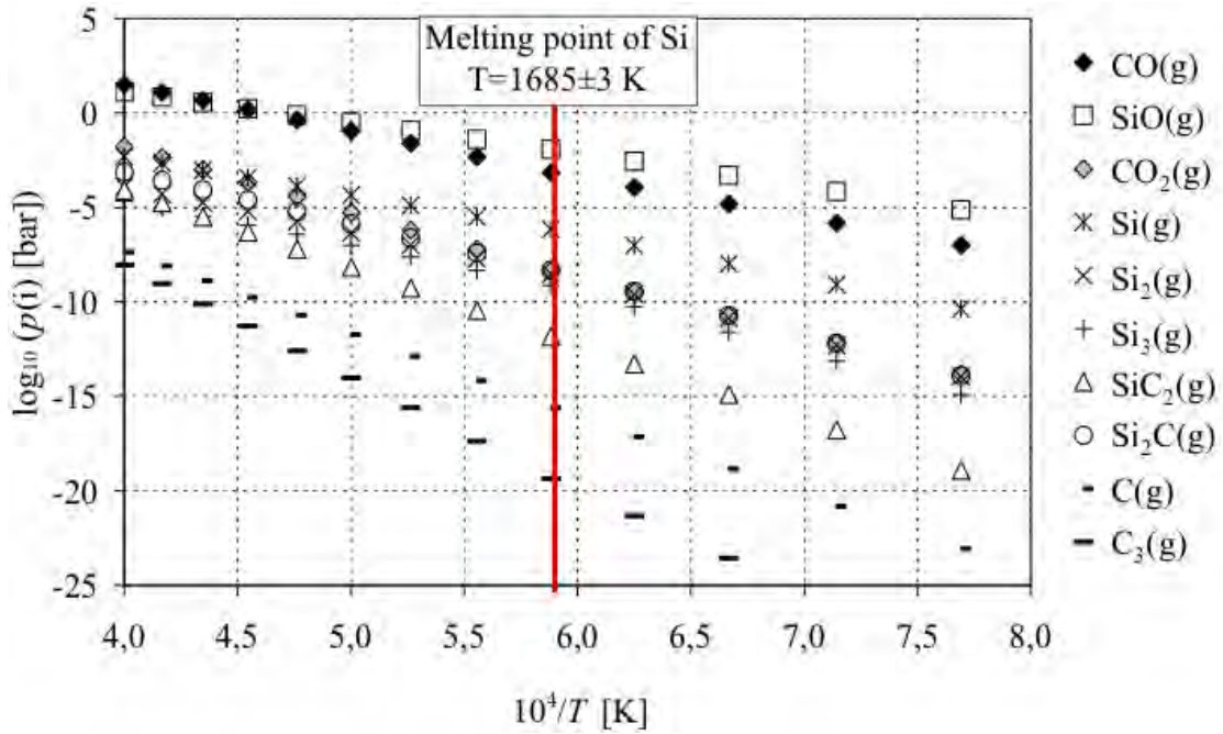
Figure 2.10: Decimal logarithmic plot of partial pressures in equilibrium with three-phases domain SiC-SiO 2 -Si as a function of the inverse of temperature [K]. After melting point of Si at T = 1685 K the slope of the curves changes.
