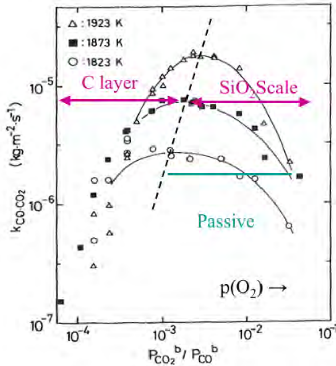
Figure 1.5: Relationship between k_{\text{CO}\cdot\text{CO}_2} and p_{\text{CO}_2}^b/p_{\text{CO}}^b/ from [44].
