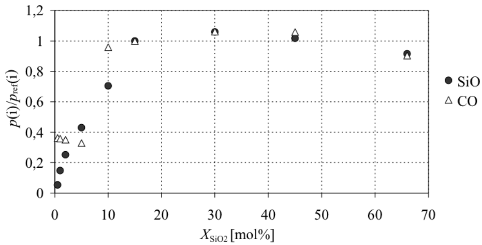
Figure 3.35: Relative partial pressures of SiO(g) and CO(g) as a function of powder composition of different samples referenced to 15 mol% at 1625 K.
