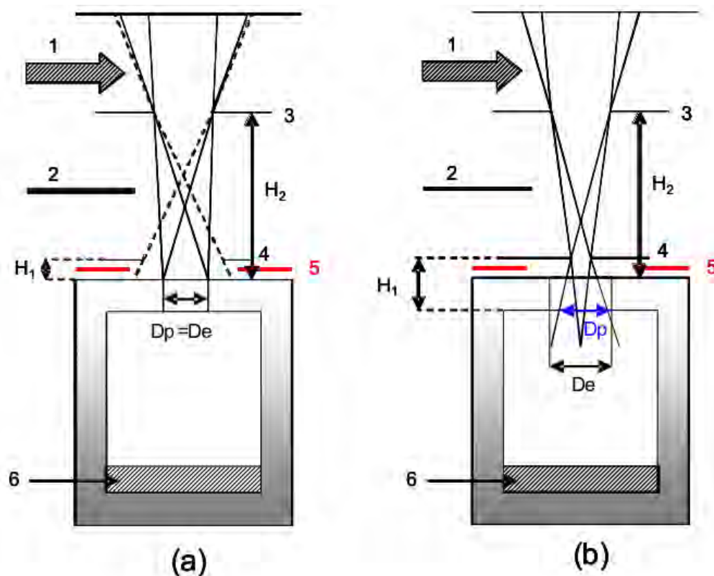
Figure 3.6: Conventional collimation (a) and restricted collimation (b) of molecular flow from effusion cell with different sampling apertures. 1: Electron beam. 2: Movable free shutter. 3: Source aperture. 4: Field aperture water cooled. 5: Furnace thermal shields. 6: Sample. D_p is the penumbra diameter and D_e is the effusion orifice diameter. [96]
