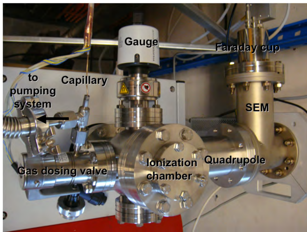
Figure 3.7: Experimental arrangement with quadrupole mass spectrometer and capillary tubing: a) arrangement order of single components and b) a photograph to display orthogonal arrangements.
