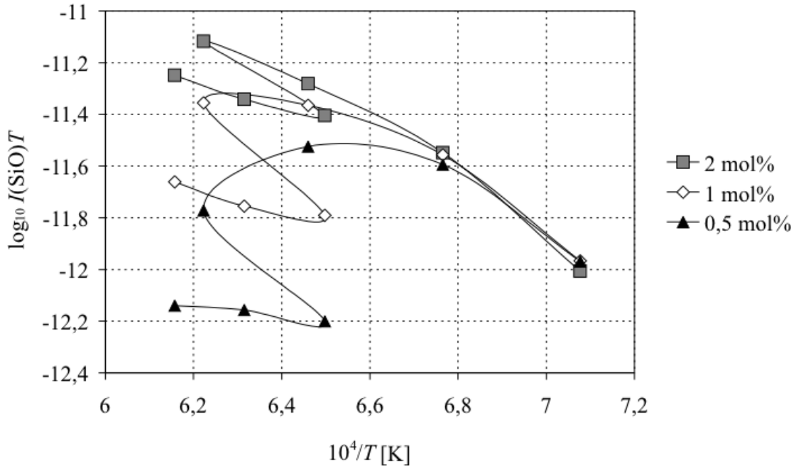
Figure 3.33: Evolution of the decimal logarithm of I(\text{SiO}) \cdot T for SiC-SiO 2 mixtures with 2, 1 and 0,5 mol% SiO 2 content as a function of the inverse of temperature.
