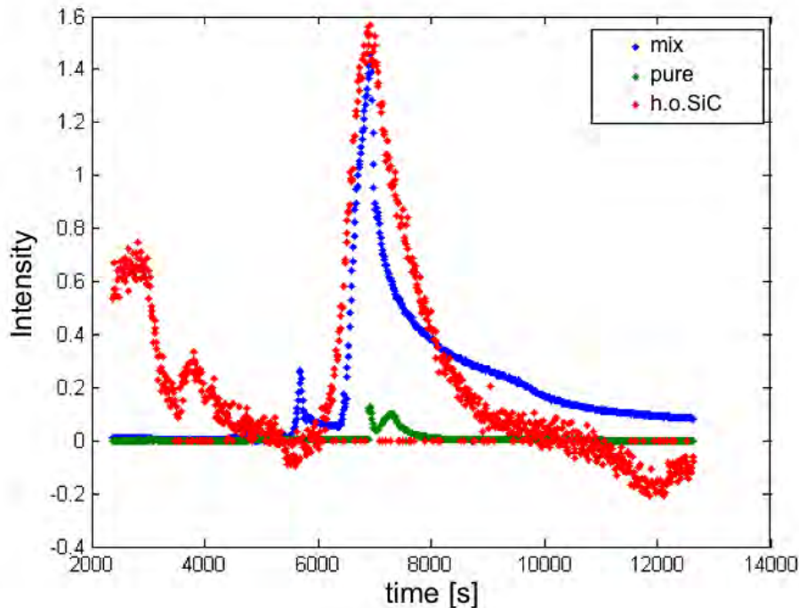
Figure 3.52: Intensities of CO ions during vaporization of SiC powder (green), SiC with 2 mol% SiO 2 mixture (blue) and oxidized bimodal SiC powder mixture (red) as functions of time. The intensities are corrected applying a sensitivity factor from nitrogen intensity.
