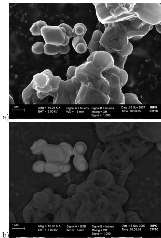
Figure 4.11: Necks formation and graphitization in sample of SiC with 2 mol% SiO 2 mixture after heating up to 1740 K for 2 hours in reactor coupled with mass spectrometer: a) SEM/FEG image; b) and back scattered electron detection imaging mode.
