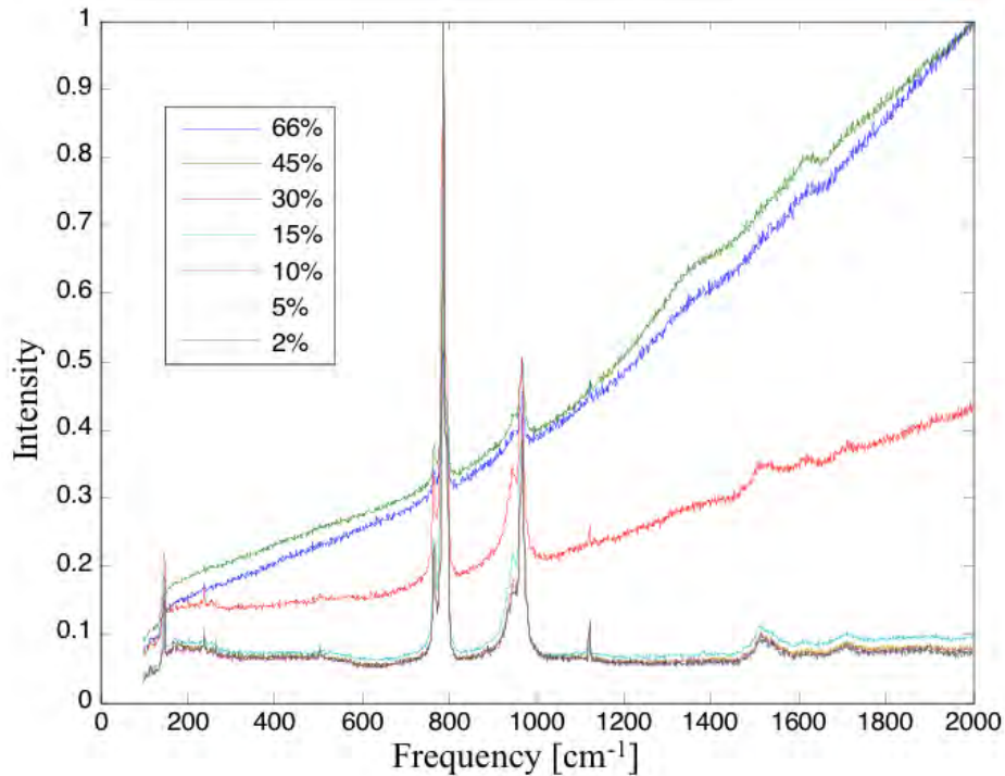
Figure 3.43: Raman spectra of SiC-SiO 2 mixtures with SiO 2 content from 2 to 66 mol% after SMHT experiment.
