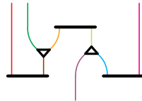
Figure 4-1: Examples of derivations in the calculus of structures (top row), their translation into the functorial calculus (middle row), and the flows associated with the latter (bottom row).
