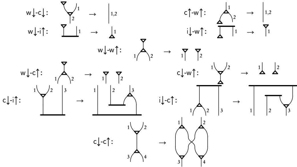
Figure 7-1: Atomic-flow reduction rules.
