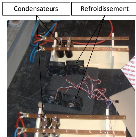
Figure C-5 : Charges capacitatives
