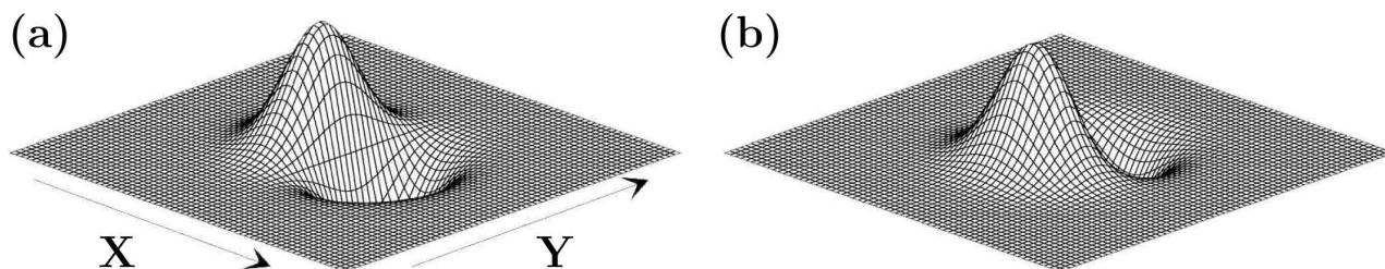
Figure B.1 3D plot of the derivative of the 2D Gaussian wavelet function used for the WTMM method, along the two axis X (a) and Y (b).
