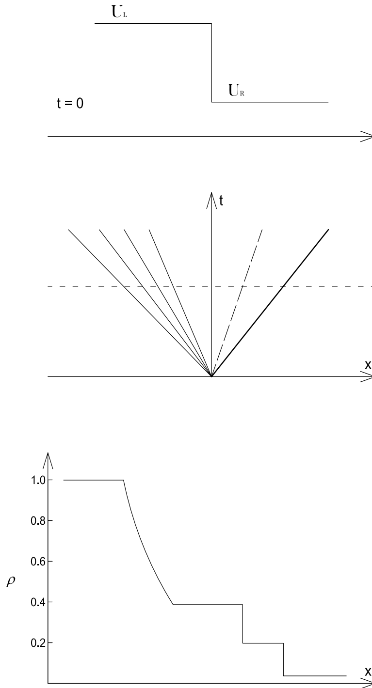
Figure 4.1: Top : Illustration of the initial data for the Riemann problem. At the initial time, the data consists of two constant states on the left and right cells, separated by a discontinuity at the cell interface (diaphragm). Middle : Solution of the Riemann problem for a shock tube made of 3 waves: expansion, contact discontinuity and shock waves. Bottom : corresponding density profile that reproduces the resulting 4 states.
