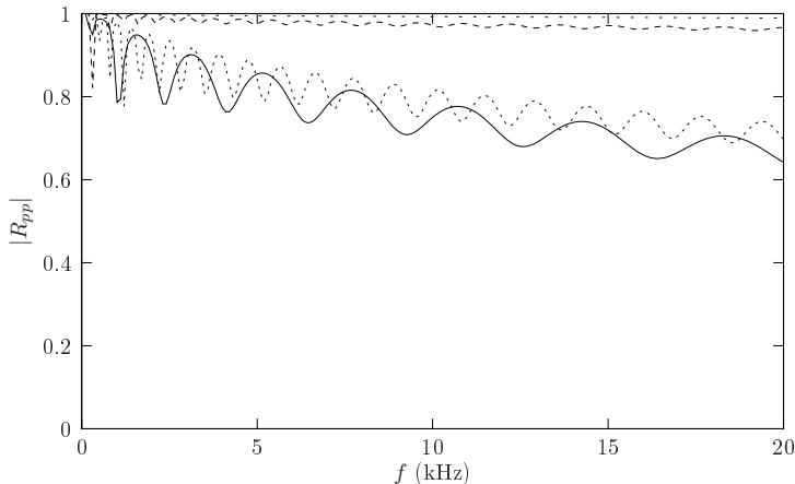
Figure 7.4: First term of the reflection matrix of a beam. \cdots , uniform beam covered with a 700 \mu\text{m} damping layer ( R_{20\text{kHz}}=0.985 ); ---- , beam with black hole profile without damping layer ( R_{20\text{kHz}}=0.97 ); - \cdot - \cdot - , beam with black hole profile covered with 10 \mu\text{m} of damping layer ( R_{20\text{kHz}}=0.7 ); — , beam with black hole profile covered with 700 \mu\text{m} of damping layer ( R_{20\text{kHz}}=0.62 ).
