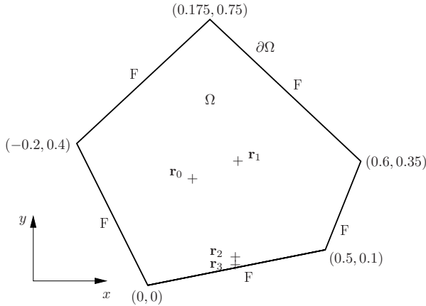
Figure 4.11: Polygonal plate for comparison of the proposed approach to FEM with free (F) boundaries. \mathbf{r}_0 = (0.125, 0.3) , source; \mathbf{r}_1 = (0.245778, 0.350778) , \mathbf{r}_2 = (0.245778, 0.073775) and \mathbf{r}_3 = (0.245778, 0.058386) , observation points. Coordinates are given in meters.
