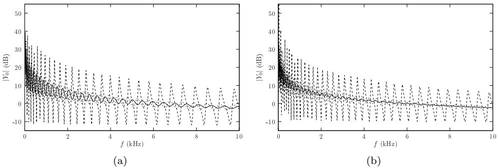
Figure 8.5: Driving-point mobilities for different temperature gradients. (a) Uniform beam, (b) beam with power-law thickness profile. \cdots\cdots , no thermal load; -\cdot-\cdot- , temperature profile (i) of Fig. 8.3; — , temperature profile (iii) of Fig. 8.3.
