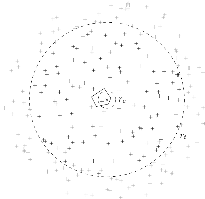
Figure 2.7: Example of image source cloud truncation for AISM. —, plate boundaries; ----, characteristic and truncation circles of radii r_c and r_t centered on the receiver; +, sources taken into account for AISM; +, ignored image sources.
