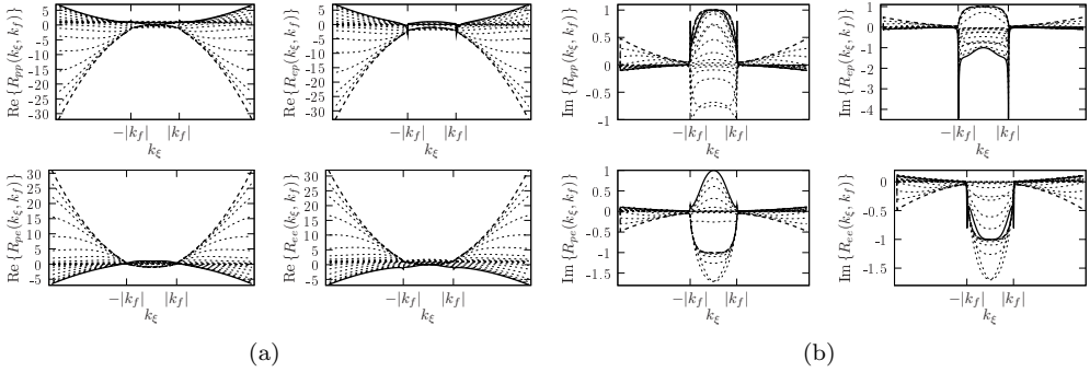
Figure 3.10: Reflection matrix of a stiffener edge with translational and rotational stiffnesses k_t and k_r arbitrarily varying from zero to infinity. (a) Real part, (b) Imaginary part. —, k_t = 0 and k_r = 0 (free edge); ----, k_t = \infty and k_r = \infty (clamped edge); ·····, intermediary states.
