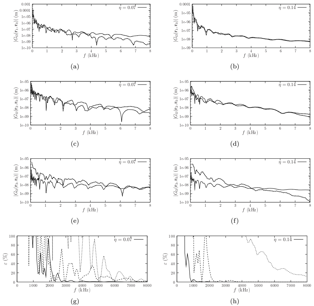
Figure 4.12: Modulus of the Green's function of the polygonal plate as a function of frequency computed by the proposed method ( \cdots\cdots\cdots ) and by FEM (—), for \eta = 0.07 (left column) and \eta = 0.14 (right column), at points (a,b) r_1 , (c,d) r_2 and (e,f) r_3 . (h,g) Error at points: —, r_1 ; - - - - -, r_2 ; \cdots\cdots\cdots , r_3 .
