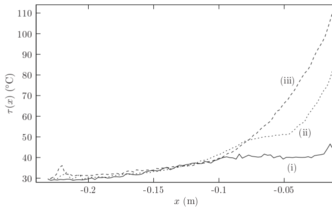
Figure 8.3: Measured temperature gradients on a uniform beam. Temperature at the bottom of the beam: —, 40.5 °C; ·····, 90.3 °C; -----, 114 °C.
