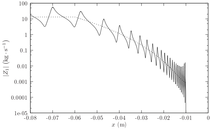
Figure 7.3: First term of the impedance matrix of a beam. —, beam with black hole profile covered with a 10 \mu\text{m} damping layer; \cdots\cdots , reference beam having a reflection matrix equal to zero.
