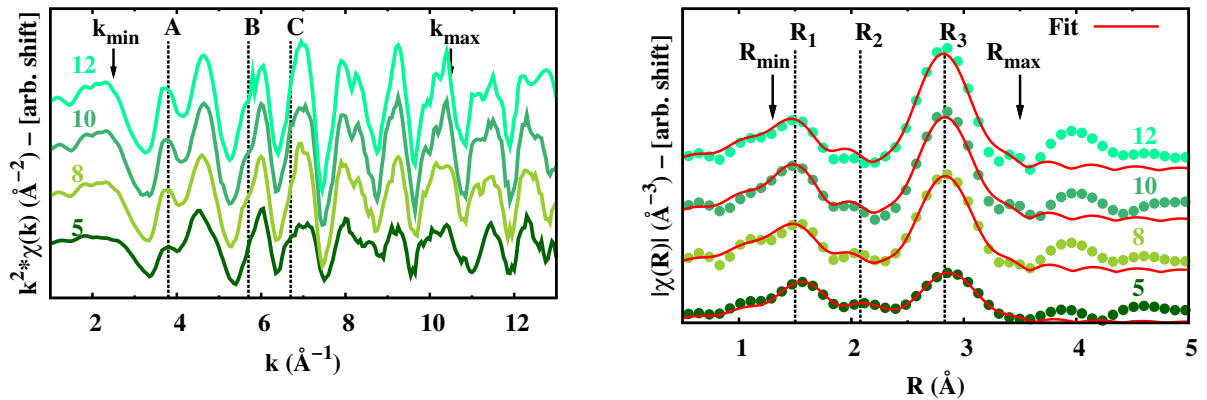
(a) k^2 -weighted EXAFS signals (sccm, labels on spectra); k_{min} and k_{max} delimit the Fourier-transformed part of the spectrum used in the fit.
