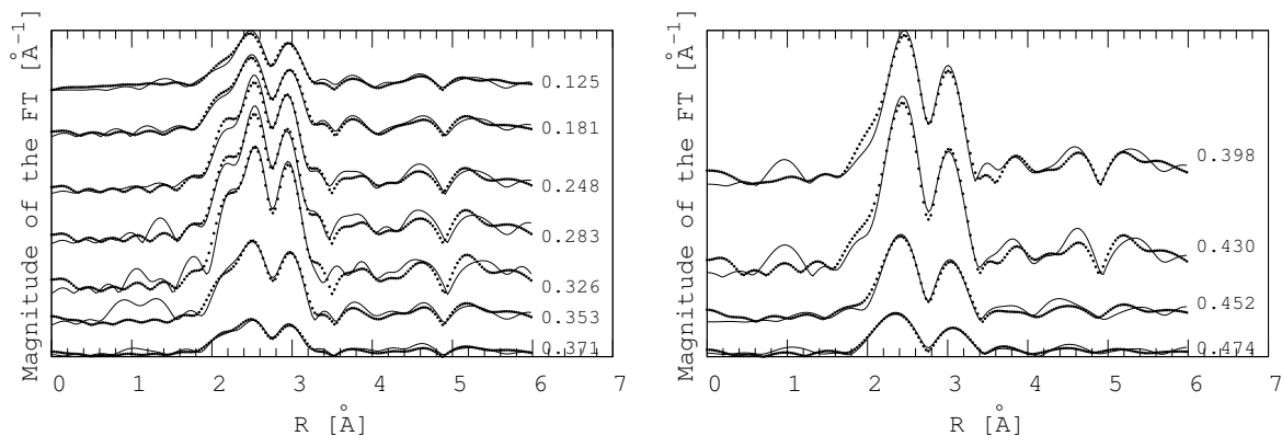
Figure B.6: Moduli of the Fourier Transforms of the \chi_{\Re}(k) at different grazing angles (continuous line) with the corresponding best fit curves (dots). The refined values of the grazing angles are displayed on the right side (in deg.).
