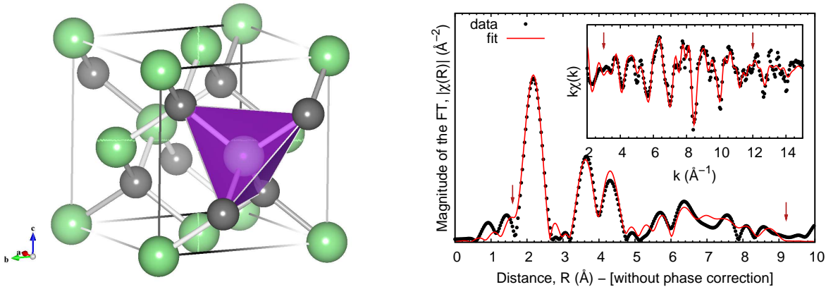
(a) Ball and stick model: Mn (violet), Ga (green), As (gray); the nearest neighbors distances are highlighted.
