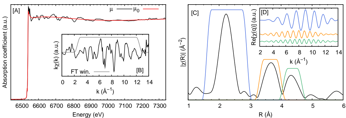
Figure 2.7: Example of data processing for Zn_{0.9}Mn_{0.1}Se fluorescence spectrum at Mn K-edge: the background ( \mu_0 ) is removed [A] to obtain the EXAFS spectrum [B]. Consequently it is Fourier-filtered to obtain a pseudo radial distribution function [C] whose peaks can be back-filtered to extract their contribution in the EXAFS signal [D]. Hanning windows are used for the Fourier transforms and, for convenience, are scaled in the plot.
