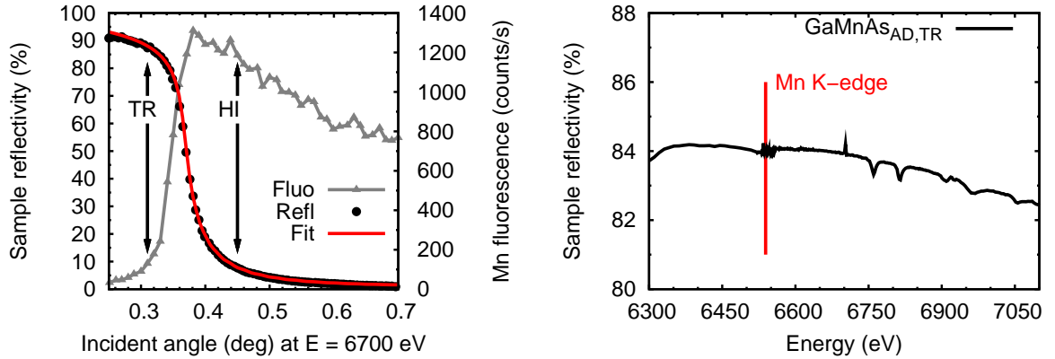
(a) Reflectivity with relative fit ( \rho_{\text{exp}} = 5.157\ \text{g/cm}^3 ) and fluorescence yield as a function of the incident angle.
