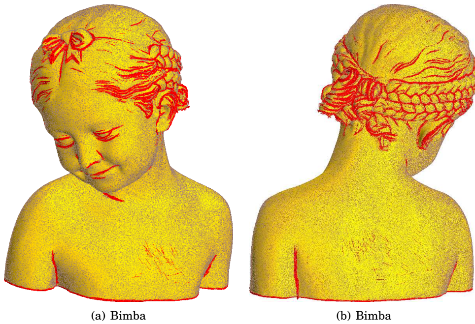
Figure III.13 – Detected features in the Bimba model
