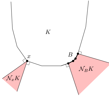
Figure IV.5 – Normal cones of a point x and a subset B of the convex hull K .
