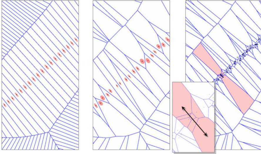
Figure III.2 – Voronoi-based normal estimation. In the second picture, one can see the angle defect in the normals estimated using the pole method, even if the points have been only moderately perturbed. The third picture shows clamped Voronoi cells under stronger noise. (courtesy of P. Alliez et al. )
