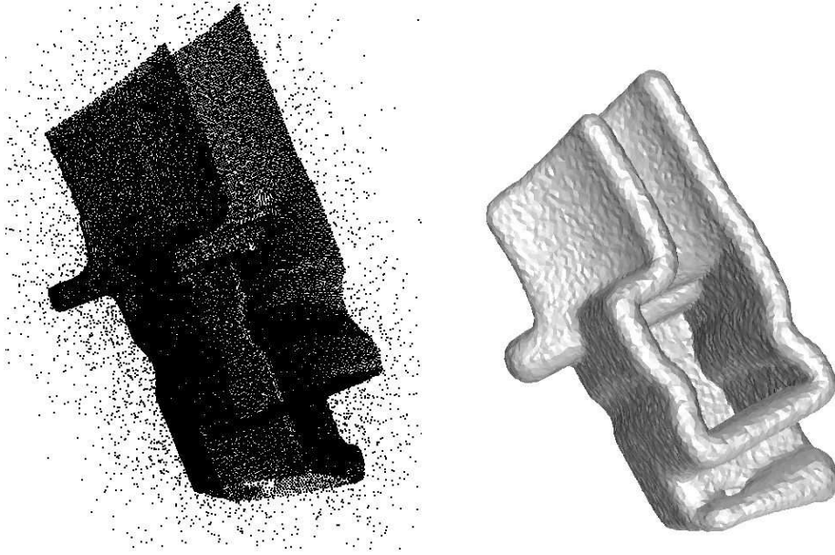
Figure IV.2 – On the left, a point cloud sampled on a mechanical part (blade) to which 10% of outliers have been added — the outliers are uniformly distributed in a box enclosing the original point cloud. On the right, the reconstruction of an isosurface of the distance function d_{\mu_C, m_0} to the uniform probability measure on this point cloud (obtained by using the CGAL Surface Mesher).
