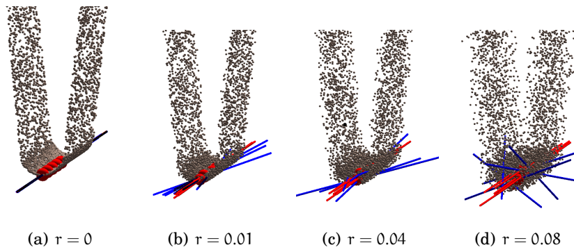
Figure III.10 – Principal curvature directions computed with our method (in red) are stable under noise. Directions computed by jet-fitting (in blue), are unreliable, especially when points from separate parts of the shape begin to mix ( d ).
