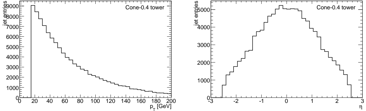
(a) jet p_T(ttH) distribution
