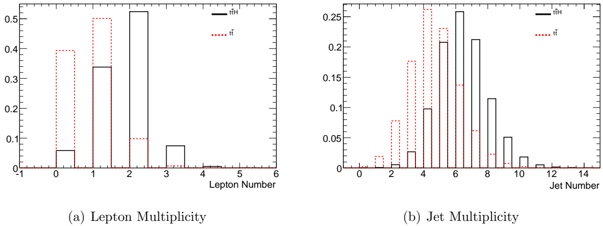
FIGURE 3.11: Lepton Multiplicity and Jet Multiplicity
