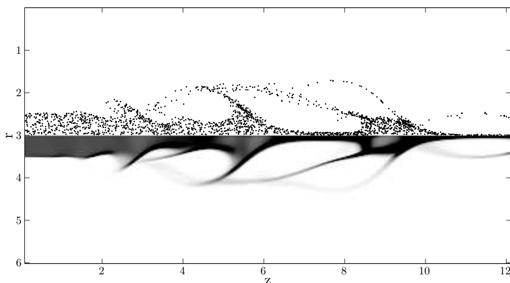
Figure 9.5 – Non evaporating polydisperse spray, high inertia droplets , Stokes 0.71 to 4.45 corresponding to diameters d = 60 \mu\text{m} to d = 150 \mu\text{m} , at dimensionless time t=15 : (top) Lagrangian particle positions with 40000 particles over gas vorticity, (bottom) Eulerian number density with a 400 \times 100 \times 5 grid.
