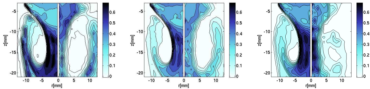
Figure 5.4 – Comparison between IPI experimental measurements (right half) and numerical simulation (left half) for total droplet concentration at phase \pi in droplet/mm 3 . From left to right: decane (non evaporating reference liquid), methanol and heptane (evaporating liquids). Experimental results are presented through an averaged field obtained from 120 instantaneous phase-locked samples with a reduced field of view of 27 \times 20 mm 2 . Numerical simulation was obtained on a 400 \times 400 grid.
