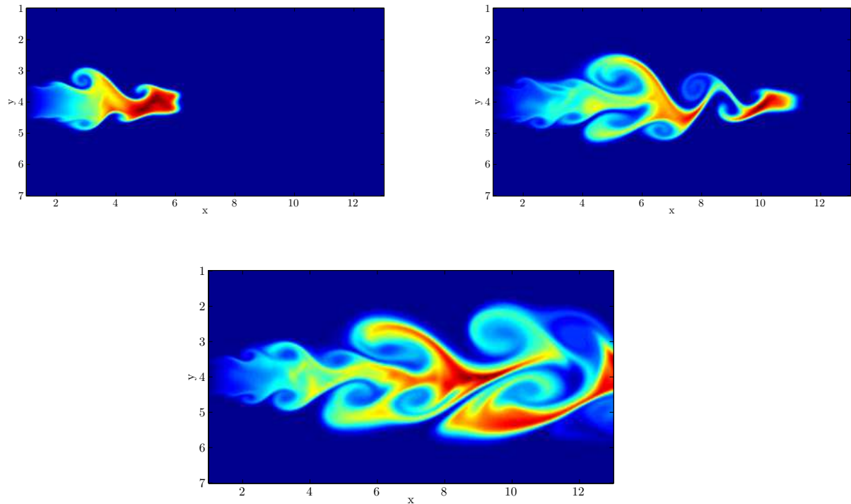
Figure 10.6 – Gaseous fuel mass fraction obtained from multi-fluid computed spray evaporation, on a 400 \times 200 \times 10 grid. Three times are plotted: (top-left) t = 5 , (top-right) t = 10 , (bottom) t = 20 .
