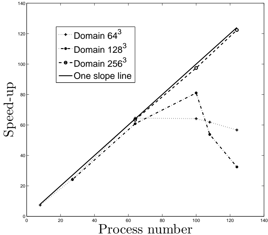
Figure 7.8 – Speed-up evolution with the number of parallel processes used, for three spatial domain discretization: 64^3 (dotted line), 128^3 (dashdot line) and 256^3 (dashed line). A one slope line is also plotted (solid line). The curve obtained for each discretization corresponds to Amdahl vision. A saturation occurs, except for the 256^3 where the number of processes leading to saturation is not reached.
