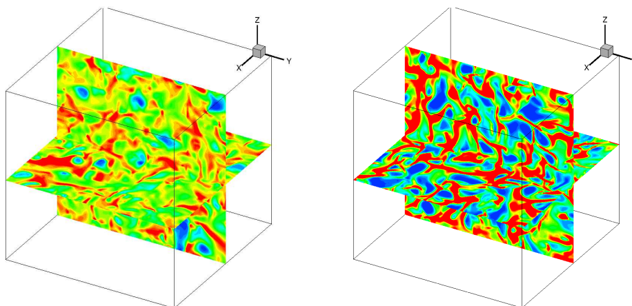
Figure 11.3 – Eulerian spray number density obtained with the multi-fluid method on a 128^3 Cartesian grid. Slice planes inside the domain ( x = x_{max}/2 , z = z_{max}/2 ) for two Stokes number: (left) St = 0.17 , (right) St = 1.05 .
