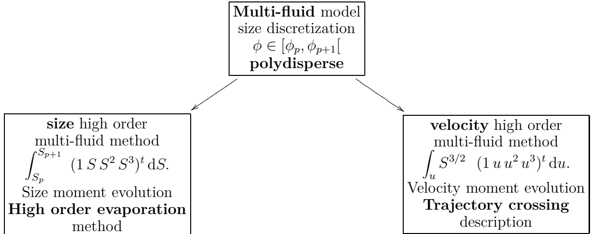
Figure 2.6 – Size/Velocity high order multi-fluid method. These methods describe accurately droplet evaporation and trajectory crossings, respectively.
