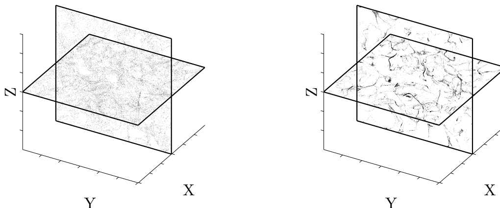
Figure 11.5 – Lagrangian droplet positions obtained by a DPS with 2150000 droplets. Slice planes inside the domain ( x = x_{max}/2 , z = z_{max}/2 ) for two Stokes number: (left) St = 0.17 , (right) St = 1.05 .
