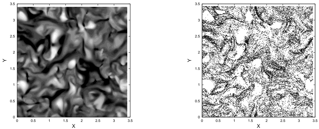
Figure 11.9 – Gas vorticity square norm in the x - y plane at z = z_{max}/2 . The gaseous turbulence has reached its stationary state.
