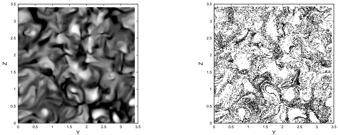
Figure 11.7 – Eulerian Lagrangian comparisons in the y - z plane at x = x_{max}/2 for low inertia droplets, St = 0.17 : (left) Eulerian multi-fluid number density, (right) Lagrangian droplet positions.
