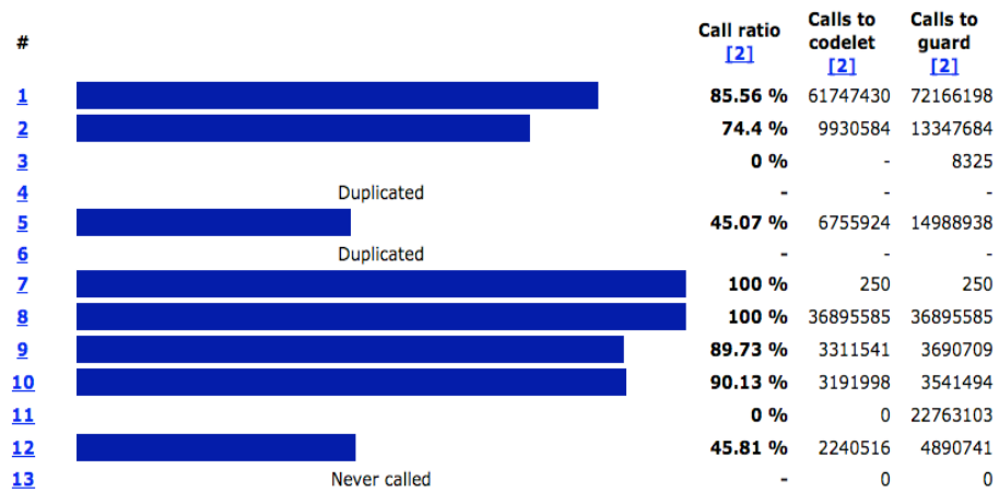
Specialized codelets call ratio
