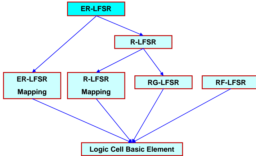
Figure 34: LFSRs Combinés
