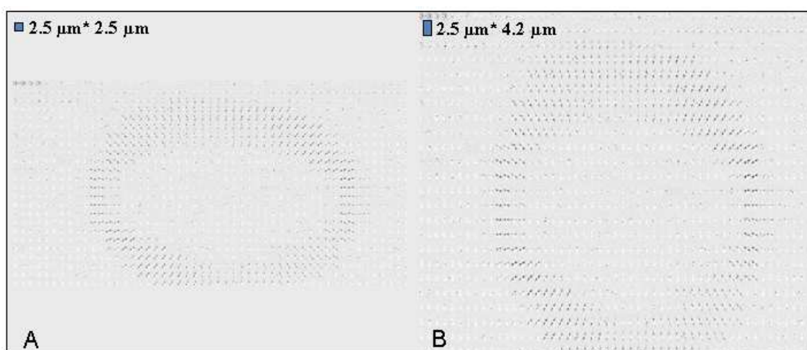
Figure 6.20 A: Composite image of SAXS patterns collected with a raster-mesh of 2.5 \mu\text{m} * 2.5 \mu\text{m} . The area of each “pixel” is limited to the Q -range of the refraction streak. The microdrop shape, revealed by the water/air interface refraction streaks, is distorted into an ellipse due to the change in microdrop speed with change of pressure in the reservoir. (see section 5.2.6) B: image corrected for the speed change. The apparent vertical step is 4.2 \mu\text{m} .
