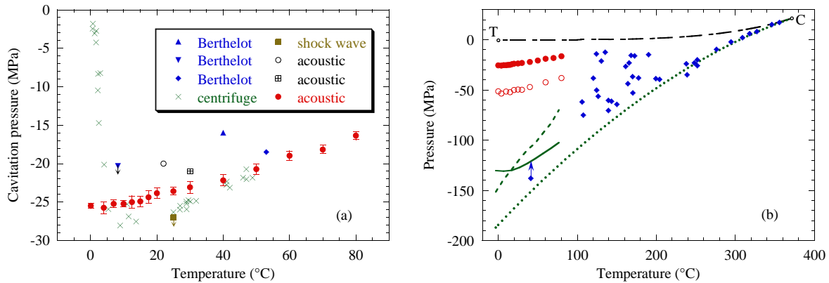
Figure 3.2: (a) Cavitation pressure versus temperature for different experiments: the corresponding method and reference are given in the legend. Only the experiments with the most negative cavitation pressures were selected, except the inclusion work, for sake of clarity. An arrow means that cavitation was not observed. The error bars on the filled circles represent the uncertainty on the pressure calibration. (b) Cavitation pressure versus temperature, calculated with CNT [C11] (dotted line), or using DFT with Speedy’s EoS [30] (solid line) or with the EoS from a recent molecular dynamics simulation [61] (short-dashed line). The parameters used are V = (10 \mu\text{m})^3 , \tau = 1 \text{ s} , and \Gamma_0 from Eq. 2.6. The dash-dotted line shows the saturated vapor pressure from the triple point (T) to the critical point (C). Some experimental results are also shown. Filled diamonds correspond to experiments on mineral inclusions [49]; the arrow shows a correction to the pressure estimate to account for the quartz compressibility. Filled circles show our data obtained with an acoustic method, and empty circles the spinodal we once proposed to interpret them [C29].
