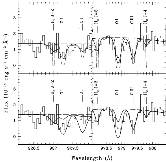
Fig. 2. Sample of OI lines detected at the redshift of IZw 18 ( 750 \text{ km s}^{-1} ). The \text{H}_2 lines are from the Milky Way. The C III line is at a redshift of 720 \text{ km s}^{-1} . The histogram shows the data. The upper panels show the final fit (thick line) together with the theoretical spectrum before convolution with the instrumental line spread function (thin dot-dashed line). The OI line at 927.7 \text{ \AA} is not saturated, the line at 927.2 \text{ \AA} is barely saturated, while the one at 978.9 \text{ \AA} is saturated. The bottom panels show the same data with the theoretical profiles using an OI column density reduced and increased by a factor of 10 (i.e. \log N(\text{OI}) = 15.6 and 17.6 , respectively). Such column densities are clearly excluded. With \log N(\text{OI}) = 15.6 , the line at 927.2 \text{ \AA} would not be detectable, and the line at 978.9 \text{ \AA} would be much fainter than observed. With \log N(\text{OI}) = 17.6 , the line at 927.7 \text{ \AA} would be much deeper than observed.
