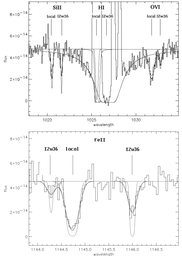
Fig. 1. H I and Fe II lines in IZw 36. The flux is in \text{erg s}^{-1} \text{cm}^{-2} \text{\AA}^{-1} and the observed wavelength in \text{\AA} . The data (histogram) are binned by a factor 3 for display purposes. The thin line represents the line profile before the convolution with the total line broadening represented by \sigma_{\text{tot}} in Sect. 3.1 and the thick line is the convolved profile. For each of the spectral windows, we used the two observations and all the available FUSE detection channels (Sect. 2) to perform the fit. Here we show the spectrum of segment LiF1 for the upper plot and of segment LiF2 for the lower plot. a) (upper) Plot of the Ly\beta line. The center of the line is blended with terrestrial airglow emission lines. Atomic hydrogen in the Milky Way is invisible because of its low column density \sim 10^{19} \text{ cm}^{-2} (estimated from Heiles 1975). The Si II \lambda 1020.70 lines and O VI \lambda 1031.93 lines from the Milky Way and IZw 36 are also visible in this spectrum. b) (lower) Plot of the strong Fe II \lambda 1144.94 line.
