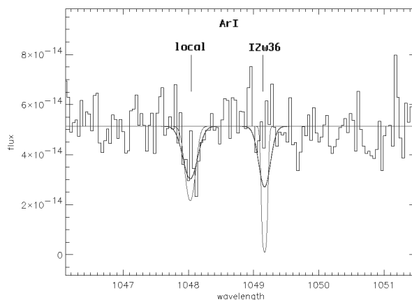
Fig. 3. Lack of argon in IZw 36. See Fig. 1 for a description of the plot. Data are binned by a factor 2 for display purposes. The line plotted at the redshift of IZw 36 is for \log N(\text{Ar I}) = 14.0 and b = 12.0 \text{ km s}^{-1} .
