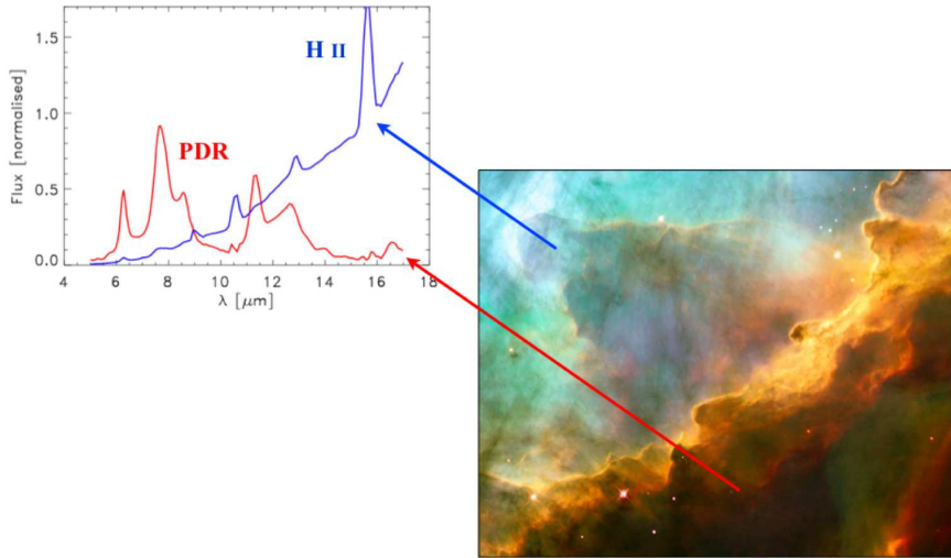
Figure 1.14: Right: Optical image of the SW part of the star-forming region M17 taken with the WFPC2 instrument on the Hubble Space Telescope. The newly-formed, ionizing stars are located in the direction of the upper left corner of the picture. The image is a composite of three filters that capture three strong emission lines observed in H II regions: red – N II; green – H \alpha ; blue – O III. Image credit: ESA, NASA, and J. Hester (Arizona State University). Left: Mid-infrared spectrum of the H II region (in blue) and of the photo-dissociation region (in red) extracted from the ISO/ISOCAM observations of Cesarsky et al. (1996) by Madden et al. (2006). These spectra highlight the difference in physical conditions inside H II regions and PDRs, which translate in different dust emission properties. The spectrum of the H II region is dominated by a rising continuum from very hot small grains, strong emission lines from ionized gas (e.g., the strong [Ne III] line at 15.8 \mu\text{m} ), and no emission by PAHs molecules, which are destroyed by the intense ultraviolet radiation field from hot stars; the spectrum from the PDR is dominated by the emission features from PAHs molecules, which are shielded from the extreme ultraviolet radiation and can survive (more details about the emission by dust will be presented in Section 1.4.3.4).
