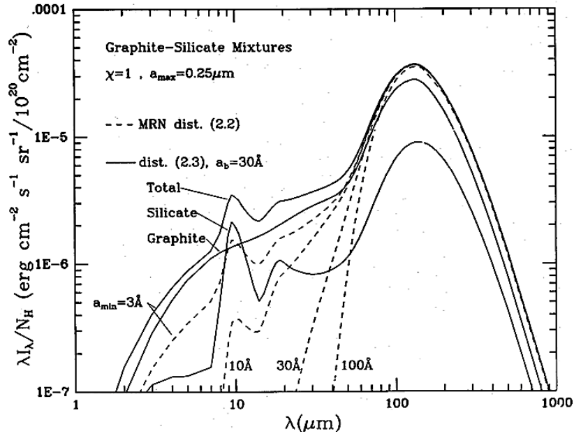
Figure 1.20: Emission spectra of mixtures of graphite and silicate grains with various size distributions, heated by the average interstellar radiation field. Curves are labelled by a_{\min} , the lower cutoff on the size distribution; an upper cutoff a_{\max} = 0.25 \mu\text{m} is taken in all cases. The dashed lines are for a classical Mathis, Rumpl & Nordsieck (1977) size distribution, whereas the plain lines show a size distribution with a higher relative quantity of small particles. Figure taken from Draine & Anderson (1985).
