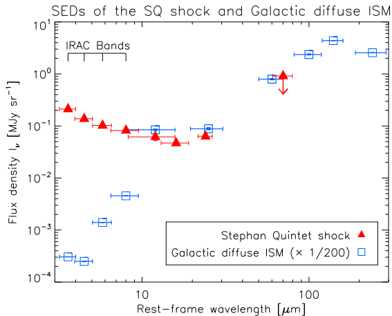
Fig. 2. The SED of the dust emission from the SQ shock seen by Spitzer (table 1), compared with that of the Galactic diffuse emission observed with Spitzer IRAC , IRAS and DIRBE towards the line-of-sight centered on the Galactic coordinates (28.6, +0.8). The contribution of the gas lines is subtracted. The Galactic SED is scaled down by a factor 200. Between 3 – 8 \mu\text{m} , the SQ flux is much brighter because of the stellar continuum component. Horizontal bars indicate the filters bandwidths.
