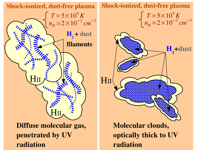
Fig. 6. Sketch of the two limiting physical states of the multiphase molecular gas we are considering in the framework of our modeling of dust emission. (Left) Dust is associated with diffuse molecular gas that is broken into fragments, filaments or sheets, penetrated by UV radiation. (Right) The dusty molecular gas is in clouds that are optically thick to UV light.
