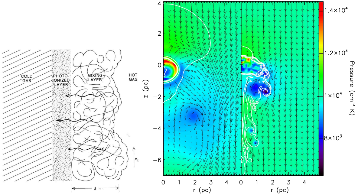
Figure 4.12: Left: Schematic description of a turbulent mixing layer from Slavin et al. (1993). Right: Numerical simulations of a CNM cloud embedded in a hot plasma stream (J. Slavin, private communication). The colors indicate the gas pressure, and the arrows the velocity field. In the left panel, heat conduction is taken into account, whereas in the right panel not. The cloud with thermal conduction ( left ) is much less disrupted than the cloud with conduction turned off ( right ). The hot gas has a speed of 50 \text{ km s}^{-1} relative to the cloud and a temperature 10^6 \text{ K} . The initial cloud density is n_{\text{H}} = 0.6 \text{ cm}^{-3} and its radius 1 pc. The cloud to hot gas density contrast is \chi = 125 . The ambient pressure is 10^4 \text{ K cm}^{-3} . No cooling processes are included in these simulations.
