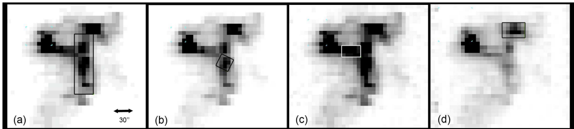
FIG. 7.— We show here the rectangular sub-regions extracted from the main components of the SQ shock system overlaid on the H 2 0-0 S(1) line emission. a) The Main Shock region centered on 22 h 35 m 59.6 s , +33°58′05.7″. b) A region in the main shock centered on 22 h 35 m 59.97 s , +33°58′23.3″ and chosen to have limited contamination from star forming regions in SQ. c) Extraction of the H 2 “bridge” feature centered on 22 h 36 m 0.14 s , +33°58′23.3″. d) An extraction of the SQ-A star forming region centered on 22 h 35 m 58.85 s , +33°58′50.4″.
