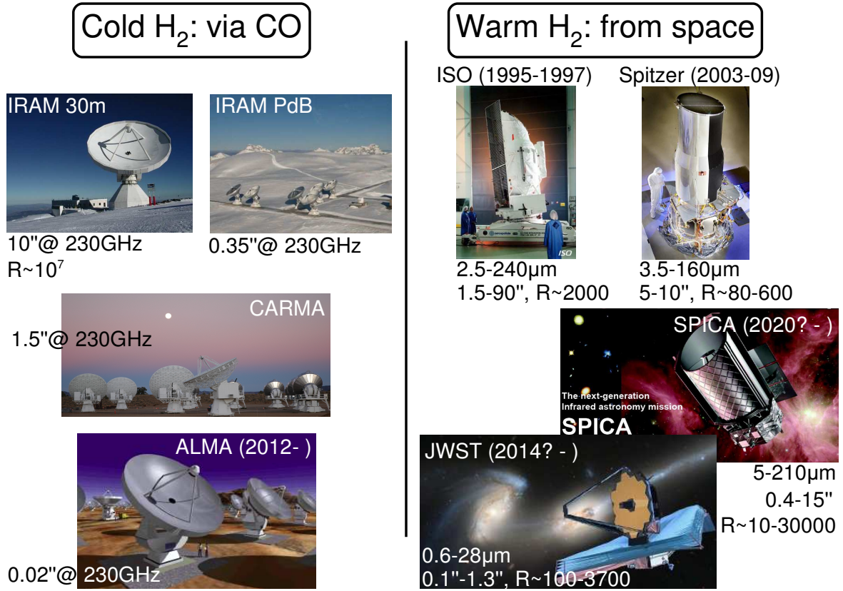
Figure 3.9: Cold and warm molecular gas are observed with two different kinds of observatories. Cold molecular gas is essentially derived from CO ground-based observations with single-dish radiotelescopes or interferometers. On the other hand, the IR emission from warm H_2 must be observed from space. This figure shows a few examples (past, present and future) of these observatories, with their basic characteristics (wavelength coverage, spatial and spectral resolution).
