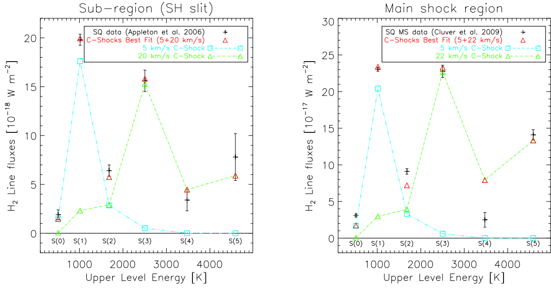
Figure 6.9: Fit of the Stephan’s Quintet H 2 spectral energy distribution with 2 shocks at fixed density n_{\text{H}} = 10^4 \text{ cm}^{-3} . Left: data from Appleton et al. (2006) , extracted within the IRS SH slit aperture in the center of the ridge. Right: data from Cluver et al. (2009) ( paper II ) for the main shock region. The 2 shock components account for comparable fractions of the total H 2 luminosity but the less energetic component accounts for most of the warm H 2 mass (see table 6.3 and 6.4 ).
