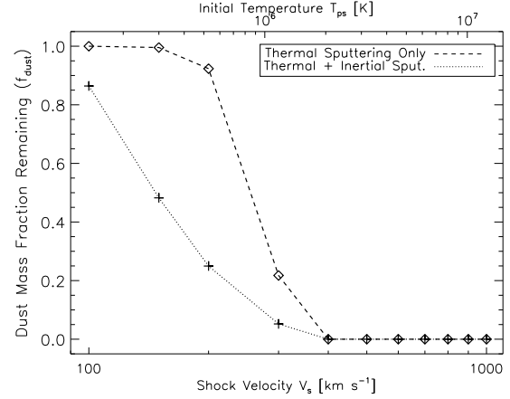
Fig. A.1. Dust mass fraction as a function of the initial (postshock) temperature, after isobaric cooling to 10^4 K. The pressure is fixed to P_{\text{ps}}/k_{\text{B}} = 2.3 \times 10^5 [cm -3 K]. The dotted line shows the result of the model which includes both inertial and thermal sputtering. As a comparison, the dashed line only shows the effect of thermal sputtering.
