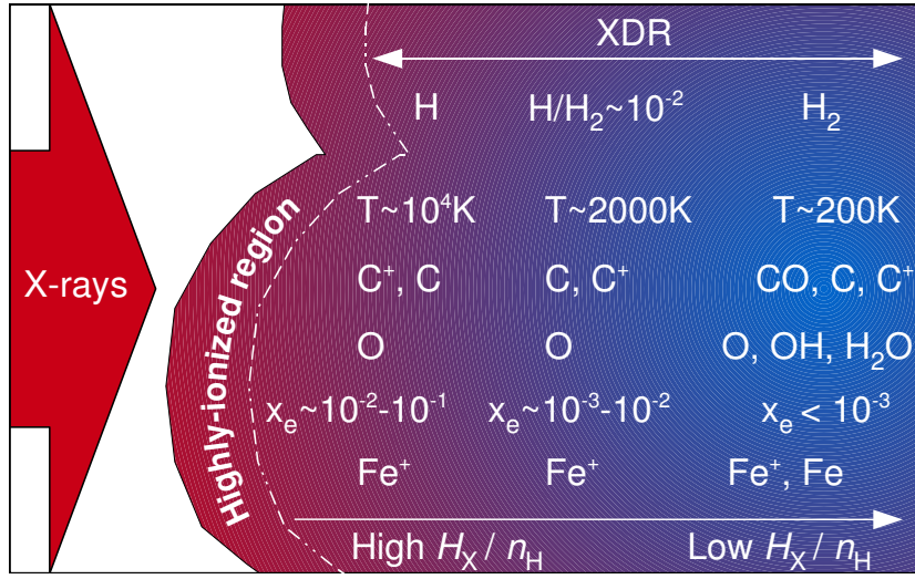
Figure 3.7: Schematic structure of an X-ray dissociation region (XDR), where an X-ray flux ( arrow on the left ) illuminates a molecular cloud ( on the right ). As we penetrate into the XDR, we indicate the approximate temperature, chemical composition and ionization fraction x_e as a function of the ratio of the local X-ray energy deposition rate per particle, H_X , to the total hydrogen density n_H .
