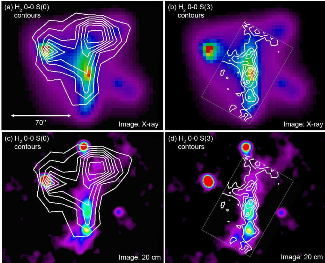
FIG. 3.— X-ray image from XMM-Newton (Trinchieri et al. 2005) in the 1.5–2.5 keV band with (a) H 2 S(0) contours and (b) H 2 S(3) contours overlaid. Also shown are 1.4 GHz radio continuum images from the VLA (Xu et al. 2003) with (c) H 2 S(0) contours and (d) H 2 S(3) contours overlaid. Contours levels are as in Fig 2.
