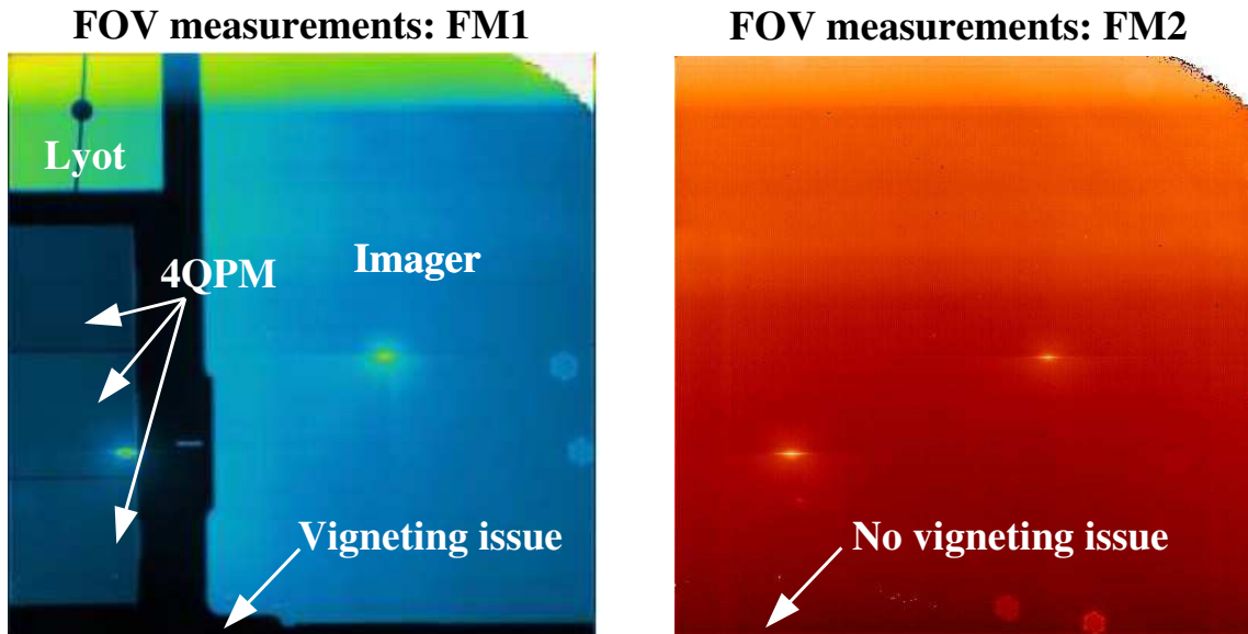
Figure 11.18: Comparison of the Field of View measurement between the two Flight model test campaigns, FM1 and FM2. On the left plot (FM1), the complete MIRIM focal plane is mounted, with the coronagraph masks and the LRS slit (see Fig. 10.10 for the pattern of the focal plane). The vignetting issue is clearly seen at the bottom of the image. The black stripe at the bottom shows that a significant fraction of the field of view is lost. On the right plot (FM2), the vignetting issue has been corrected (no black stripe anymore). Note that for the FM2 tests, the coronagraph masks are not mounted.
