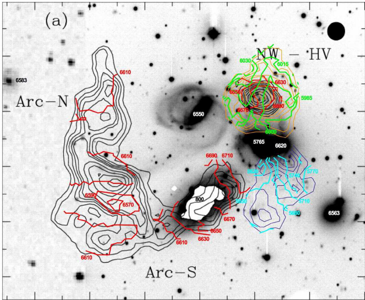
Figure 6.7: The of H I column density contours and first-order moment of the radial velocity (lines and numbers in \text{km s}^{-1} ) for low (cyan and blue), intermediate (green and orange) and high (red and black) velocity ranges. The galaxies velocities are from Sulentic et al. (2001) . This image is taken from Renaud (2007) .
