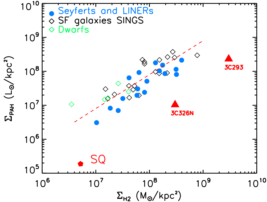
Figure 7.6: Star-formation efficiency (assumed to be traced by the surface luminosity of the PAH emission) as a function of mass of cold \text{H}_2 , derived from the CO(1-0) line intensity. The hatched line shows the relationship obtained for the SINGS sample, where empty diamonds and filled dots mark dwarf galaxies, star-forming galaxies, and AGN. The SINGS data is from Roussel et al. (2007). The filled pentagon shows the center of the SQ shock. For comparison, the filled triangles mark the \text{H}_2 -luminous radio galaxies 3C326 N and 3C293.
