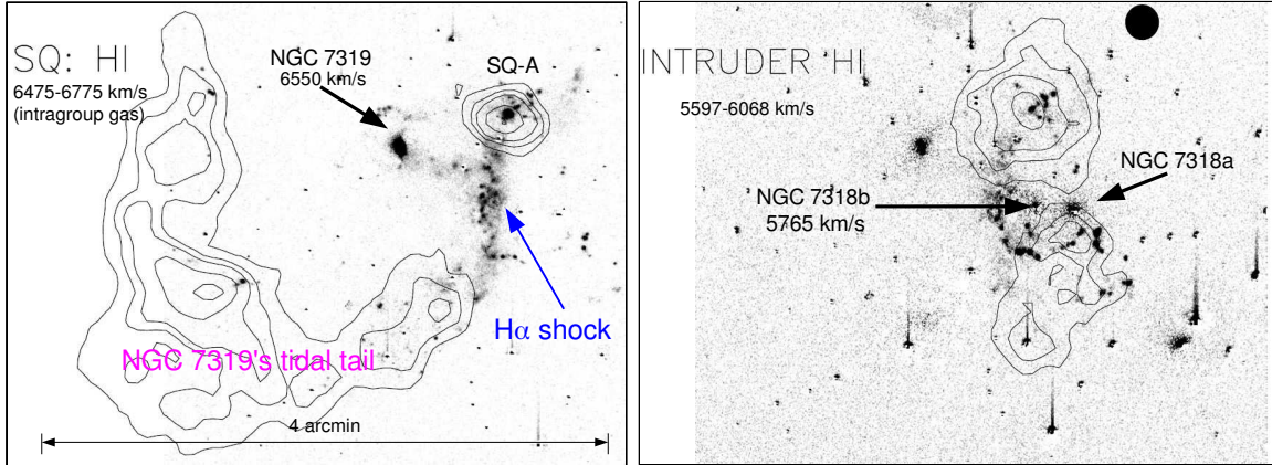
Figure 6.6: HI 21 cm radio contours superposed on H\alpha interference filter images. Left: HI contours for velocities in the SQ range 6475 - 6775 \text{ km s}^{-1} . Right: HI contours for velocities in the new intruder range ( 5597 - 6068 \text{ km s}^{-1} ). HI contours levels correspond to [0.526, 1.58, 2.63, 5.26, 7.89] \times 10^{20} \text{ cm}^{-2} with last contour shown only in the left panel. Adapted from Sulentic et al. (2001) .
