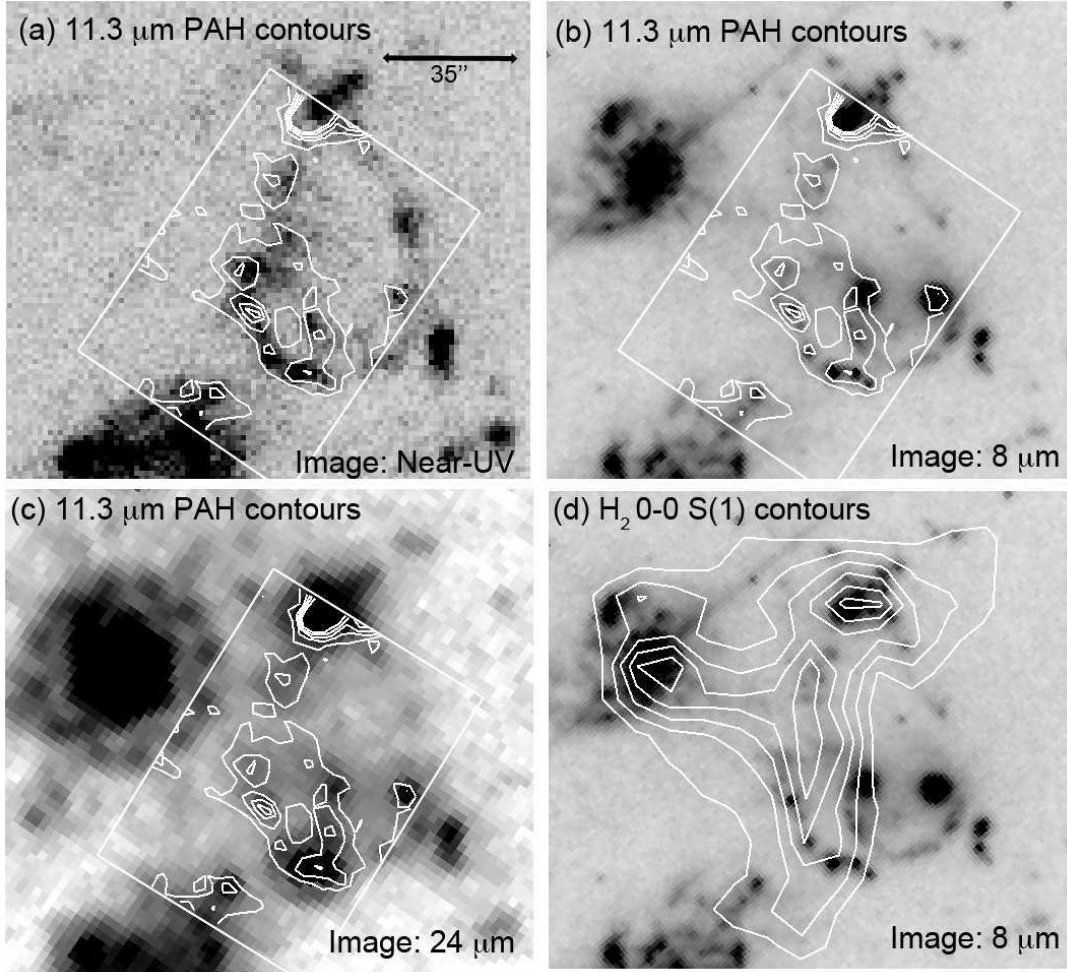
FIG. 6.— Dust as tracers of star formation. This shows 11.3μm PAH contours overlaid on (a) the Near-UV, (b) an 8μm image and (c) a 24μm image. By comparison the H 2 0-0 S(1) contours show little correlation with the 8μm image (as shown in d). Contour levels are as follows (in units of MJy/sr): (a), (b) and (c) are 0.2, 0.35, 0.5, 0.65, 0.8. Contour levels for (d) are as in Fig. 2b.
