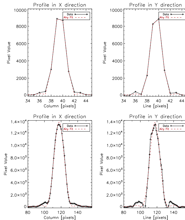
Figure 11.15: Low (2 upper plots ) and super-resolution (2 bottom plots) PSF profiles in the X and Y directions. The low-resolution PSF correspond to one single position MIRIM image. For the super-resolution PSF, the sampling is increased by a factor of 7. Red dashed lines are the results of the Airy fits.
