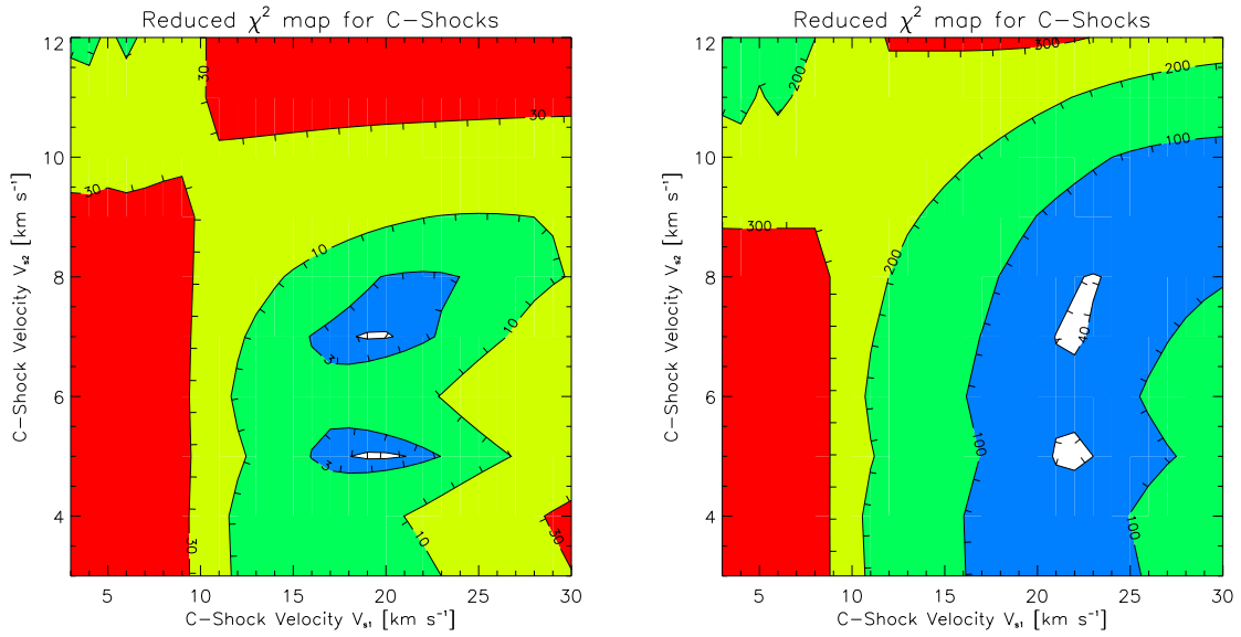
Figure 6.10: Reduced \chi^2 map for the fit of the Stephan’s Quintet H 2 spectral energy distribution with 2 shocks at fixed density n_{\text{H}} = 10^4 \text{ cm}^{-3} . Left: data from Appleton et al. (2006) , extracted within the IRS SH slit aperture in the center of the ridge. The \chi^2 contours are 1.5, 3, 10, 30. Right: data from Cluver et al. (2009) ( paper II ) for the main shock region. The \chi^2 contours are 40, 100, 200, 300.
