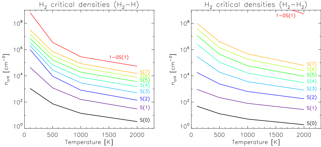
Figure 3.3: Critical densities, n_{\text{crit}} , for the S(0) to S(7) H 2 rotational lines, and the 1-0S(1) rovibrational line. The corresponding upper J levels are thermalized if the gas density is higher than n_{\text{crit}} . The collisional partner is H on the left plot and H 2 on the right . The critical densities are calculated at 100, 500, 1000 and 2000 K from Wrathmall et al. (2007).
