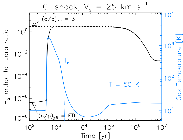
Figure 4.8: Evolution of the H 2 ortho-to-para ratio and temperature (in blue, labeled on the right) for a 25 km s -1 C-shock. Two initial values of the o/p ratio are shown: the Local Thermodynamical Equilibrium (LTE) value at 10 K ( 3.5 \times 10^{-7} ), and the high-temperature limit (3). The preshock medium is molecular, at a density n_{\text{H}} = 10^4 \text{ cm}^{-3} . The preshock magnetic strength is B = 100 \mu\text{G} , perpendicular to the direction of propagation of the shock.
