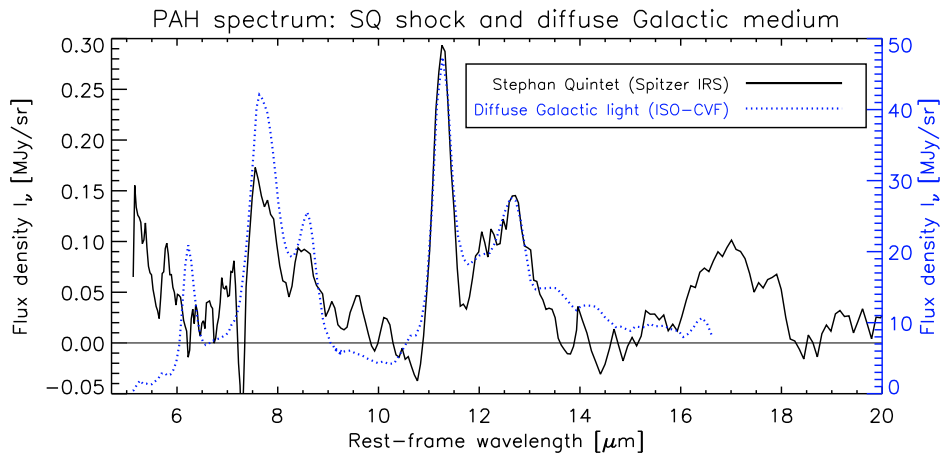
Fig. 4. Spitzer IRS PAH emission spectrum extracted in the center of the SQ ridge (black solid line), compared with the ISOCAM-CVF spectrum of the diffuse galactic medium (blue dashed line, with flux density labeled on the right). The IRS spectrum is smoothed to a resolution \mathcal{R} = \lambda/\delta\lambda = 24 \rightarrow 51 , comparable with the ISO-CVF resolution ( \mathcal{R} = 35 \rightarrow 45 ). Gas lines are removed in both spectra. Note that the flux scales are different for each spectrum (labels on the left for SQ, and on the left for the Galaxy).
