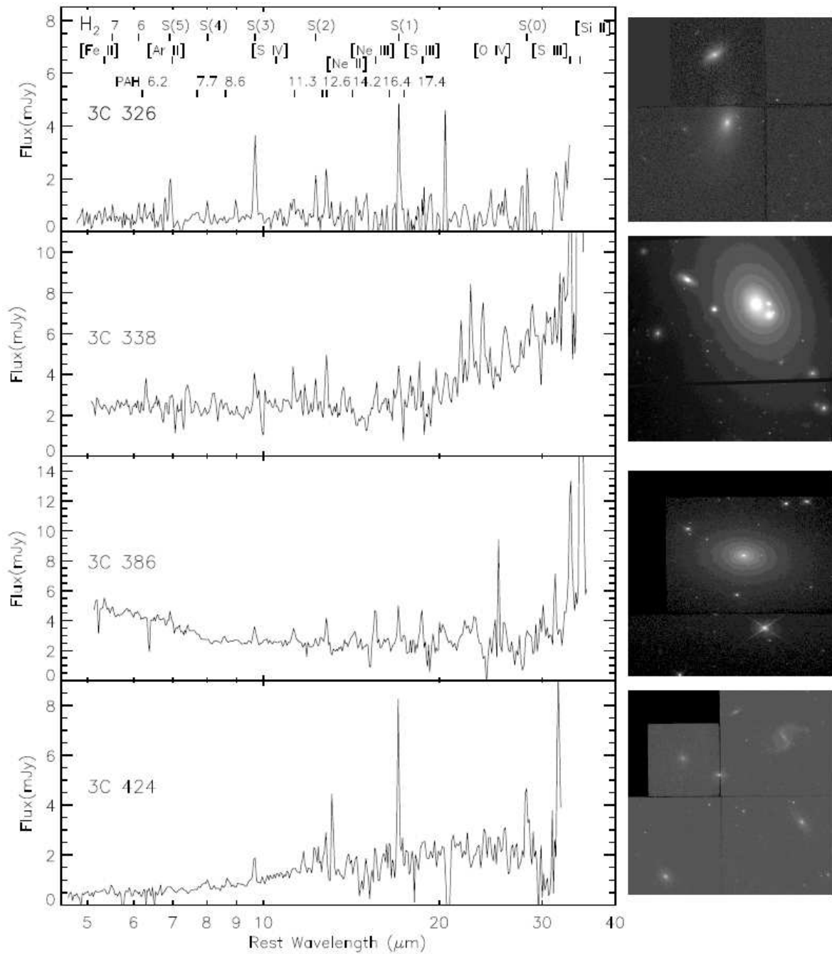
Figure 1.4: Examples of Spitzer IRS low-resolution spectra of MOHEGs (3C 326, 338, 386, 424). These sources show no silicate absorption and very weak PAH emission. On the right, we show HST WFC2 and ACS images. Taken from Ogle et al. (2009) .
