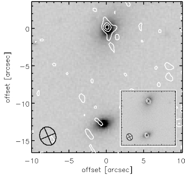
Fig. 1. Continuum-free CO(1-0) emission-line morphology of 3C326 N (white contours) superimposed on the SDSS R-band image of 3C326 N and 3C326 S. Contours are given for 3, 4, and 5 \sigma . The inset shows the same SDSS R-band with the line-free 3mm continuum morphology superimposed as white contours. We used the continuum morphologies to align the millimeter and optical data, assuming that the AGN reside in the nuclei of the galaxies. With this alignment, we find an offset of 0.7'' between the CO line emission and continuum (millimeter and optical) which, given the faintness of the line emission and much greater beam size, is not significant. The ellipse in the lower left corner shows the beam size and position angle in both images.
