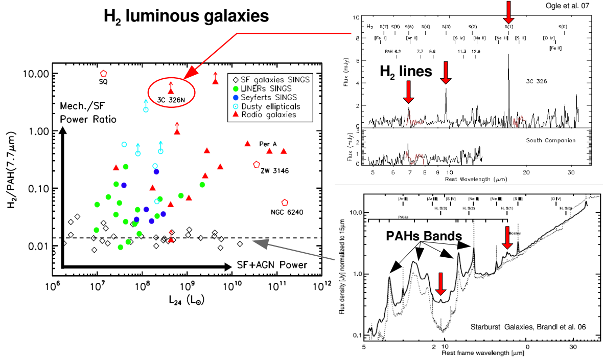
Figure 1.2: H_2 -luminous galaxies in one plot. Left: Ratio of H_2 rotational emission summed over the 0-0 S(0)–S(3) lines to 7.7\mu\text{m} PAH luminosity, as a function of the 24\mu\text{m} continuum luminosity. The ratio indicates the relative importance of mechanical heating and power by star formation. At all IR luminosities, the observations reveal galaxies with excess H_2 emission beyond that expected from Star Formation (SF). The empty diamonds and the dashed line show the range spanned by SF-dominated galaxies. The H_2 -luminous galaxies include active galactic nuclei galaxies (Seyferts, LINERs and radio galaxies), cooling flows (Perseus A, ZW3146) and interacting galaxies/mergers (Stephan’s Quintet –SQ– and NGC 6240). The H_2 -luminous radio-galaxies are from the Ogle et al. (2009) sample. The excess H_2 emission reveals large (up to 10^{10} M_\odot ) quantities of warm ( T > 150\text{ K} ) molecular gas. On the right side we compare the spectrum of the 3C326 H_2 -luminous radio-galaxy ( Ogle et al., 2007 ) with that of starburst galaxies ( Brandl et al., 2006 ).
