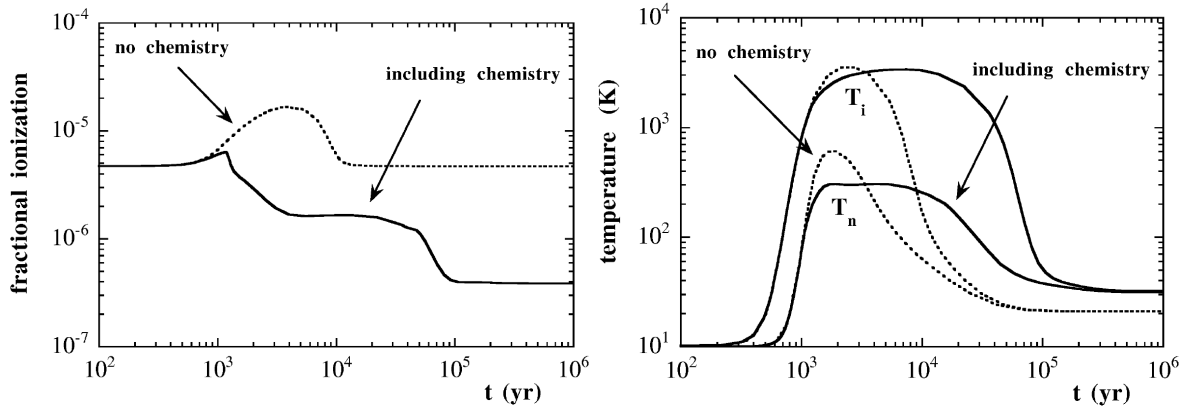
Figure 4.2: Impact of the chemistry on the fractional ionization ( left ) and temperature ( right ) of a C -shock. The shock velocity is 10 km s -1 . The preshock medium is molecular, at a density n_{\text{H}} = 10^3 \text{ cm}^{-3} . The preshock magnetic strength is B_0 = 25 \mu\text{G} , perpendicular to the direction of propagation of the shock. T_n and T_i are the temperatures of the neutral and ionized fluids, respectively. The plots show model results with ( solid line ) and without ( dotted line ) chemical reactions. Taken from Pineau des Forets et al. (1997).
