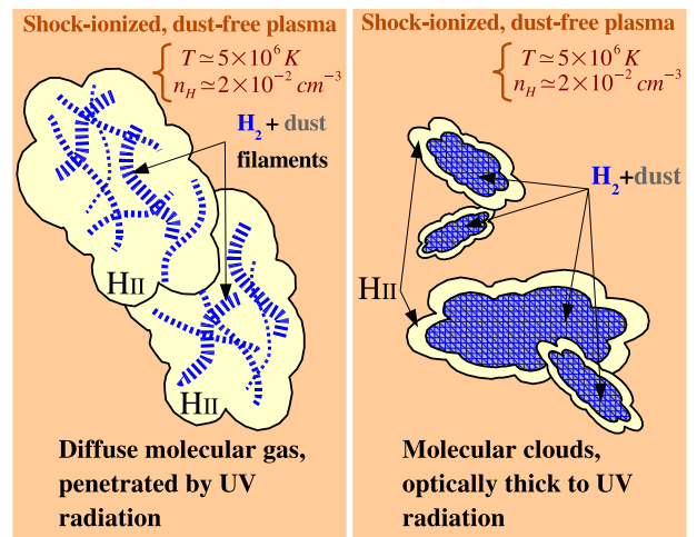
Fig. 6. Sketch of the two limiting physical states of the multi-phase molecular gas we are considering in the framework of our modeling of dust emission. (Left) Dust is associated with diffuse molecular gas that is broken into fragments, filaments or sheets, penetrated by UV radiation. (Right) The dusty molecular gas is in clouds that are optically thick to UV light.
