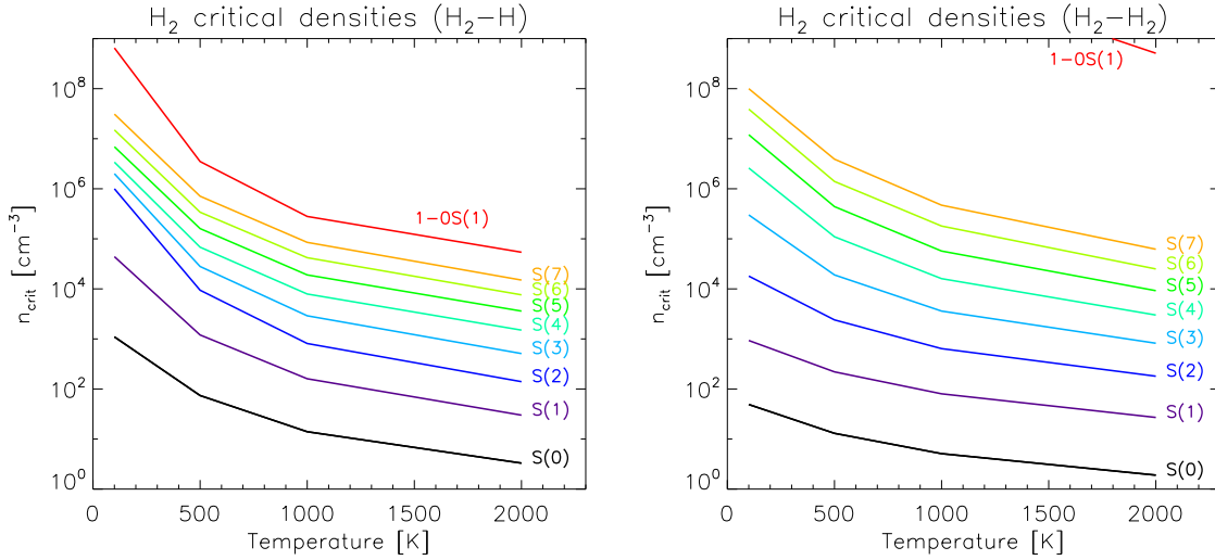
Figure 3.3: Critical densities, n_{\text{crit}} , for the S(0) to S(7) H 2 rotational lines, and the 1-0S(1) rovibrational line. The corresponding upper J levels are thermalized if the gas density is higher than n_{\text{crit}} . The collisional partner is H on the left plot and H 2 on the right . The critical densities are calculated at 100, 500, 1000 and 2000 K from Wrathmall et al. (2007).
