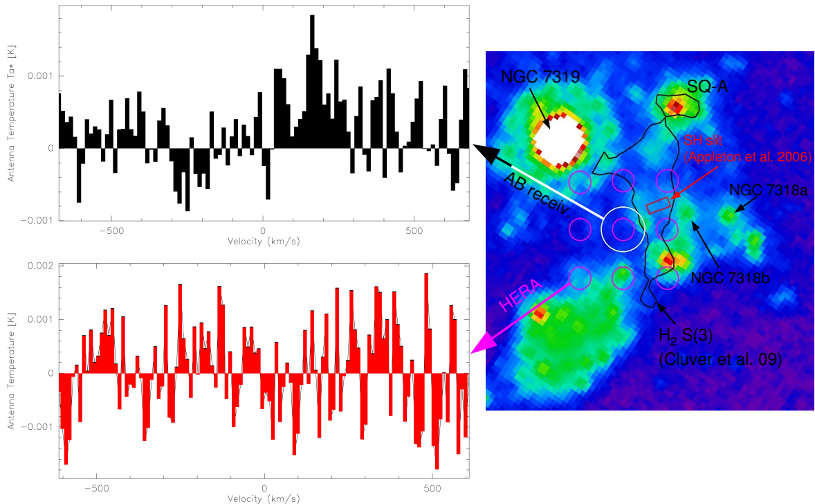
Figure 7.2: Pointing positions and averaged spectra of our two first runs of CO observations, overlaid on a Spitzer MIPS 24\ \mu\text{m} image. The small magenta circles show the CO(2-1) 11'' half-power beams of the HERA 3 \times 3 matrix. The white circle show the CO(1-0) 22'' HP beam of the AB receivers for our DDT program. The black contours is the 4\sigma ( 0.3\ \text{MJy sr}^{-1} ) \text{H}_2\ \text{S}(3) line emission from our paper II , which was not available at the time of these first CO observations. The central velocity is 6400\ \text{km s}^{-1} on the spectra. Weak lines at 6050 and 6130\ \text{km s}^{-1} are perhaps detected ( < 3\sigma ) on the CO(1-0) spectrum. On the HERA CO(2-1) spectrum no clear detection of CO gas is seen.
