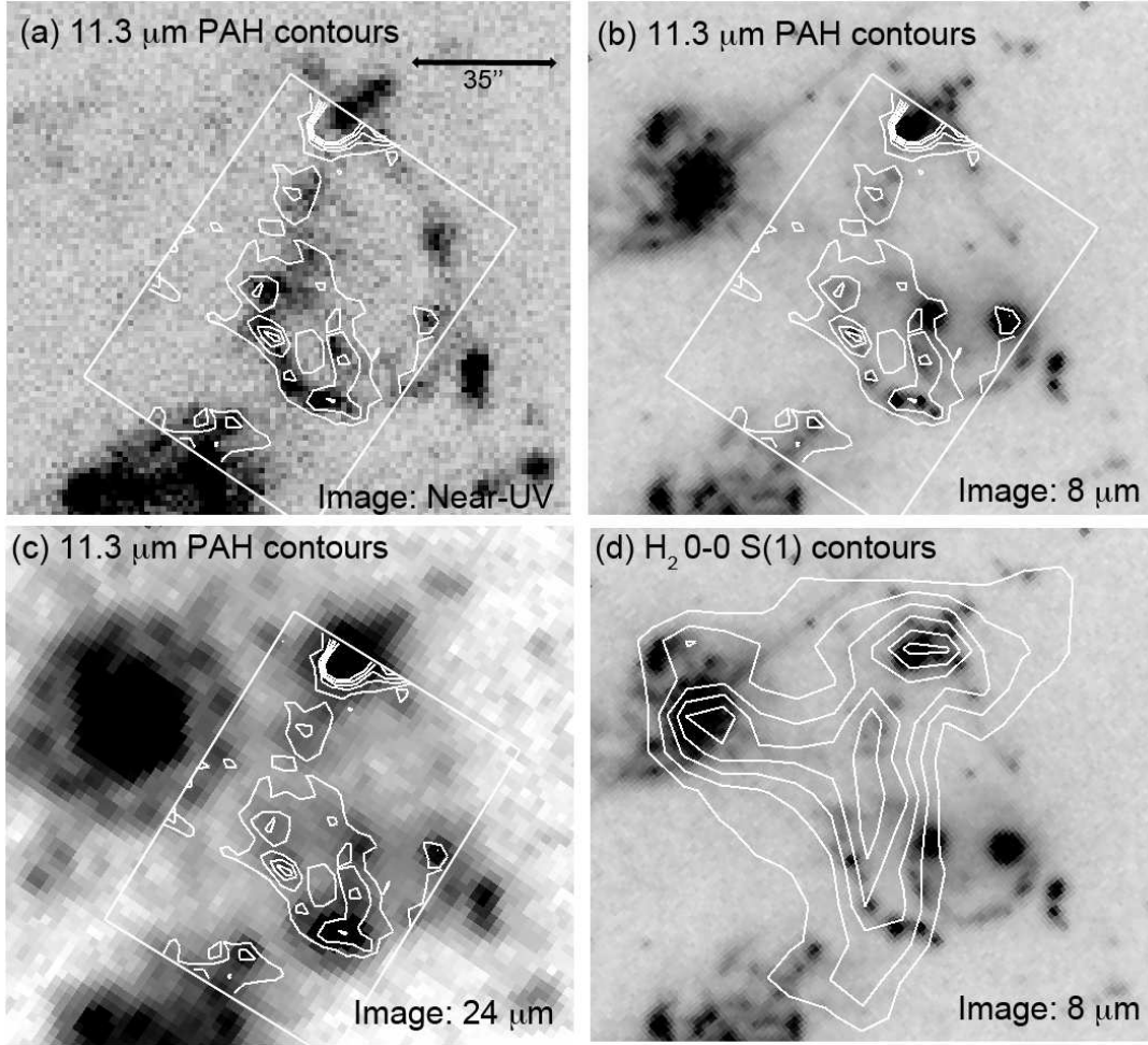
FIG. 6.— Dust as tracers of star formation. This shows 11.3 \mu m PAH contours overlaid on (a) the Near-UV, (b) an 8 \mu m image and (c) a 24 \mu m image. By comparison the H 2 0-0 S(1) contours show little correlation with the 8 \mu m image (as shown in d). Contour levels are as follows (in units of MJy/sr): (a), (b) and (c) are 0.2, 0.35, 0.5, 0.65, 0.8. Contour levels for (d) are as in Fig. 2b.
