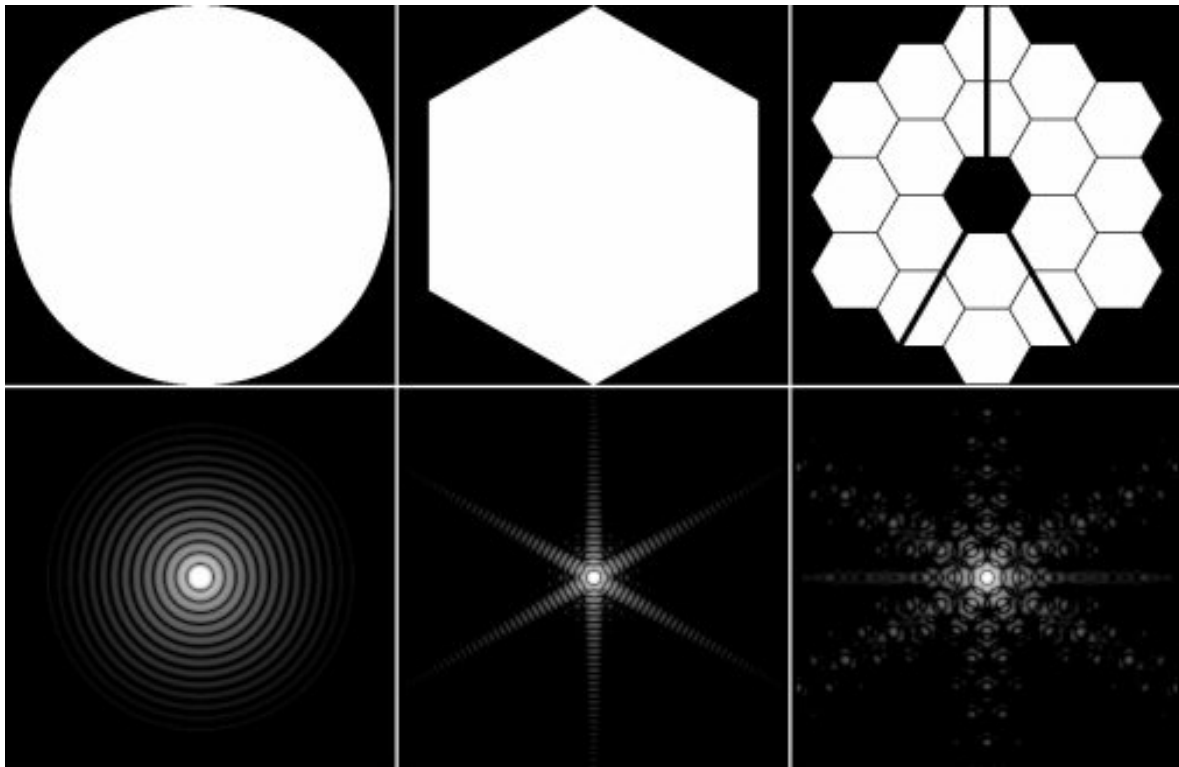
Figure 11.1: The PSF corresponding to each aperture is displayed on a logarithmic grayscale from 10^{-7} to 10^{-3} counts. The total number of counts in each of these simulated PSFs is 1. These PSF have been modeled with the JWPSF software a .
