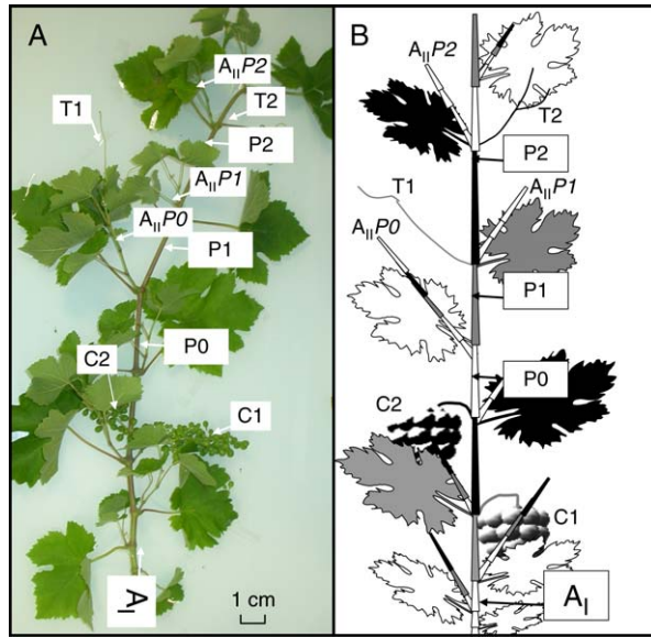
Fig. 2. (A) Photograph and (B) diagram of part of the structure of an annual shoot. A_i indicates the primary axis; P0, P1 and P2 indicate the type of phytomer on the primary axis and A_{ii}P_i , T_i and C_i indicate the secondary axes, tendrils and clusters, respectively, of the corresponding phytomer, P_i .
