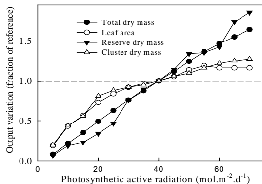
Figure 6. Sensitivity analysis of model outputs to different values of PAR. All model outputs were normalized according to the values observed at 40 \text{ mol.m}^{-2}.\text{d}^{-1} , 1200^\circ\text{Cd} after budburst with \text{FTSW}=1 .
