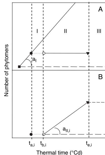
Fig. 3. Description of the variables used to analyze primary and secondary axis development as a function of thermal time. (A) Identification of the different phases of secondary axis development related to the development of the primary axis. (B) Representation of phytomer production by a secondary axis of insertion rank i on the primary axis. a_i : Leaf emergence rate on the primary axis; a_{ii,i} : leaf emergence rate on a secondary axis of rank i ; I: first phase of development of the secondary axes (lag period) between t_{a,i} (thermal time of appearance of the phytomer of rank i on the primary axis) and t_{b,i} (date of budburst for the secondary axis of rank i ); II: second phase of development of the secondary axes between t_{b,i} and t_{e,i} (thermal time at which the apex of the secondary axis of rank i stops developing) and III: third phase of development of the secondary axes, after t_{e,i} , when no new phytomers are produced.
