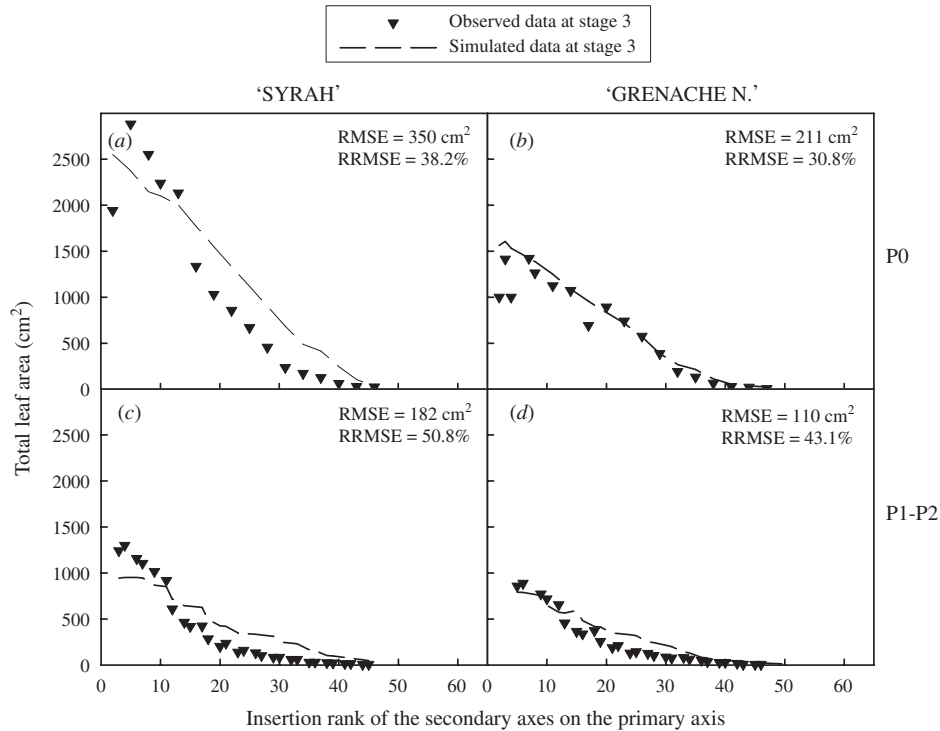
Fig. 5. Observed (symbols) and GreenLab-simulated (lines) values for total leaf areas of P0 (a, b) and P1-P2 (c, d) secondary axes as a function of insertion rank of the secondary axis, at stage 3 (stage 38 (Coombe 1995)) for 6C treatments of grapevine cultivars 'Syrah' (a, c) and 'Grenache N.' (b, d). P0 and P1-P2 secondary axes are the secondary axes arising from P0 and P1-P2 phytomers, respectively, on the primary axis.
