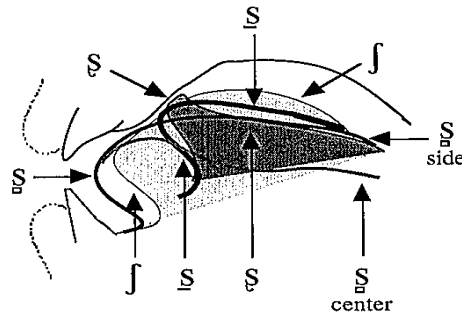
Figure 5.17 A composite diagram of Toda tongue positions in sibilant fricatives. In the case of ʃ the center and sides of the tongue have been shown separately. The position of the center and sides is taken to be much the same for the other sounds, and only one tongue line is shown for each of them.
