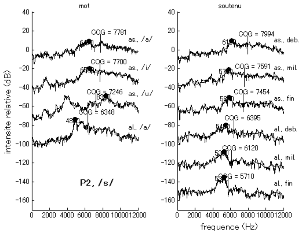
Figure 190. Spectres moyens, /s/, polonais.
