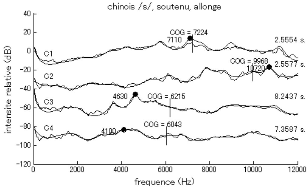
Figure 187. Spectres moyens, /s/, chinois.
