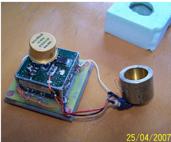
FIGURE C.11: L'oscillateur OP22-M fini.
