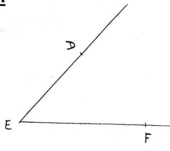
angle DEF
