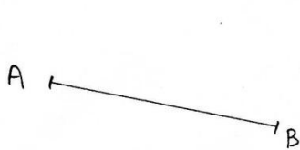
segment [AB]
