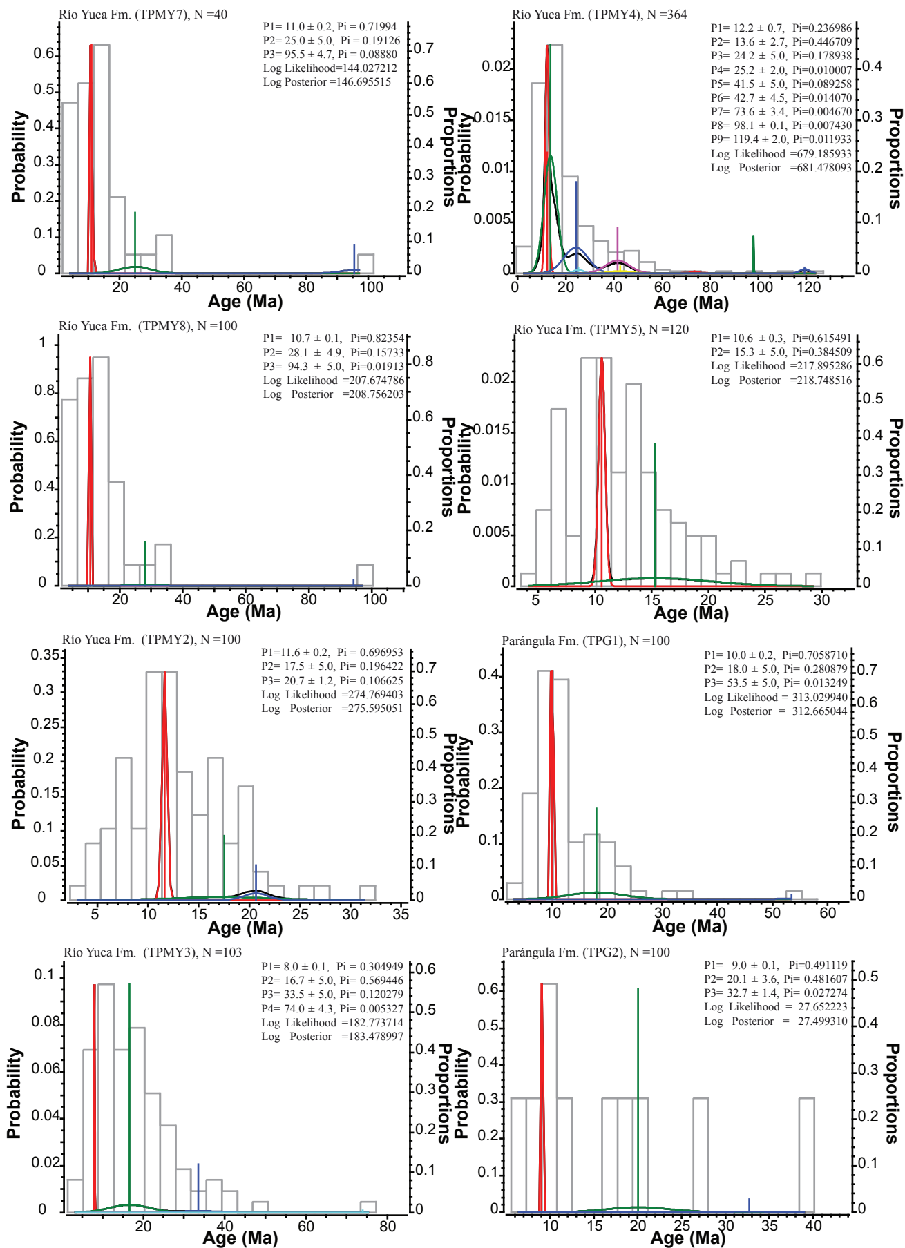
Figure A5 (cont.). Decomposition into significant ages populations using BayesQt for syngenetic fission-track samples (see Table A2).
