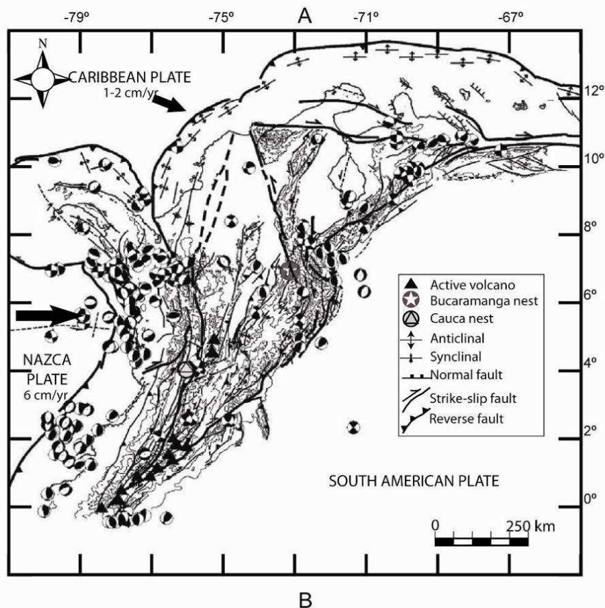
Fig. 2.10. A) Major tectonic features of northern South America and Global Positioning System (GPS) velocity vectors from different studies. All vectors denote velocities with respect to South America, and shading denotes different studies (After Colmenares and Zoback, 2003). B) Focal mechanisms of shallow earthquakes (<60 km) in the northern Andes. Usual representation as “beachballs” (Schmid projection lower hemisphere); with P-extensional quadrangles white and T-compressive black (After Cortés and Angelier, 2005).
