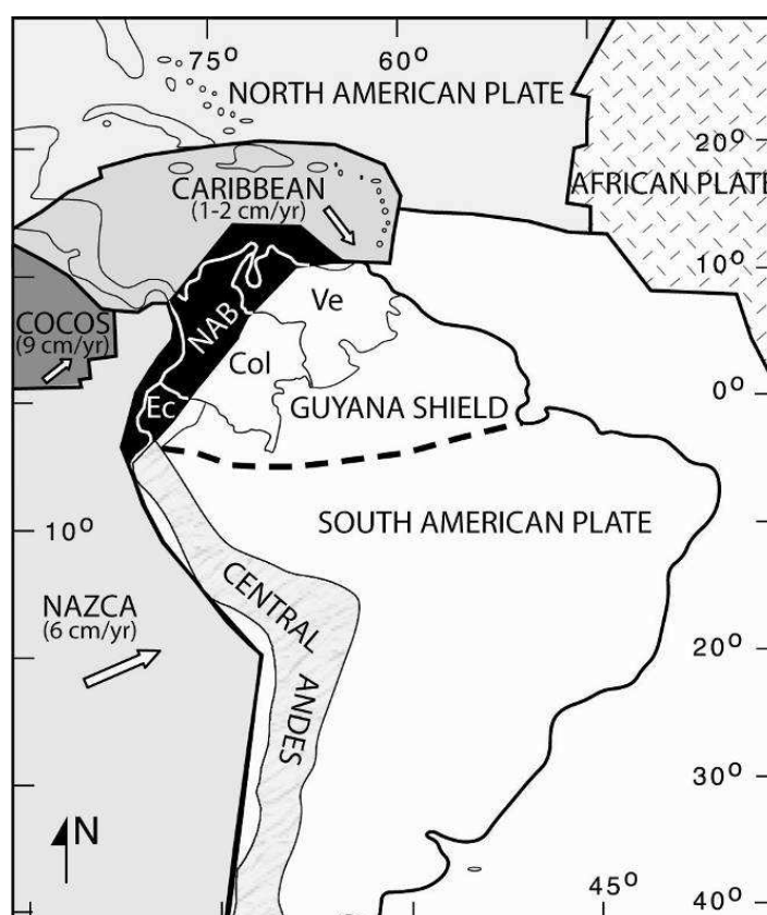
Fig. 2.1. Tectonic framework of north-western South America. NAB = Northern Andean Block; Ec, Col, Ve = geographic limits of Ecuador, Colombia and Venezuela, respectively (modified from Cediel et al. 2003).
