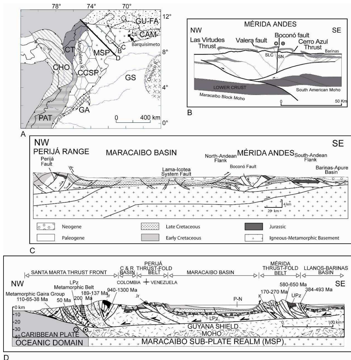
Fig. 4.2. A) Subdivision of northern Andes into tectonics domains: CAM: Caribbean Mountain terrane; CCSP: Central Continental Sub-Plate (Eastern Cordillera, Cordillera Real, San Lucas block, Ibaguë block); CHO: Chocó Arc; CT: Caribbean Terranes; GA: Garzón Massif; GS: Guyana Shield; GU-FA: Guajira-Falcón Composite Terrane; MSP: Maracaibo Sub-Plate; PAT: Pacific assemblages (after Cediel et al. 2003). B-D: Different tectonic models presented as NW-SE structural cross sections: B) across the Mérida Andes (Colletta et al. 1997; SLC: Sierra la Culata block; SN: Sierra Nevada block); C) Through the Maracaibo Basin from the Mérida Andes to the Perijá Range (Yoris and Ostos, 1997); D) Along the Maracaibo subplate (after Cediel et al. 2003). Abbreviations: C&R basin: César and Ranchería basin; LPz: lower Paleozoic; UPz: upper Paleozoic; Jr: Jurassic; K: Cretaceous; P: Paleogene; N: Neogene.
