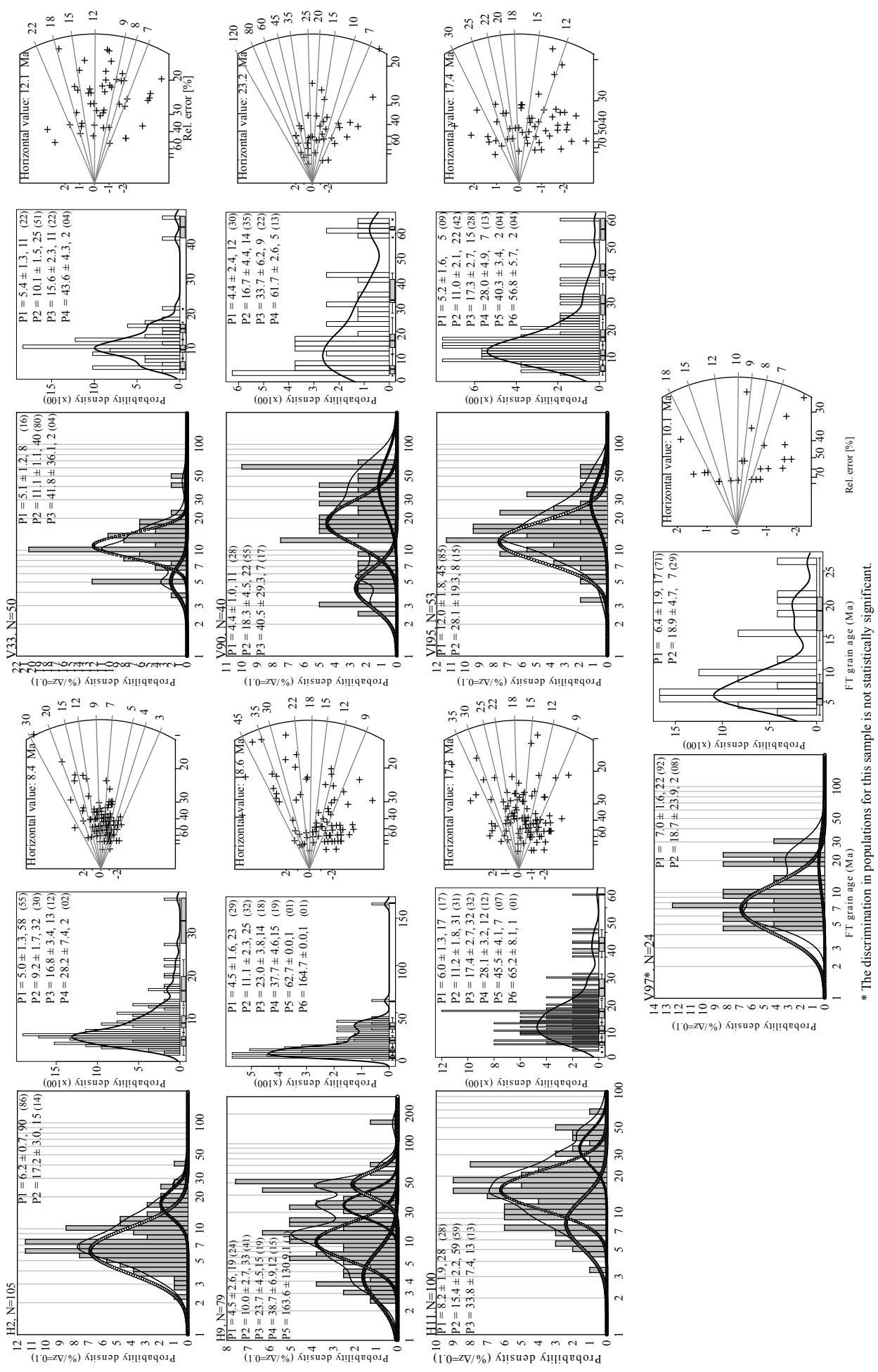
Figure A4. Decomposition into significant ages populations using Binomfit and p-partition. Radial plots of synorogenic fission-track samples (see Table A2).
