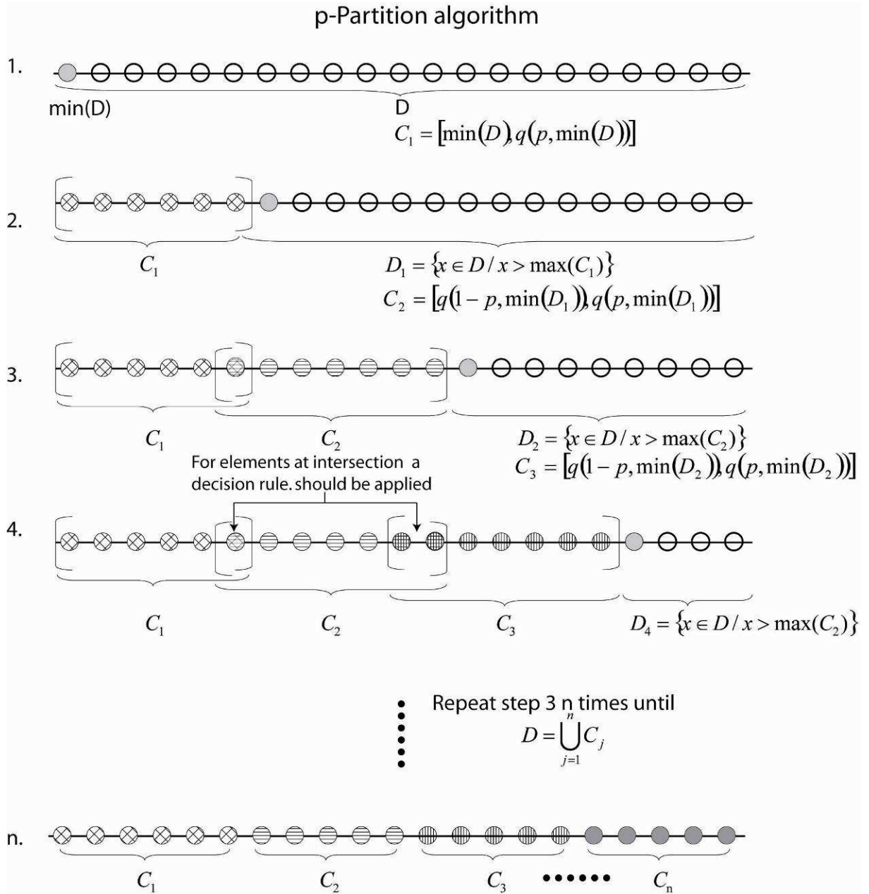
Figure 1. Flowchart showing the implementation of the p-partition algorithm.
