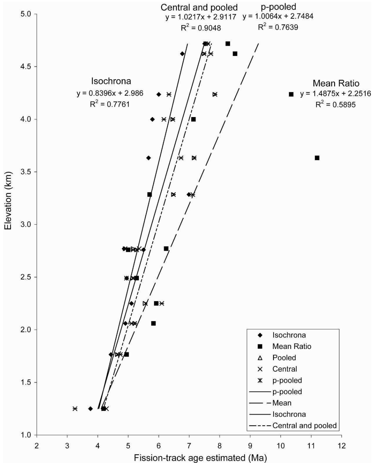
Figure 3. Comparison of age-elevations relationships given by the different fission-track age estimations
