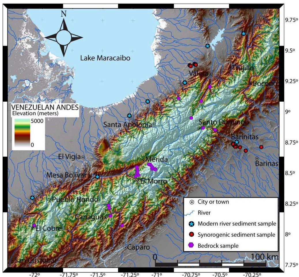
Fig. 1.3. Digital elevation model of the Venezuelan Andes with the samples location for AFT thermochronology collected in this work.
