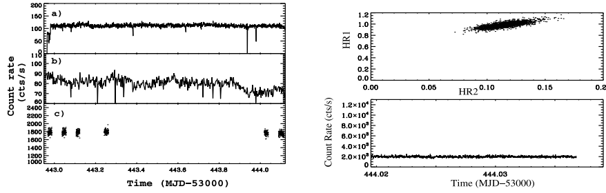
FIG. 9.—Left: Light curves of GRS 1915+105 during Obs. 3: (a) JEM-X 3–13 keV binned at 50 s; (b) ISGRI 18–50 keV binned at 200 s; (c) RXTE PCA 2–18 keV binned at 16 s. Right: CC diagram (top) and RXTE light curve (bottom) of a subinterval from Obs. 3 showing the source was in class \chi .
