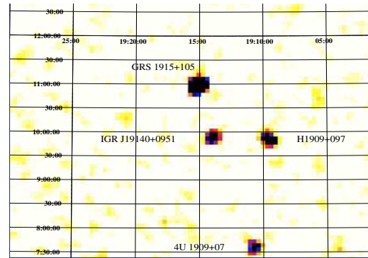
Fig. 1. The IBIS/ISGRI 20–30 keV image, showing the new source and three other sources in the field-of-view. GRS 1915+105 is bright in this energy range. The image is \sim 7^\circ width and \sim 5^\circ.3 height. North is up and East is to the left. The other sources in the field are dealt with in Molkov et al. (2004).
