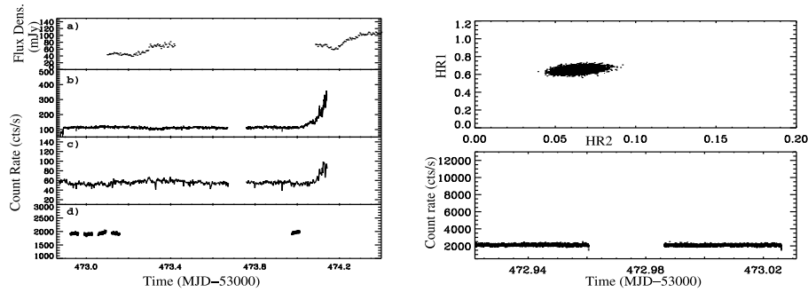
FIG. 5.—Left: Light curves of GRS 1915+105 during Obs. 4: (a) RT at 15 GHz; (b) JEM-X 3–13 keV binned at 50 s; (c) ISGRI 18–50 keV binned at 200 s; (d) RXTE PCA 2–18 keV binned at 16 s. Right: CC diagram (top) and RXTE light curve (bottom) of one subinterval from Obs. 4 showing the source was in class \chi .
