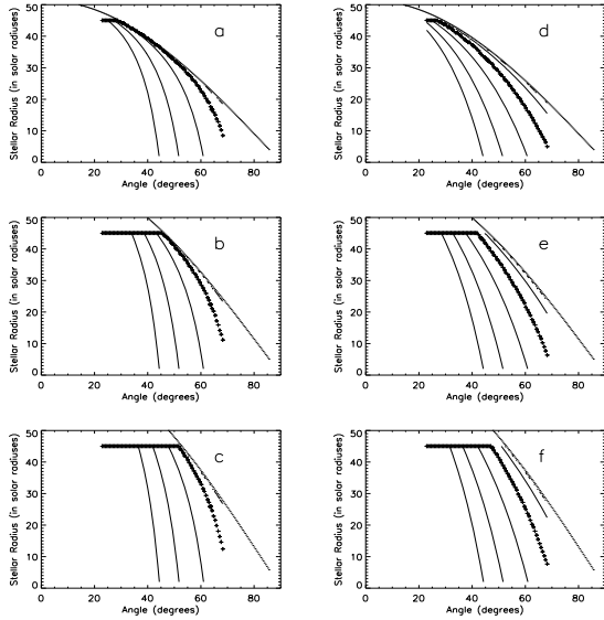
Figure 5. Most probable orbital inclination, as a function of the companion radius, for various \dot{M}_* and \beta . (a) \beta = 0.5 , \dot{M}_* = 10 M_\odot . (b) \beta = 0.5 , \dot{M}_* = 20 M_\odot . (c) \beta = 0.5 , \dot{M}_* = 30 M_\odot . (d) \beta = 1 , \dot{M}_* = 10 M_\odot . (e) \beta = 1 , \dot{M}_* = 20 M_\odot . (f) \beta = 1 , \dot{M}_* = 30 M_\odot . The ‘+’ symbols correspond to the most probable orbital inclination, confidence contours are drawn at the 25, 68 and 90 per cent confidence levels. The dotted line is the ‘eclipse limit’: points above this line are excluded as it would imply an eclipse of the neutron star by its companion, which is not observed.
