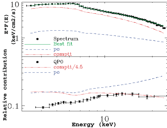
FIG. 8.— Top : RXTE PCA spectrum of Obs. 4 Int. I (filled circle). The best-fit model, the power-law component, and the comptt component are overlotted. Bottom : Relative contribution of the comptt component and spectrum of the QPO.
