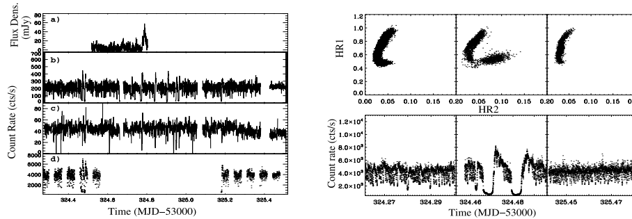
FIG. 3.—Left: Same as Fig. 2 for Obs. 2. Right: CC diagrams (top) and RXTE light curves (bottom) of three subintervals from Obs. 2, showing occurrences of class \mu/\nu (left), class \lambda (middle), and class \gamma (right).
