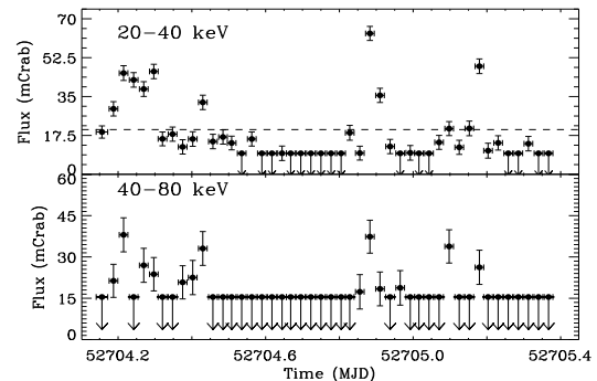
Fig. 2. The 20–40 keV ( top ) and 40–80 keV ( bottom ) ISGRI lightcurves. Each symbol represents a science window. The 3-sigma upper limits are denoted with an arrow. The dashed line in the upper panel indicates the 20 mCrab level.
