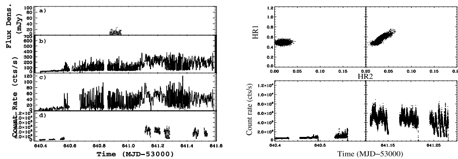
FIG. 10.—Left: Light curves of GRS 1915+105 during Obs. 7: (a) RT at 15 GHz; (b) JEM-X 3–13 keV binned at 20 s; (c) ISGRI 18–50 keV, binned at 100 s. Right: CC diagrams (top) and RXTE light curves (bottom) of two subinterval from Obs. 7 showing the source was in class \phi at the beginning and class \delta in the end. Note that between those two classes GRS 1915+105 transited through a class \theta .
