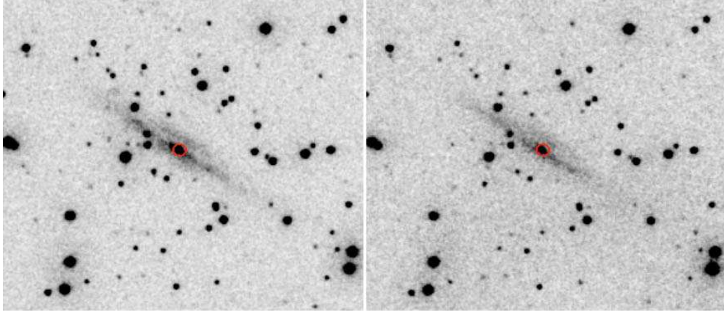
Fig. 3. 4.3'×4.1' U (left) and UVW1 (right) UVOT images of the field around IGR J09025–6814. The best X-ray position is represented by the circle.
