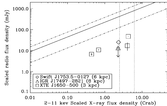
FIG. 4.—Plot of the radio vs. X-ray fluxes for the BH XTE J1650–500 (Corbel et al. 2004), the BHC SWIFT J1753.5–0127 (Cadolle Bel et al. 2006b), and IGR J17497–2821 with their (assumed) distances. All fluxes are normalized to a distance of 1 kpc. The range of correlated radio/X-ray fluxes is indicated by the dash-dotted lines, while the solid line indicates the best position. The vertical dotted lines indicate 2% and 5% of the Eddington luminosity.
