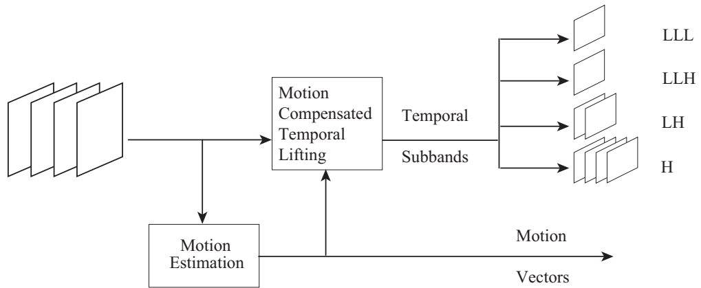
Figure 3.2: General scheme of the motion-compensated temporal analysis.
