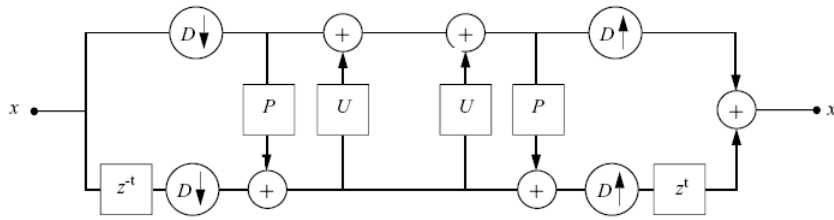
Figure 3.20: General filter bank.
