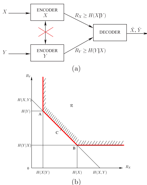
Figure 7.1: Distributed coding of statistically dependent i.i.d. discrete random sequences X and Y . Set-up (a); Achievable rate region (b).
